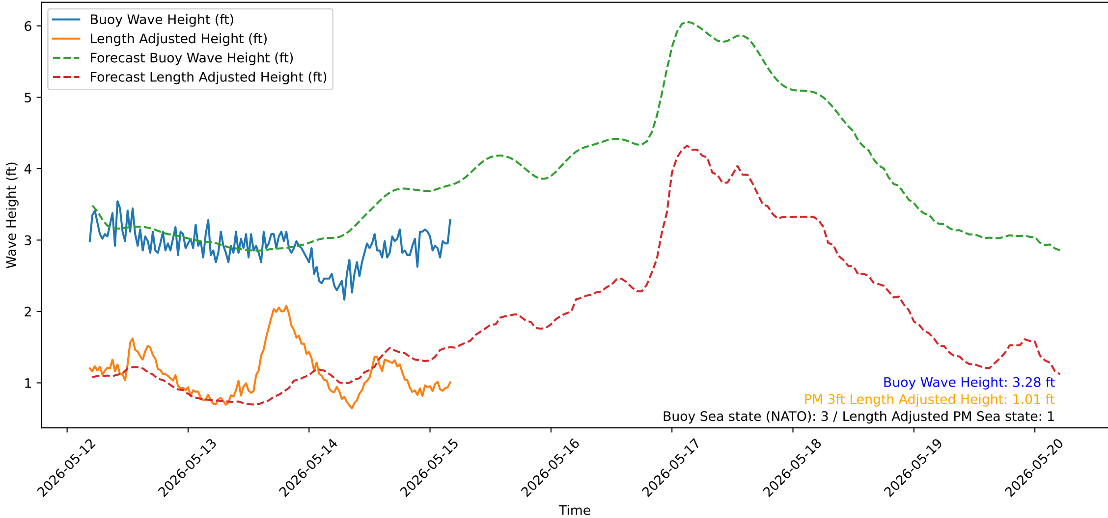
Wave Heights over Time for Oceanside Harbor at 2026-05-15 04:40:32
