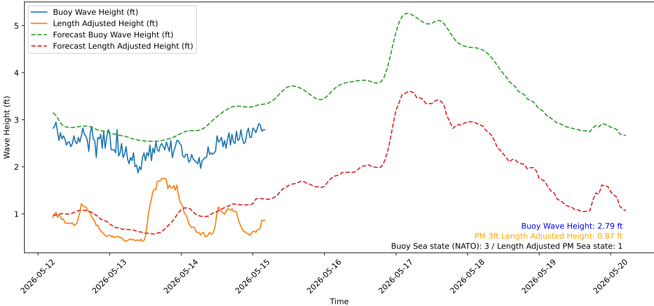
Wave Heights over Time for Red Beach at 2026-05-15 04:40:52
