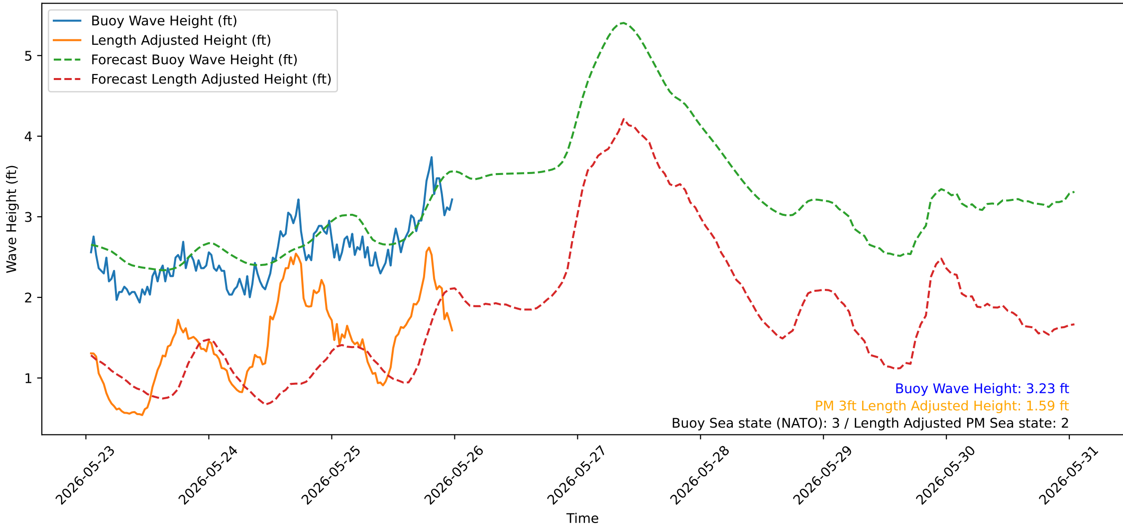
Wave Heights over Time for Red Beach at 2026-05-26 00:30:49
