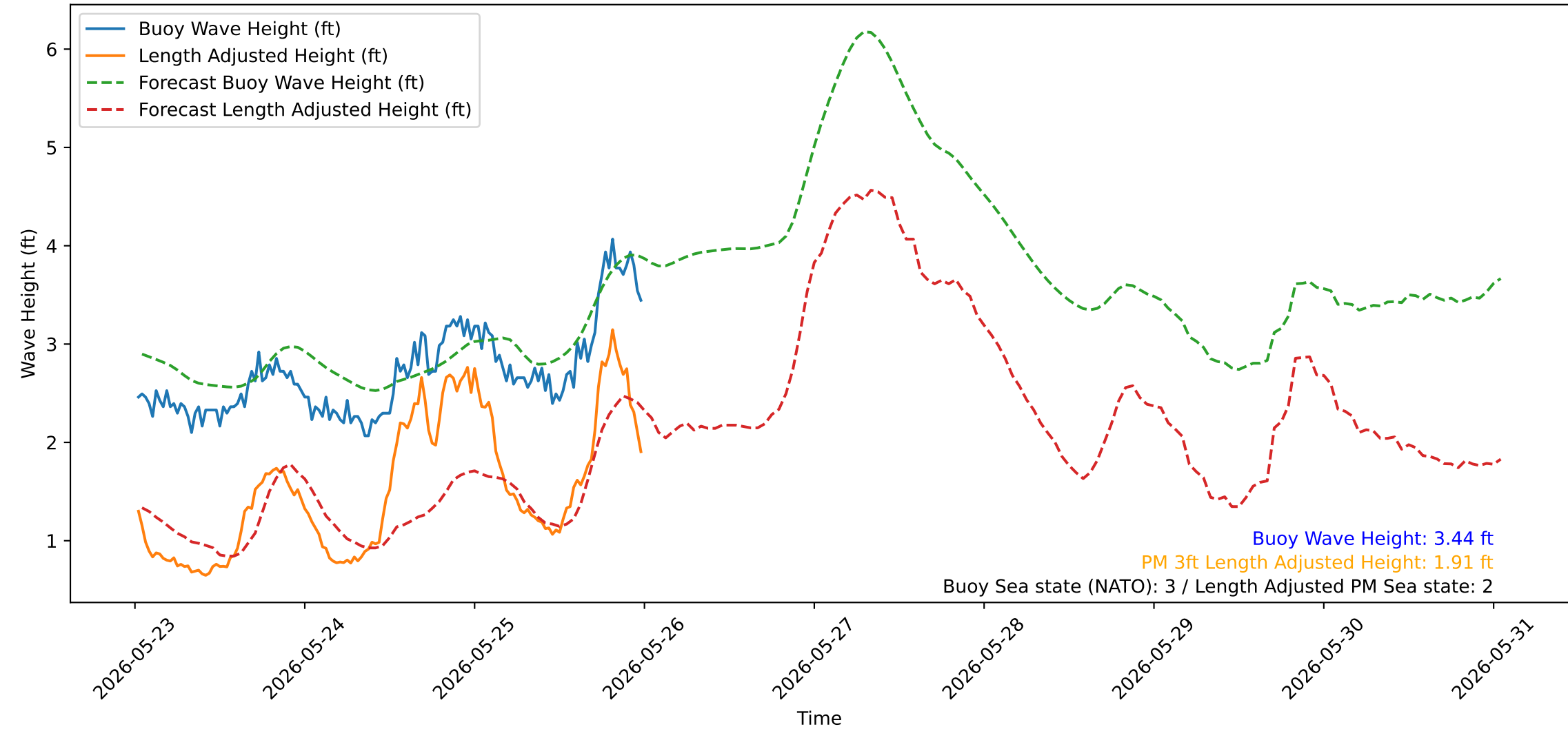
Wave Heights over Time for Green Beach at 2026-05-26 00:31:12
