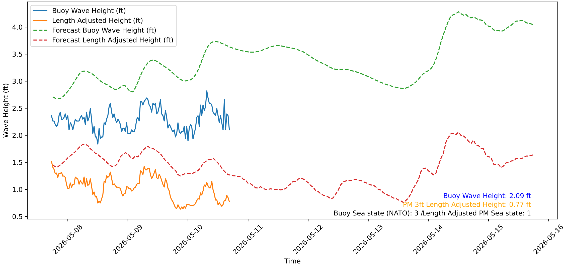
Wave Heights over Time for Green Beach at 2026-05-10 17:31:13
