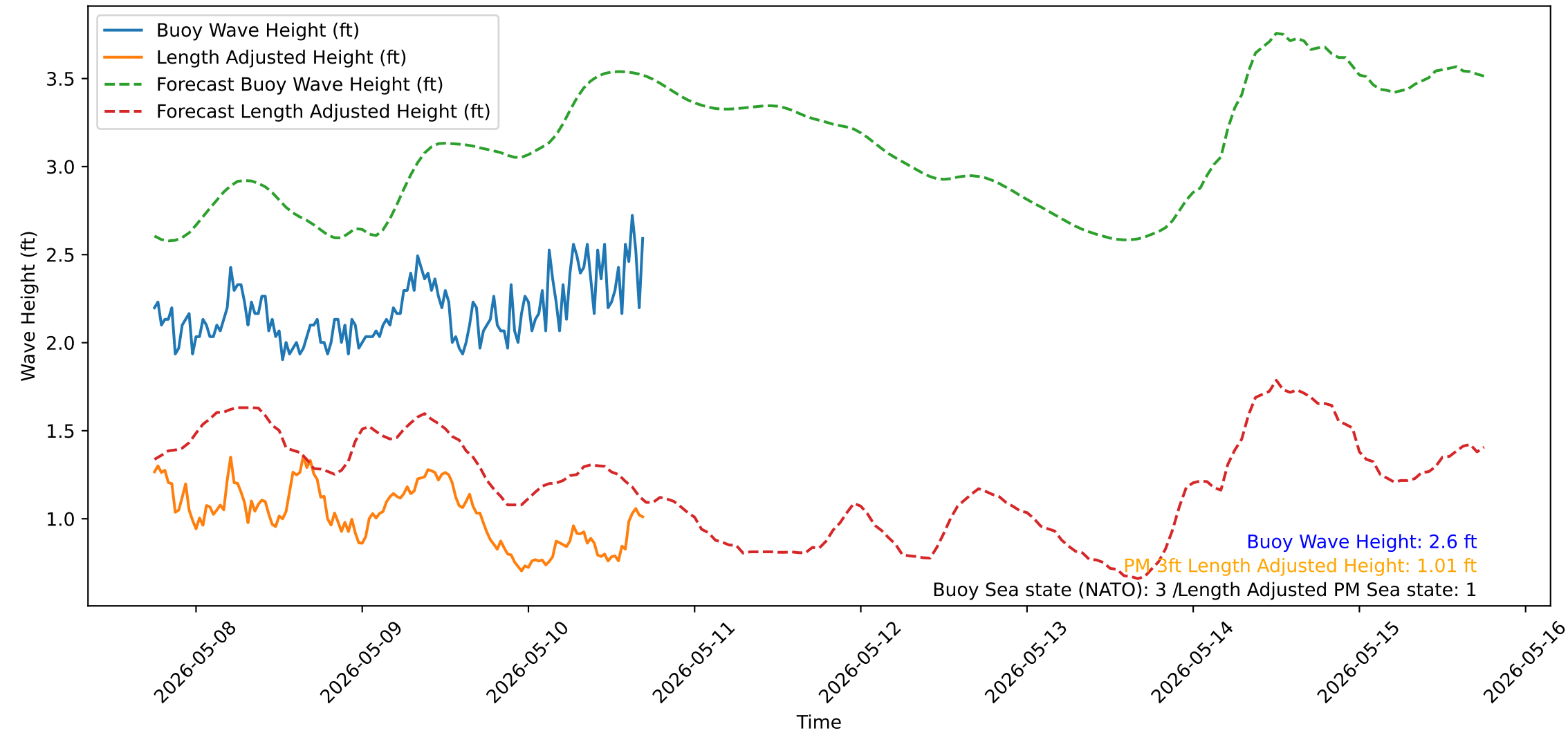
Wave Heights over Time for Red Beach at 2026-05-10 17:30:51
