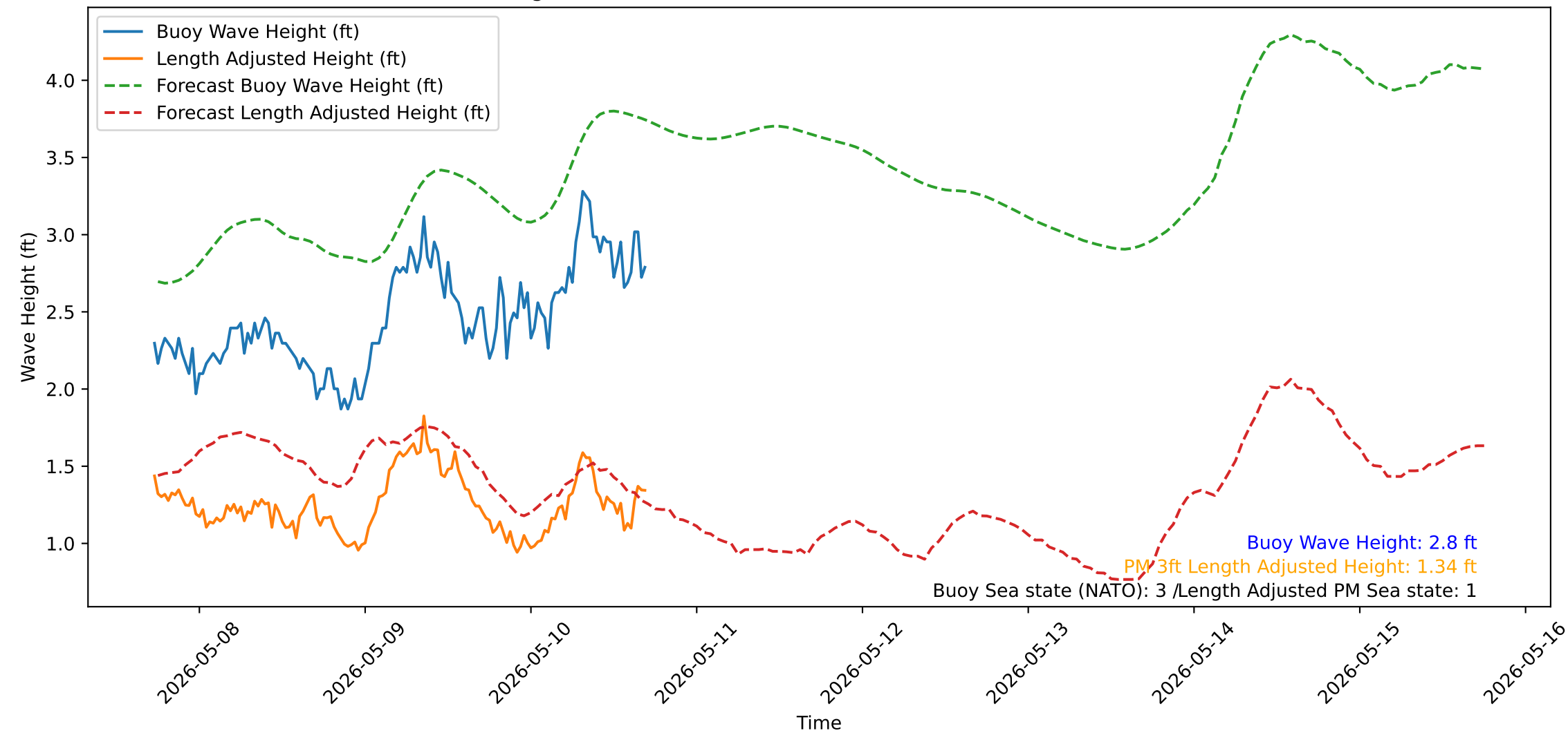
Wave Heights over Time for Oceanside Harbor at 2026-05-10 17:30:31
