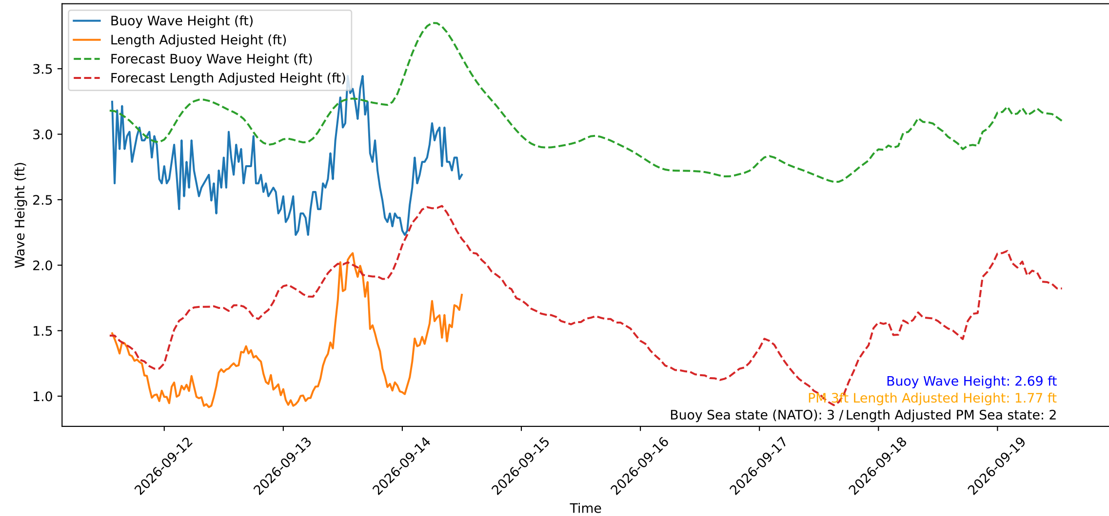
Wave Heights over Time for Red Beach at 2026-09-14 13:00:49
