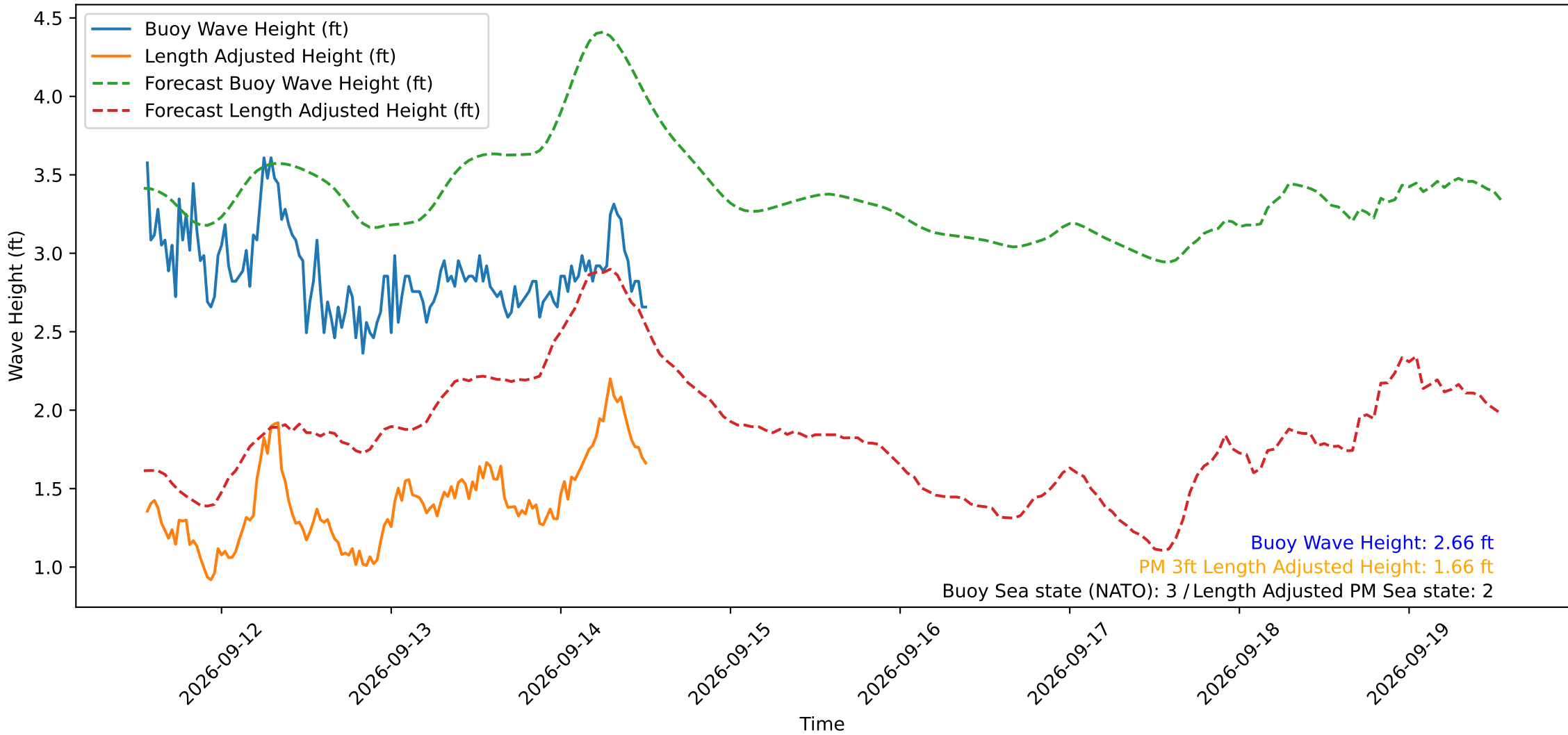
Wave Heights over Time for Green Beach at 2026-09-14 13:01:12
