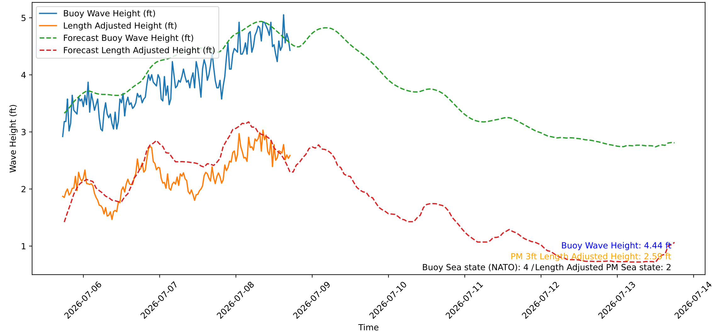
Wave Heights over Time for Oceanside Harbor at 2026-07-08 17:40:26
