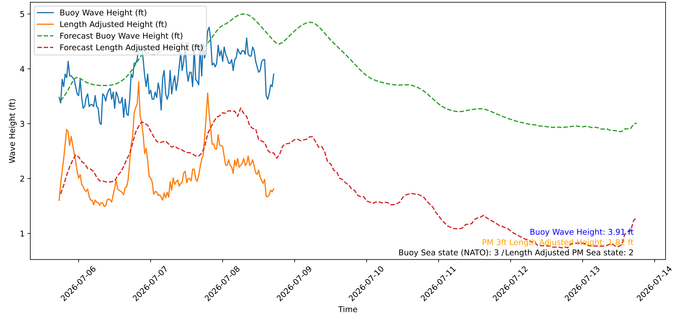
Wave Heights over Time for Green Beach at 2026-07-08 17:41:08
