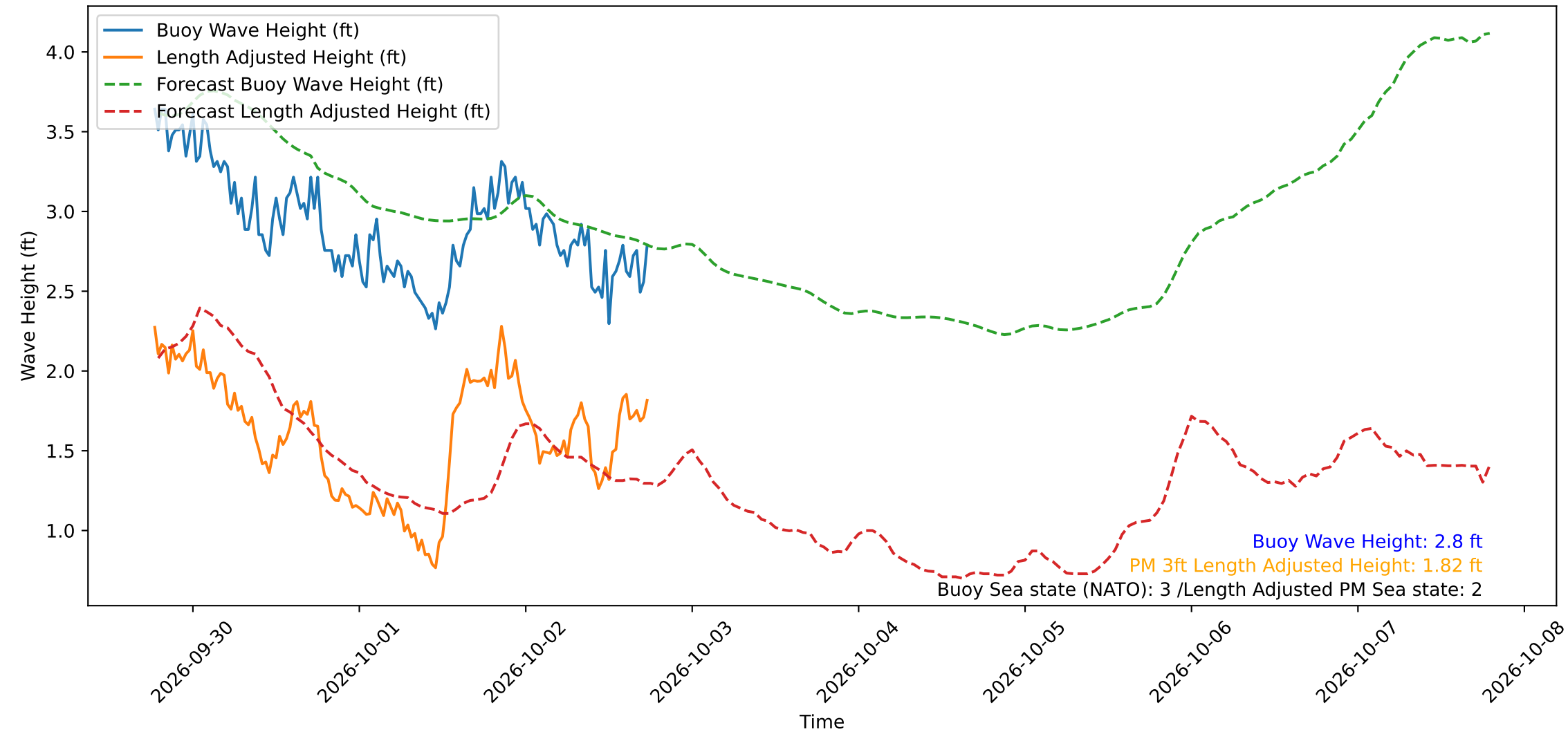
Wave Heights over Time for Oceanside Harbor at 2026-10-02 18:30:29
