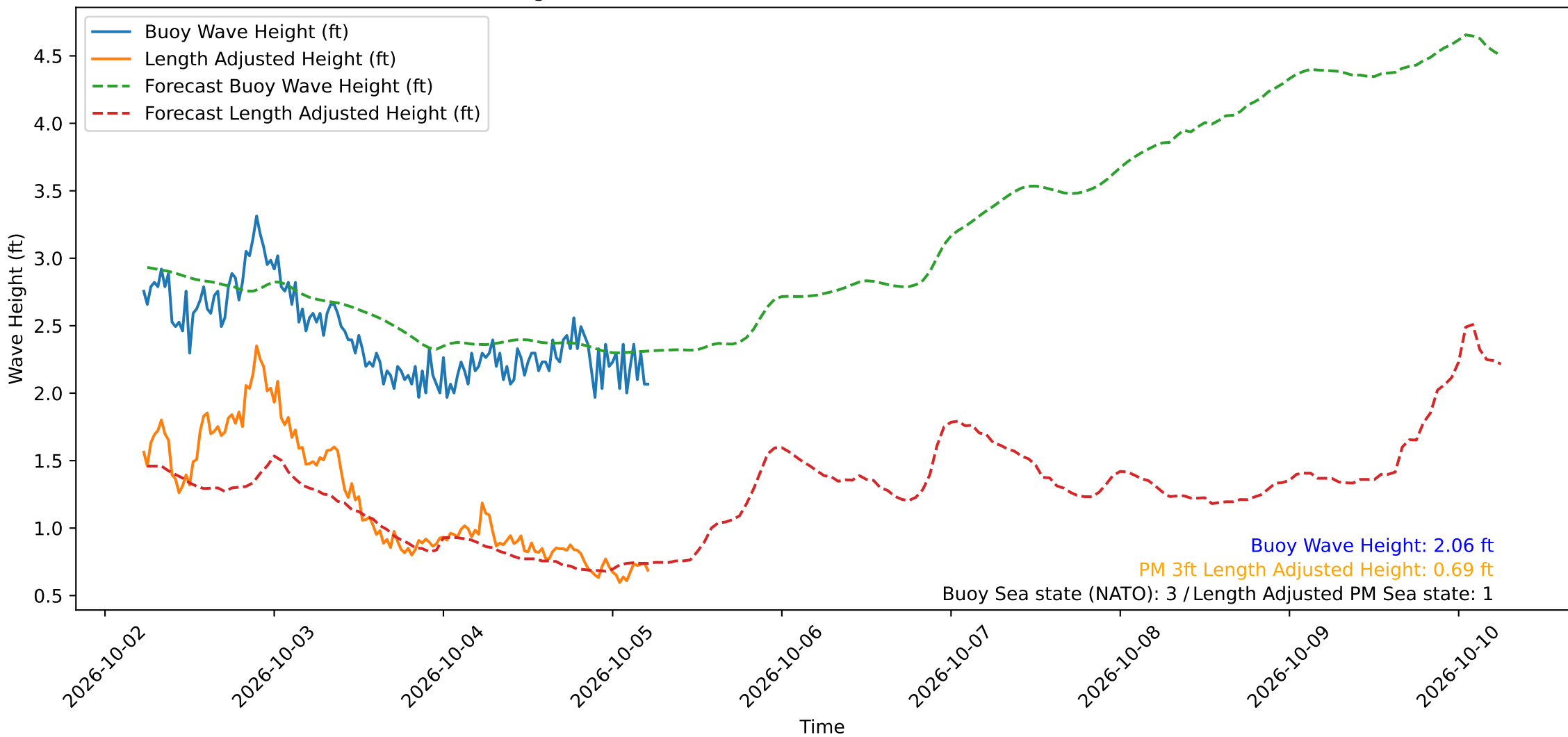
Wave Heights over Time for Oceanside Harbor at 2026-10-05 05:40:29
