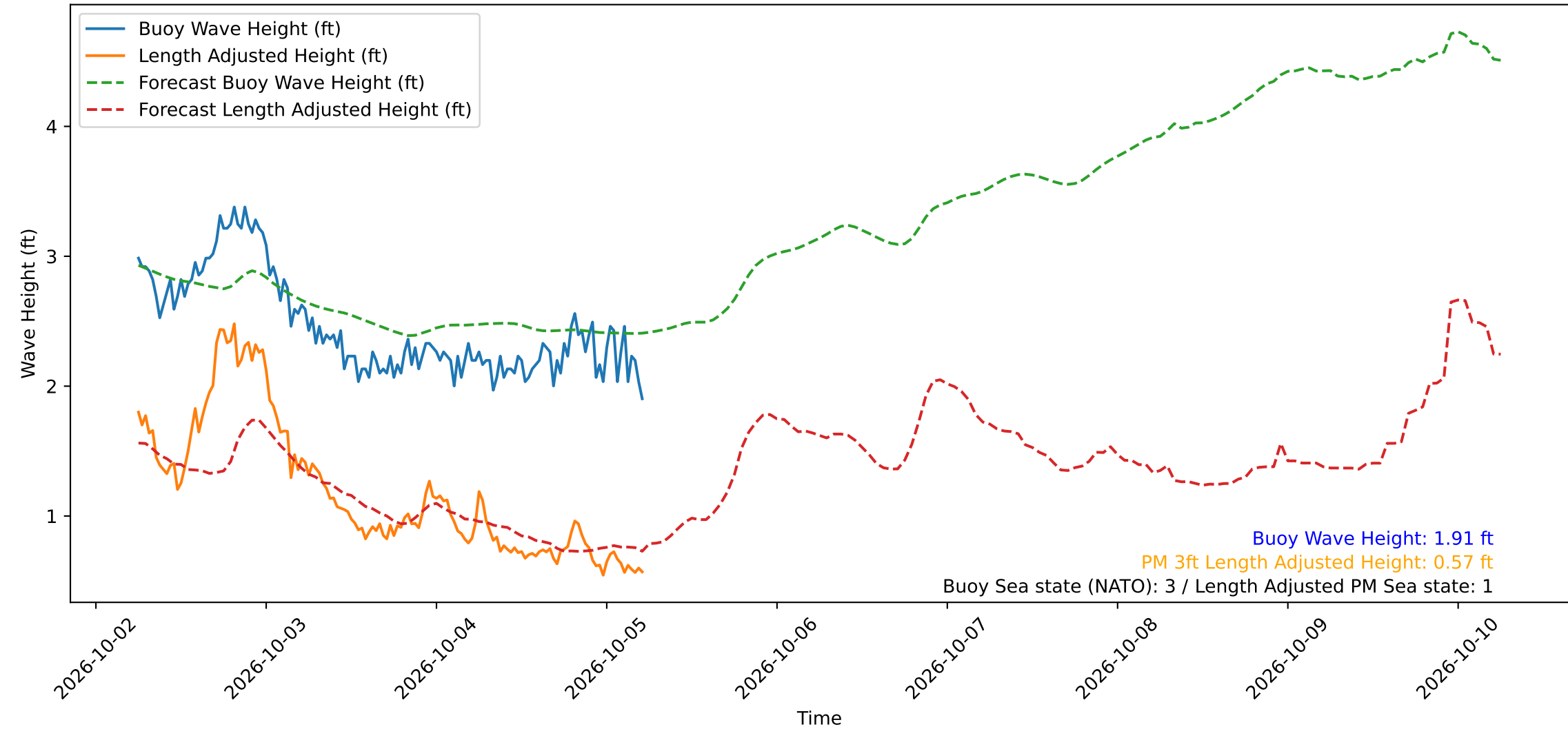
Wave Heights over Time for Green Beach at 2026-10-05 05:41:11
