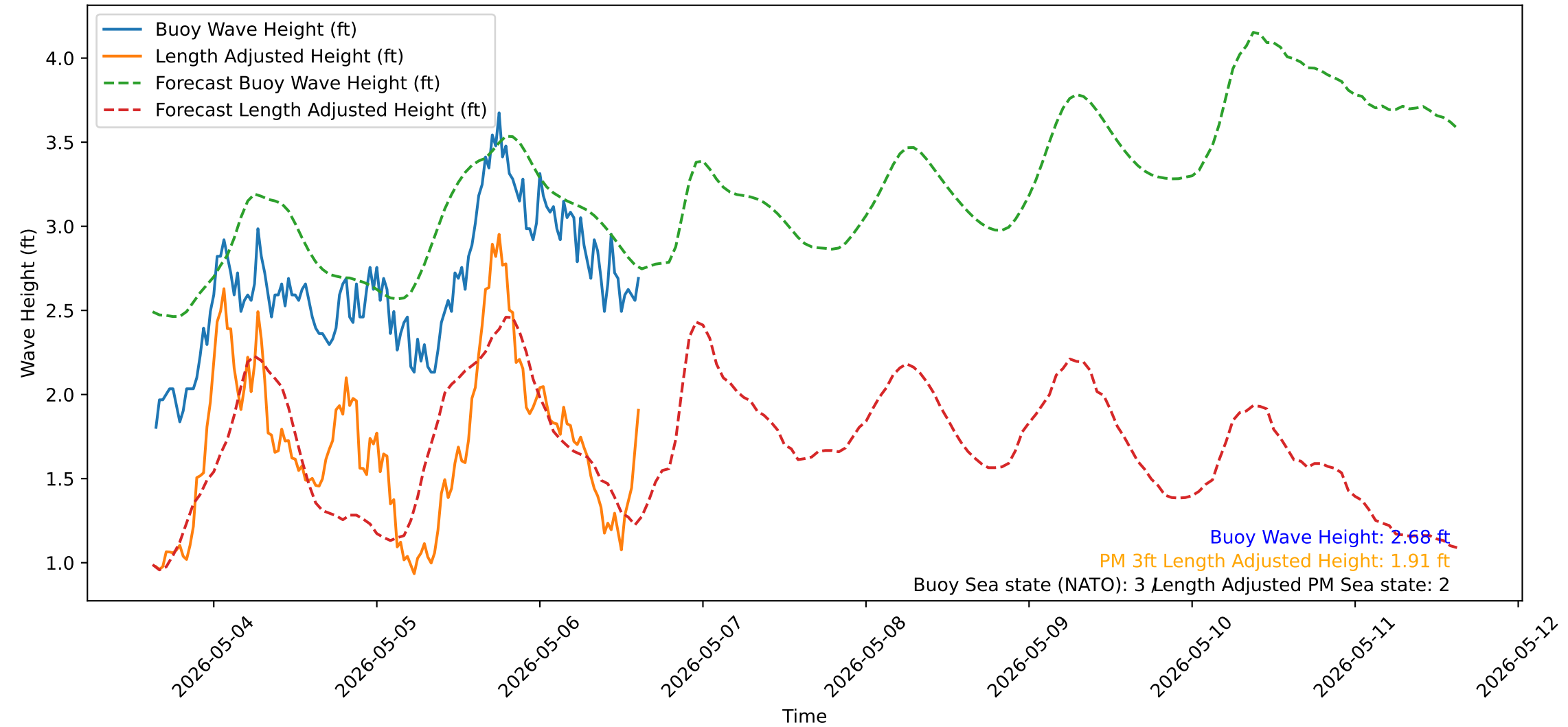
Wave Heights over Time for Green Beach at 2026-05-06 15:21:14
