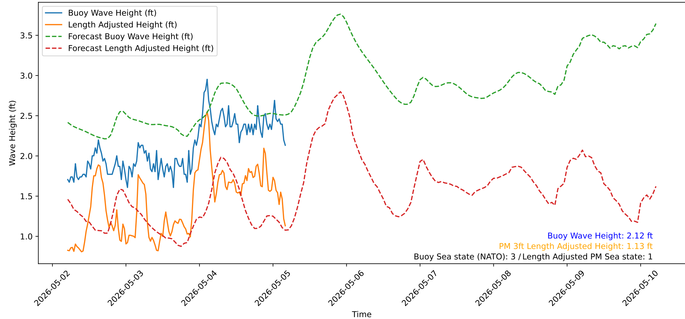
Wave Heights over Time for Red Beach at 2026-05-05 04:50:53
