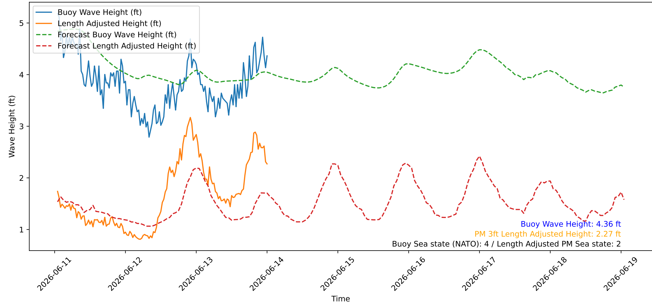
Wave Heights over Time for Oceanside Harbor at 2026-06-14 00:50:26
