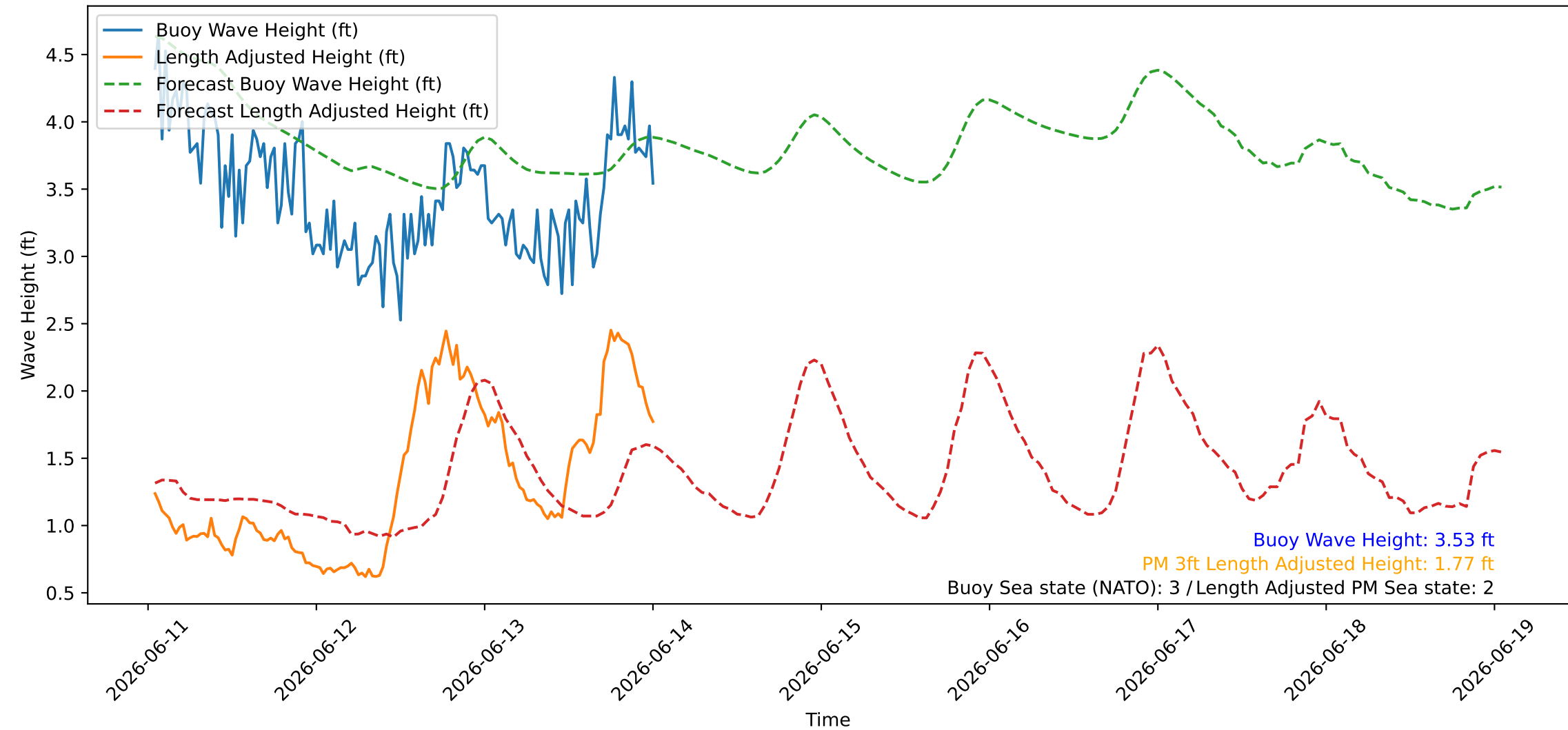
Wave Heights over Time for Red Beach at 2026-06-14 00:50:47
