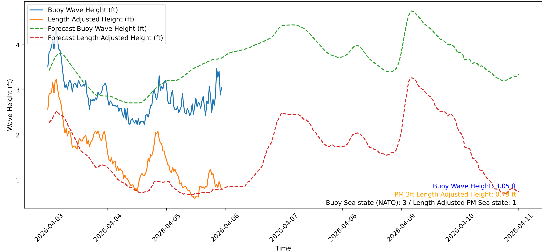
Wave Heights over Time for Green Beach at 2026-04-05 23:31:09
