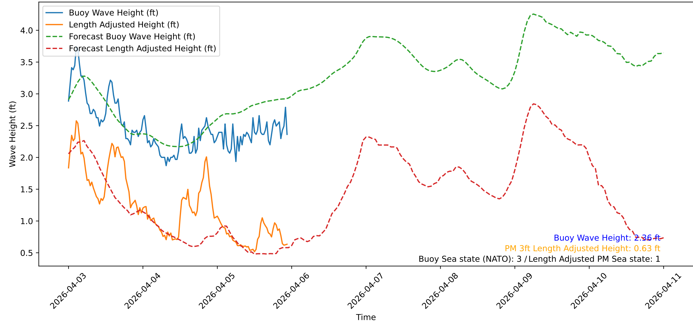
Wave Heights over Time for Red Beach at 2026-04-05 23:30:47
