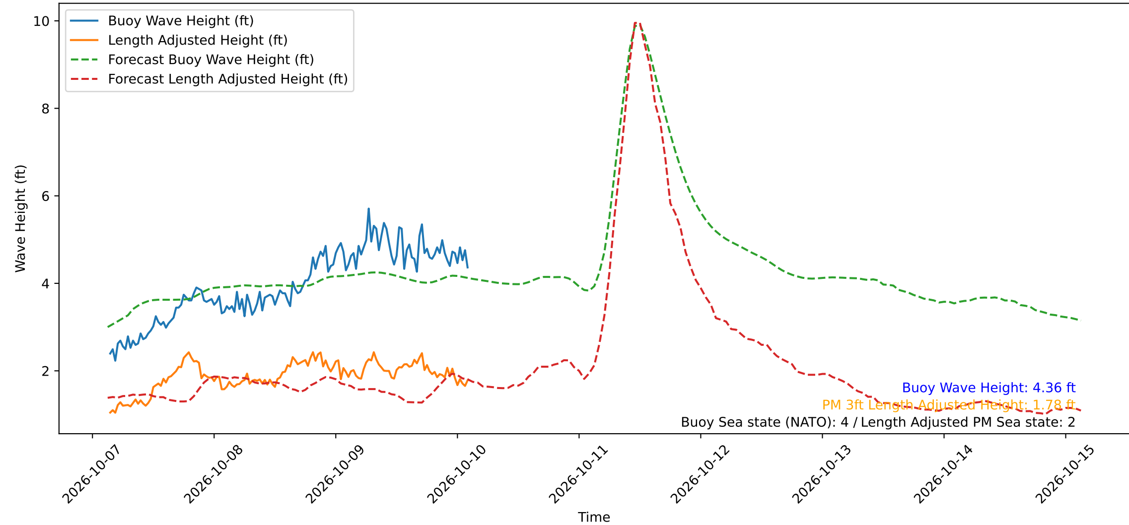
Wave Heights over Time for Red Beach at 2026-10-10 03:00:49
