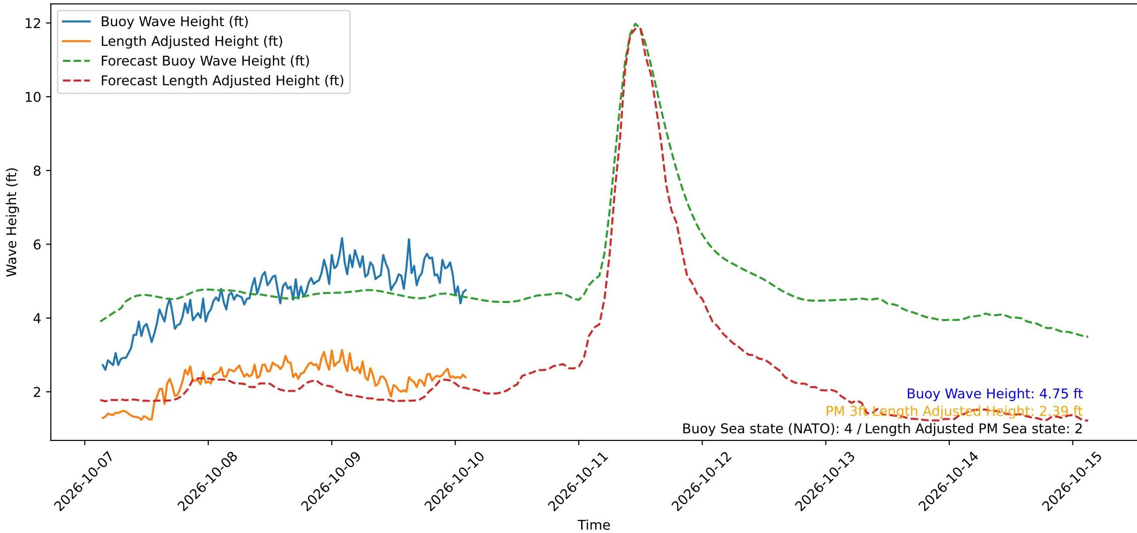
Wave Heights over Time for Green Beach at 2026-10-10 03:01:12
