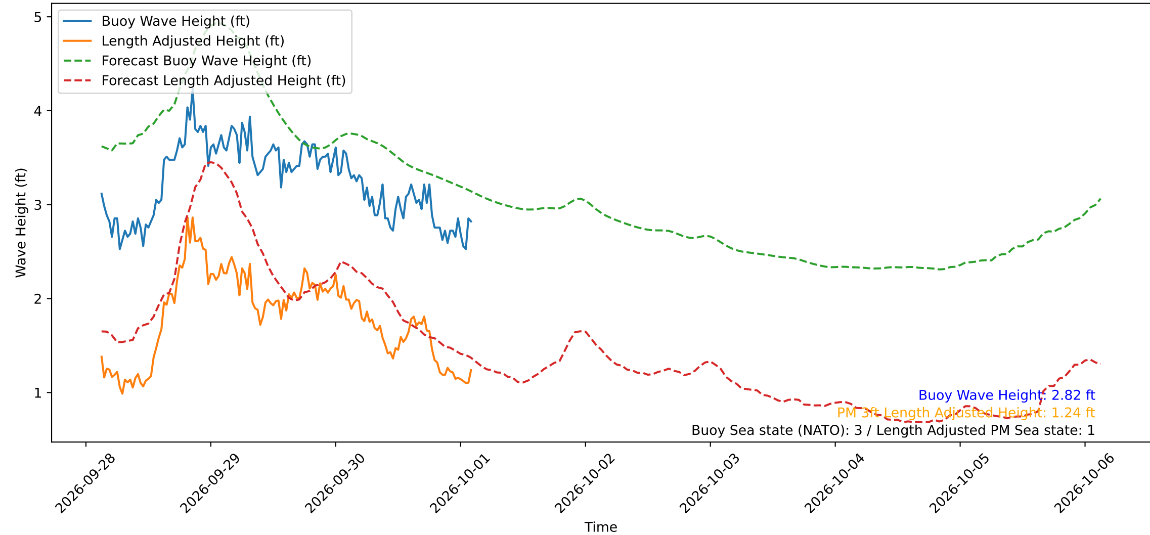
Wave Heights over Time for Oceanside Harbor at 2026-10-01 03:10:30
