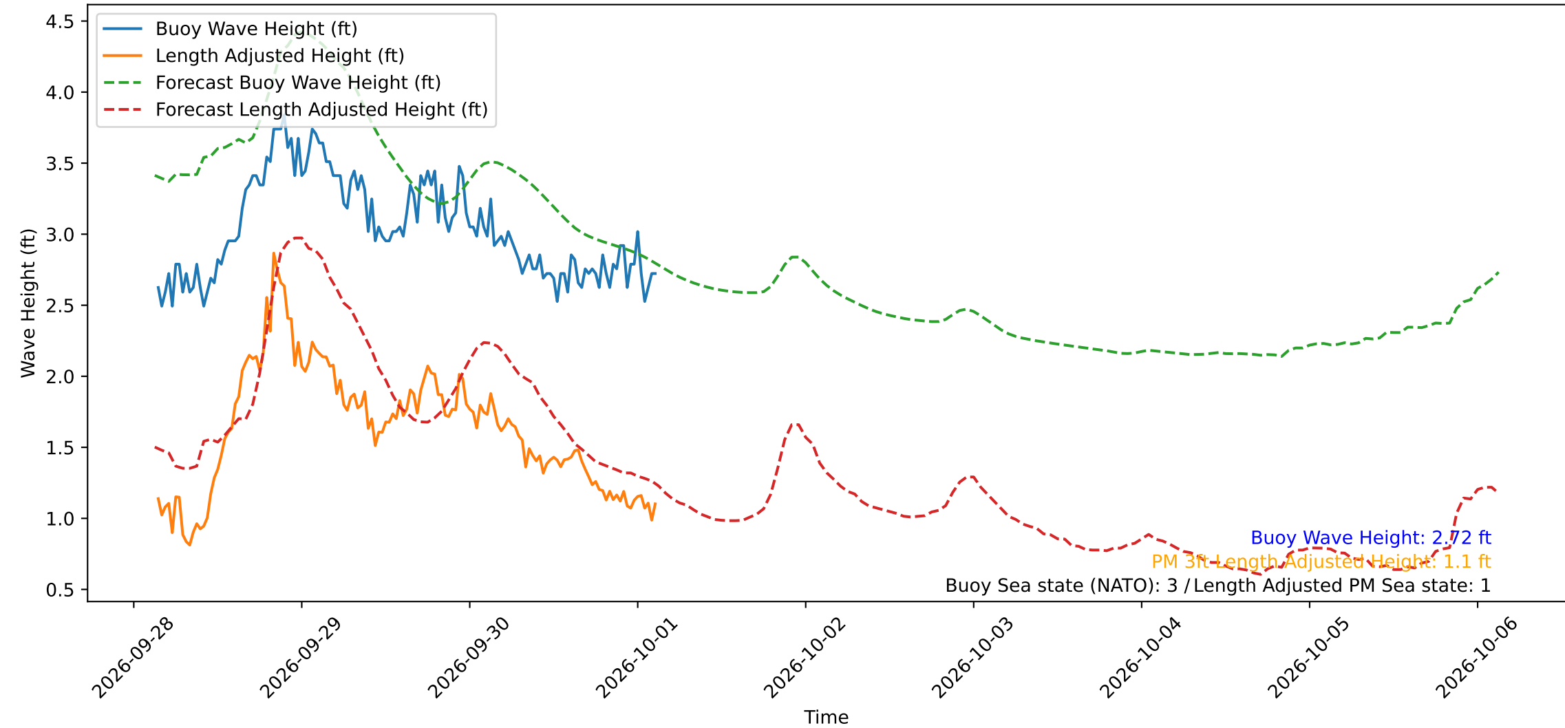
Wave Heights over Time for Red Beach at 2026-10-01 03:10:50
