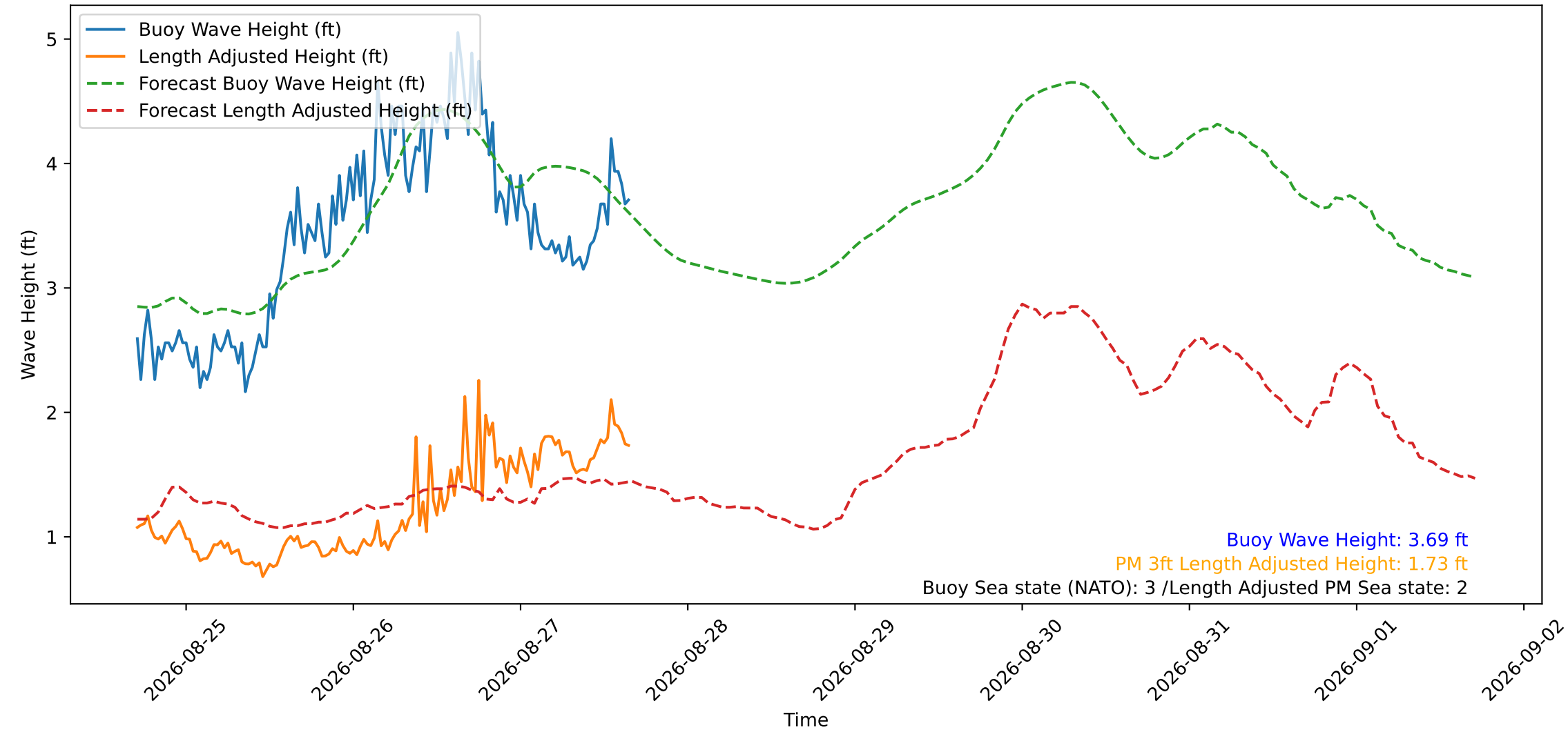
Wave Heights over Time for Red Beach at 2026-08-27 16:30:49
