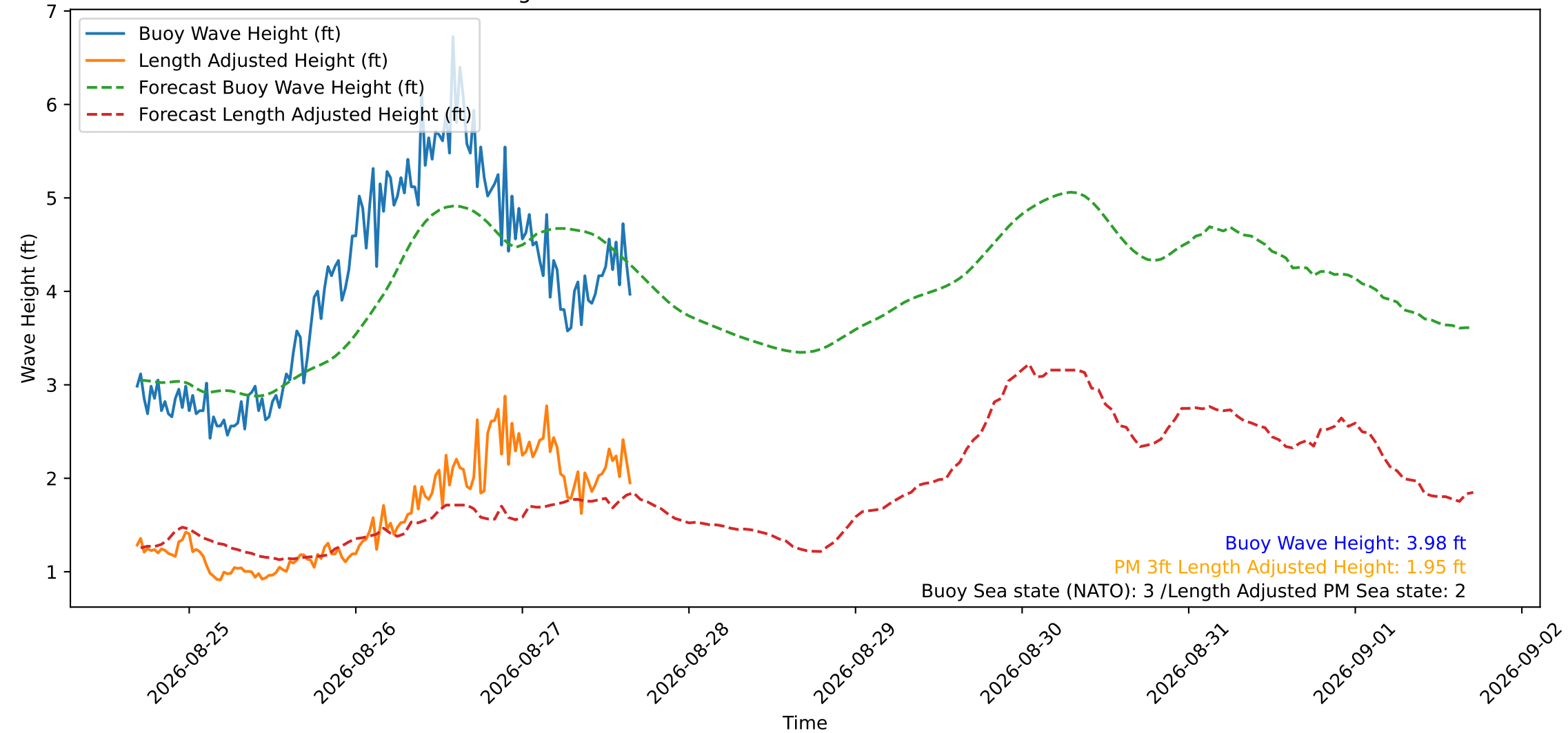
Wave Heights over Time for Oceanside Harbor at 2026-08-27 16:30:29
