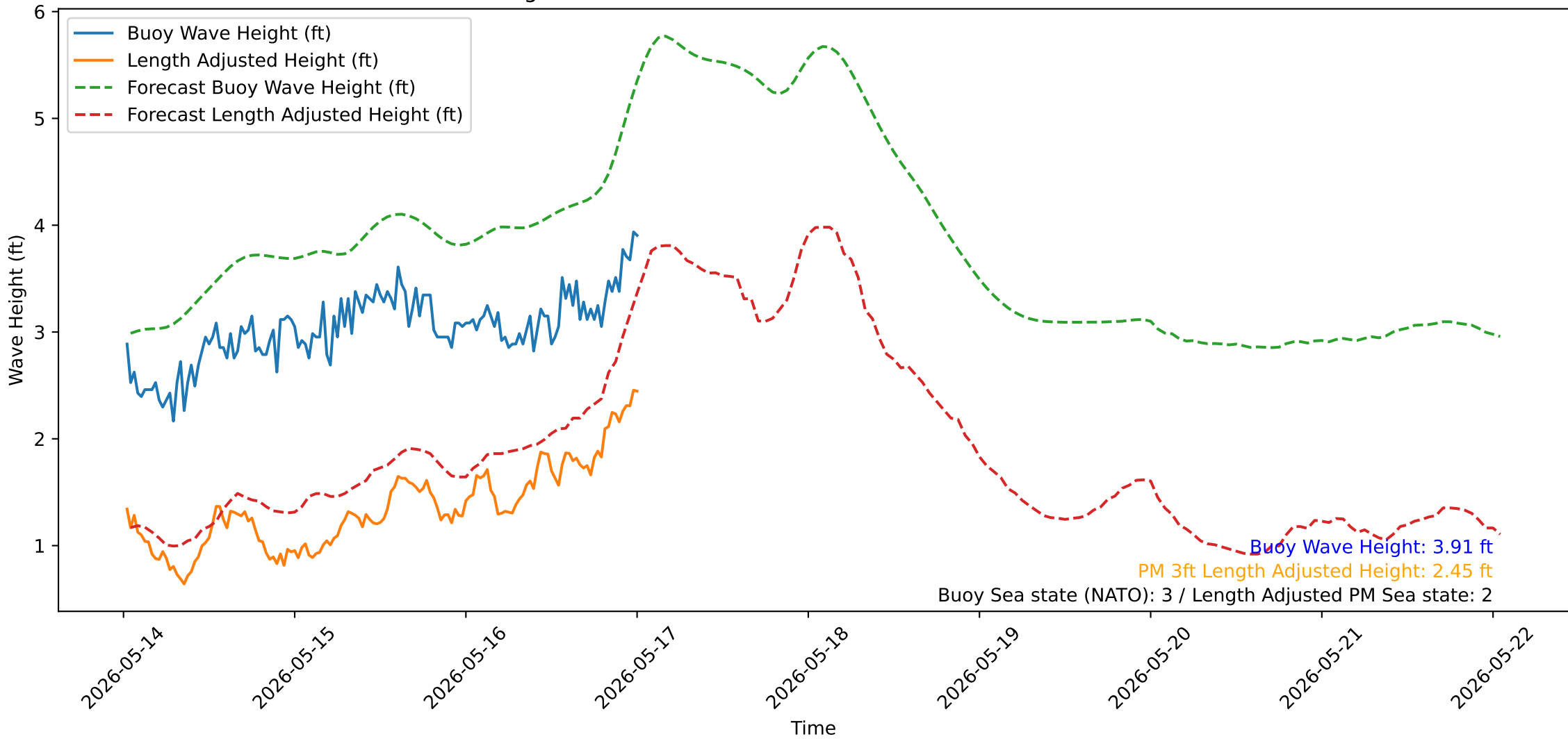
Wave Heights over Time for Oceanside Harbor at 2026-05-17 00:40:31
