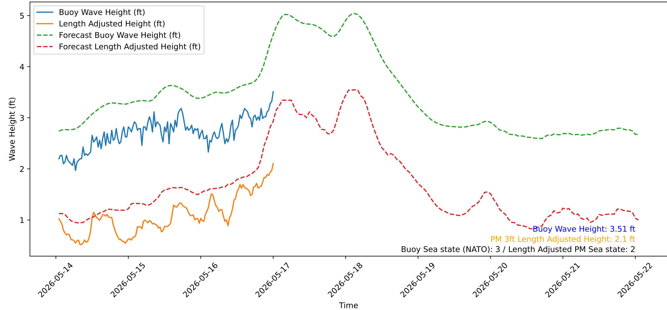
Wave Heights over Time for Red Beach at 2026-05-17 00:40:50
