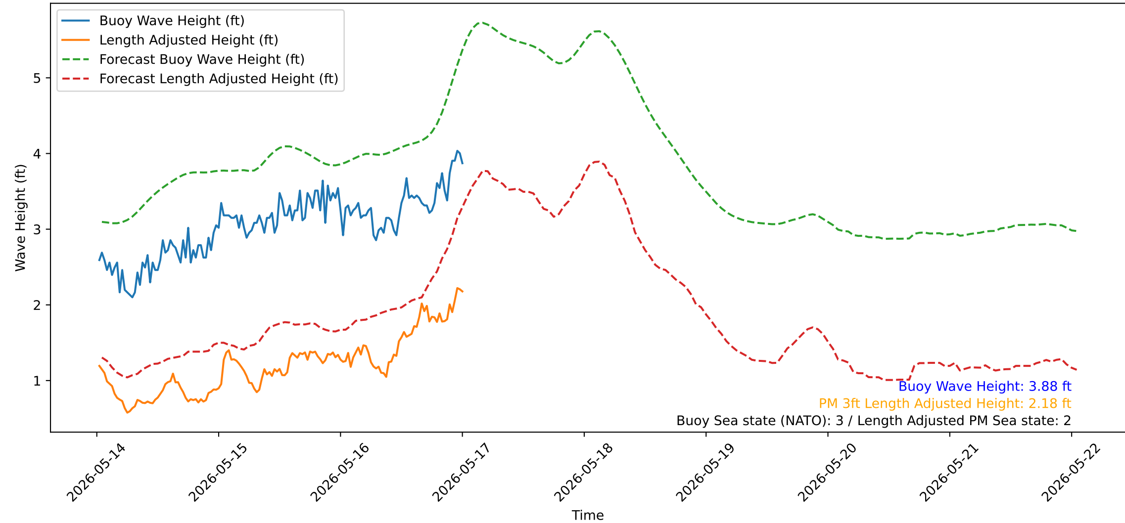
Wave Heights over Time for Green Beach at 2026-05-17 00:41:13
