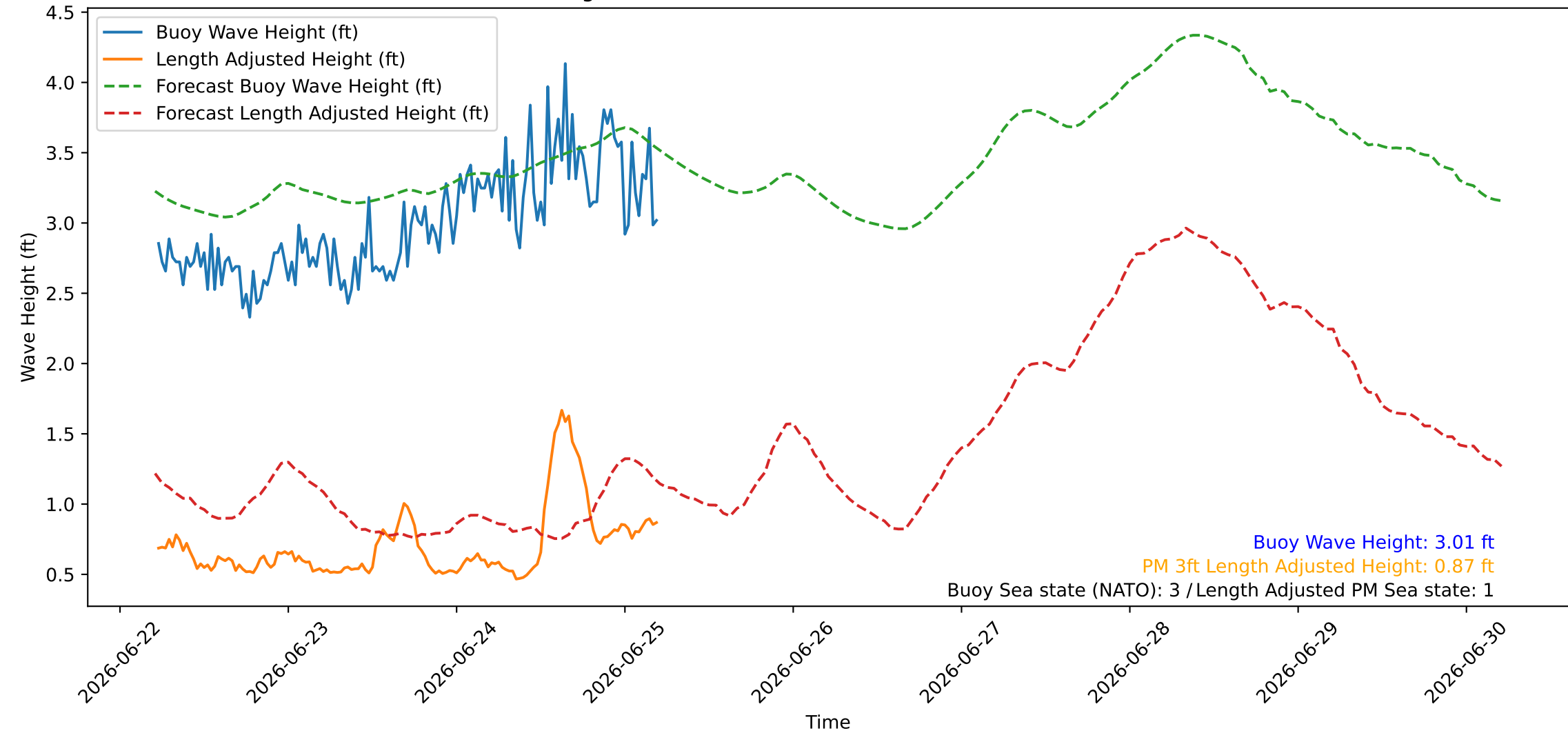
Wave Heights over Time for Red Beach at 2026-06-25 05:10:45
