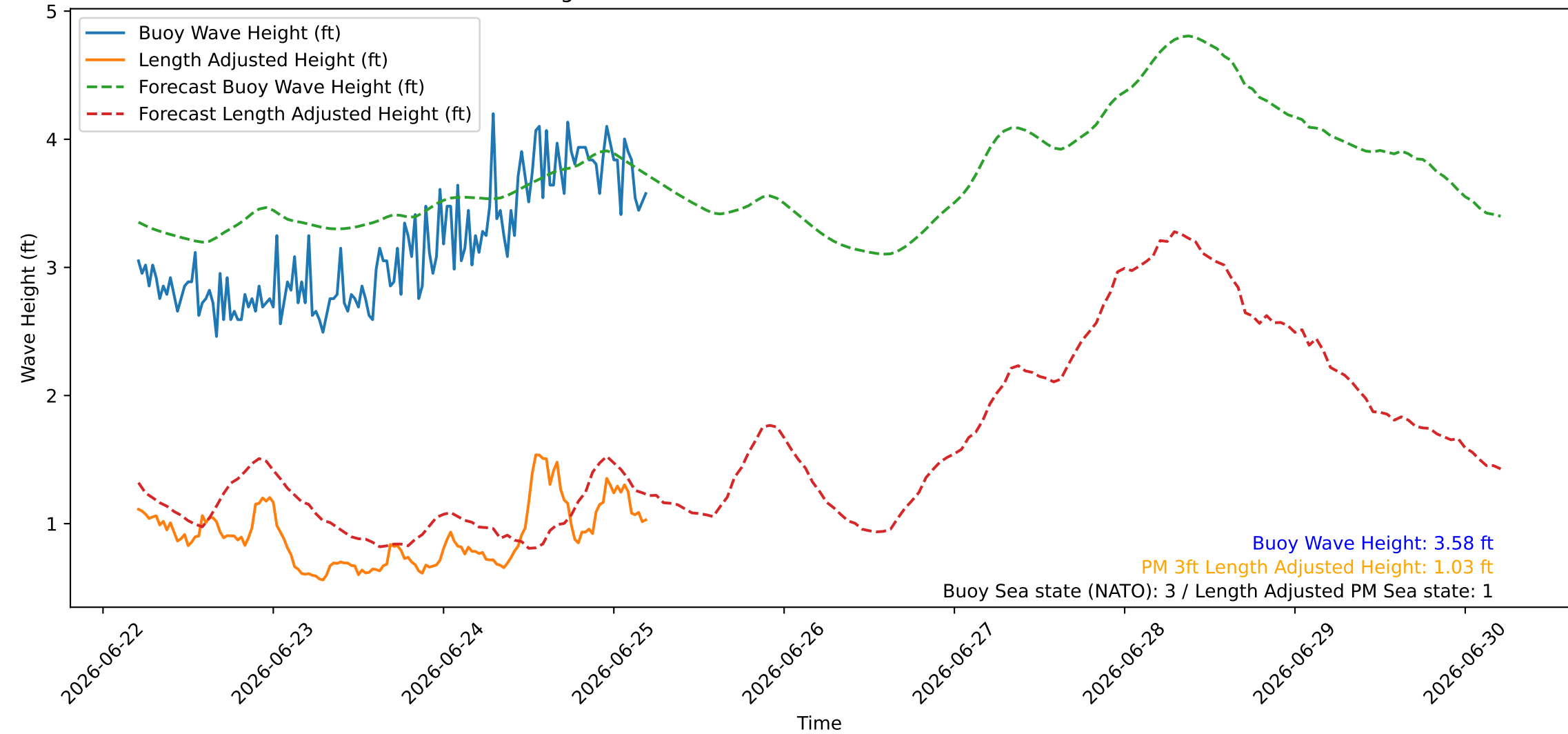
Wave Heights over Time for Green Beach at 2026-06-25 05:11:07
