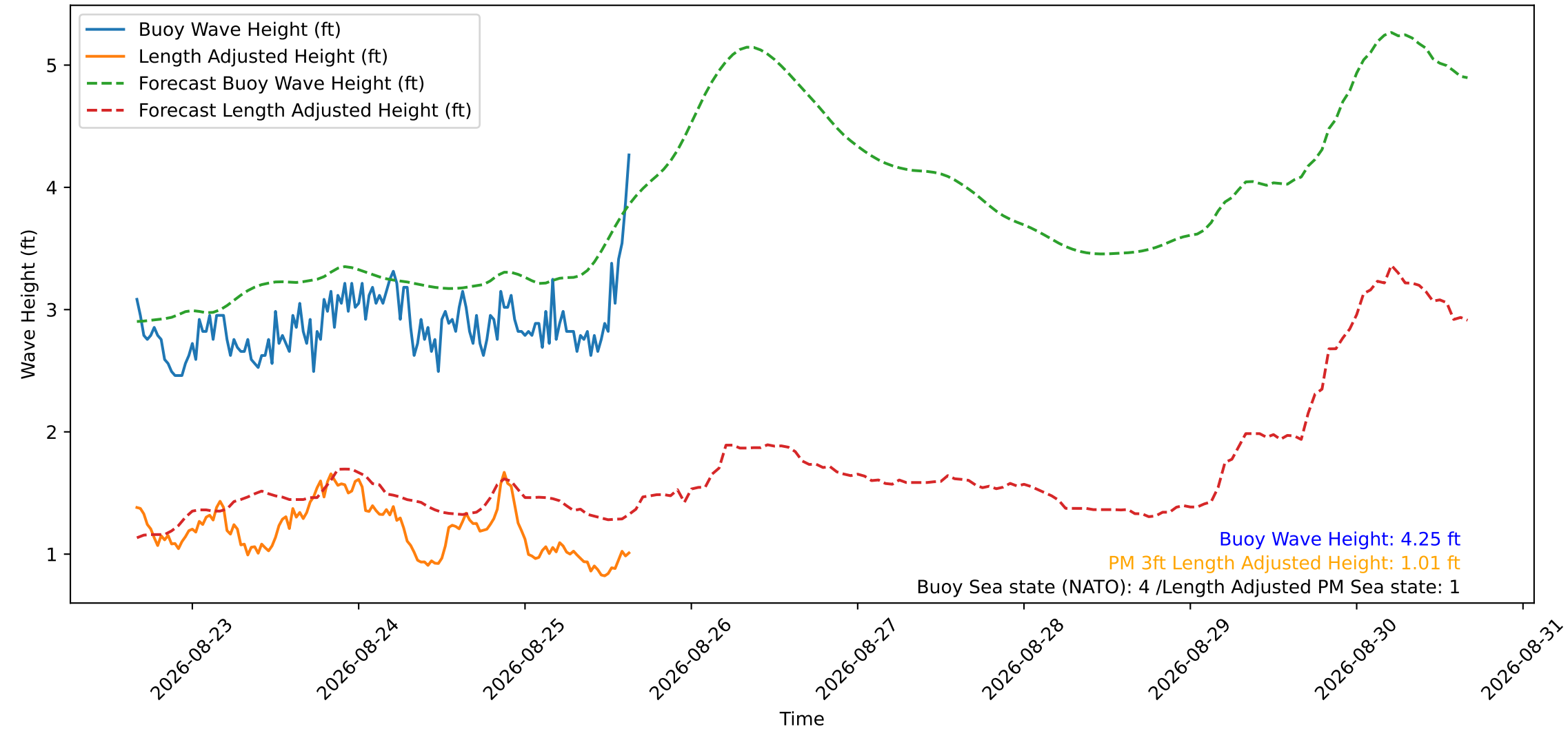
Wave Heights over Time for Green Beach at 2026-08-25 15:41:11
