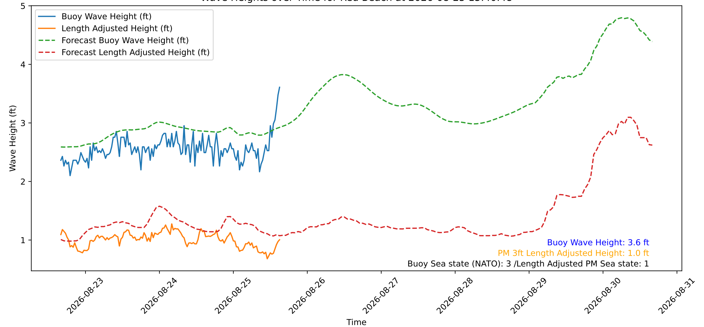
Wave Heights over Time for Red Beach at 2026-08-25 15:40:48
