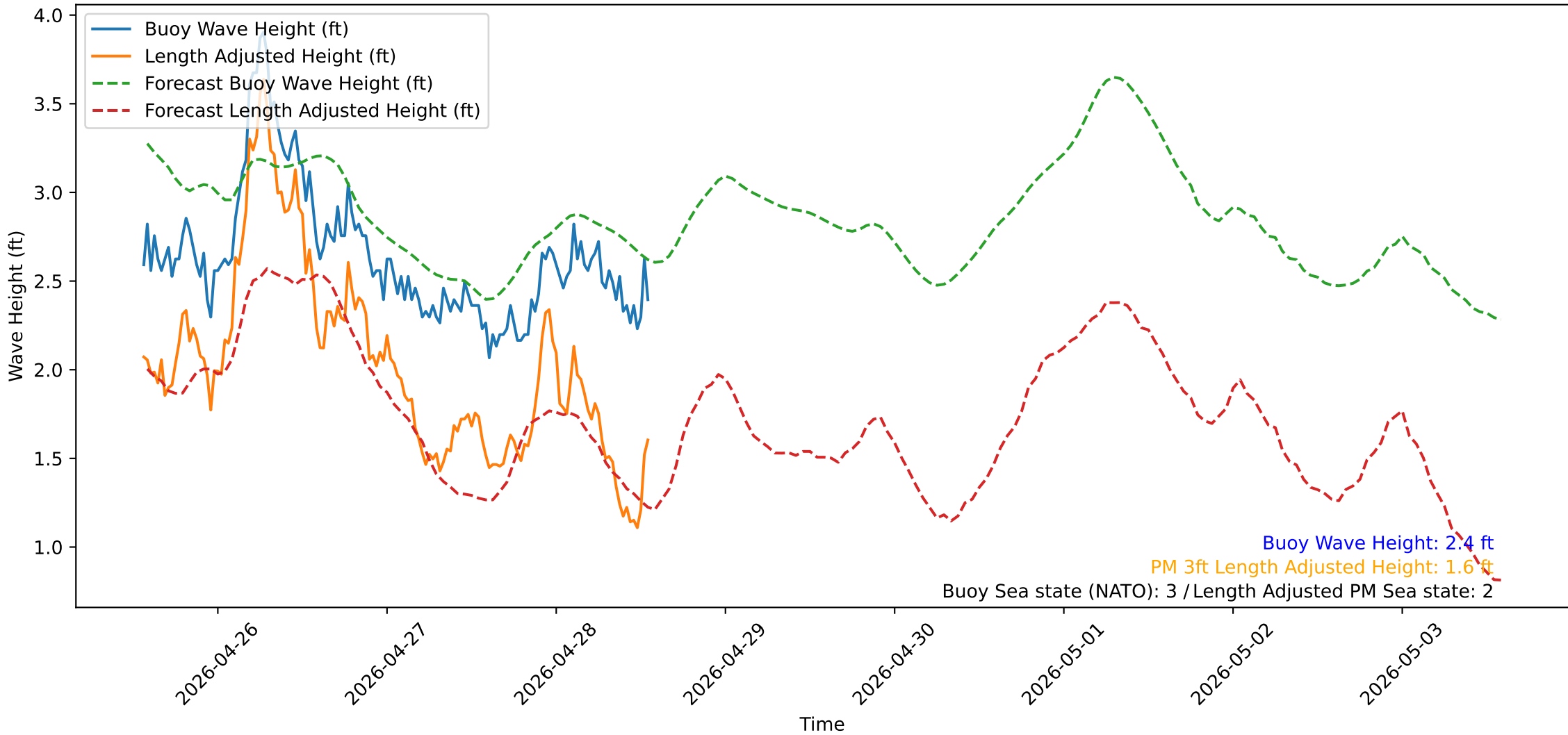
Wave Heights over Time for Oceanside Harbor at 2026-04-28 13:40:31
