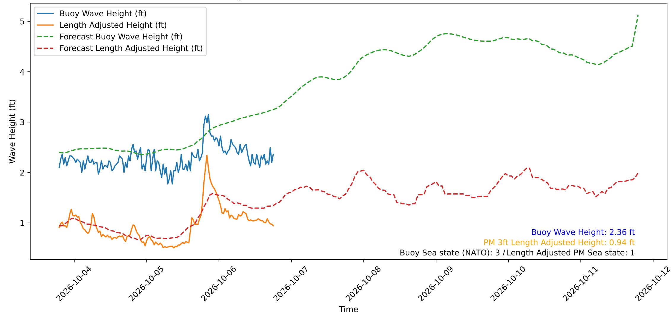
Wave Heights over Time for Green Beach at 2026-10-06 18:51:16
