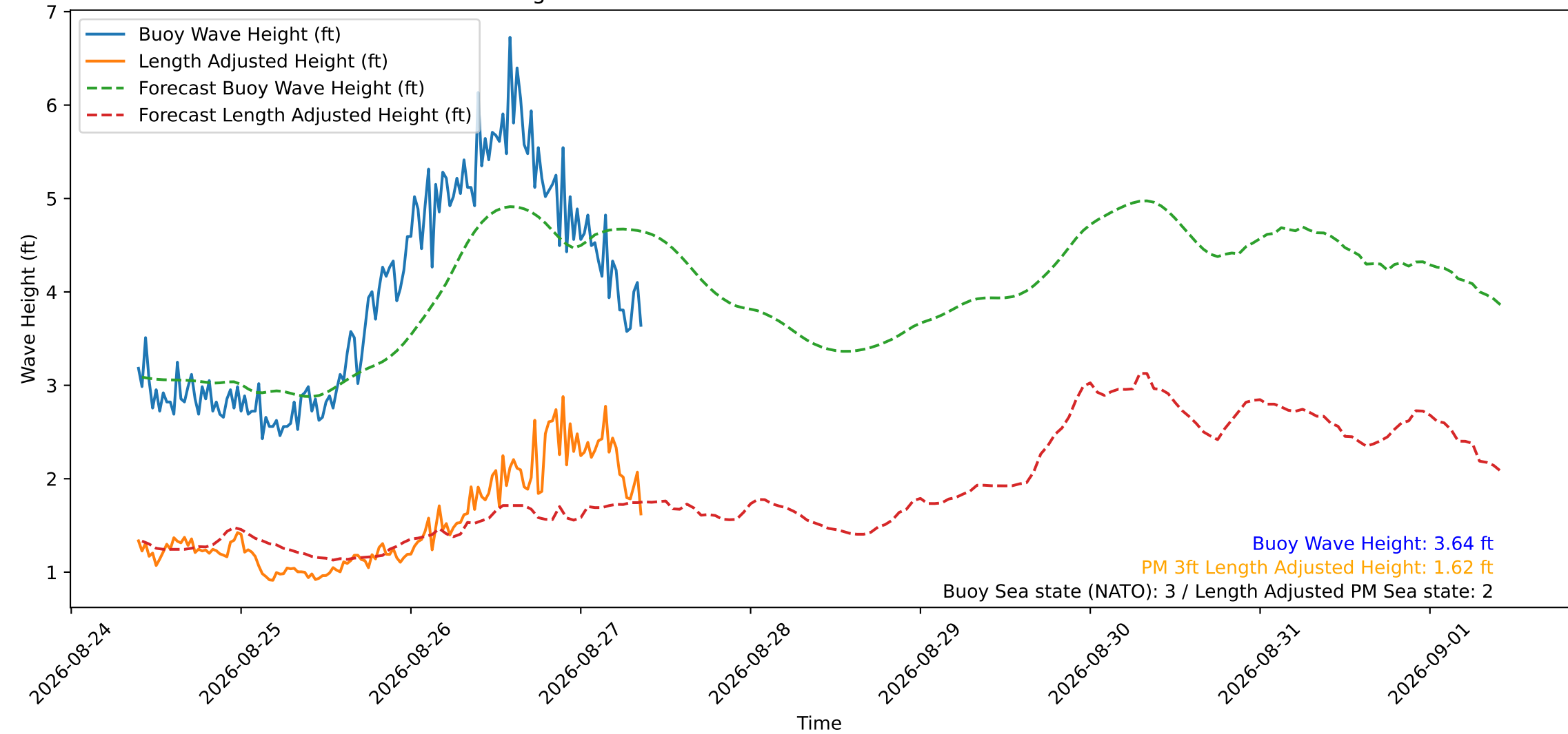
Wave Heights over Time for Oceanside Harbor at 2026-08-27 09:30:29
