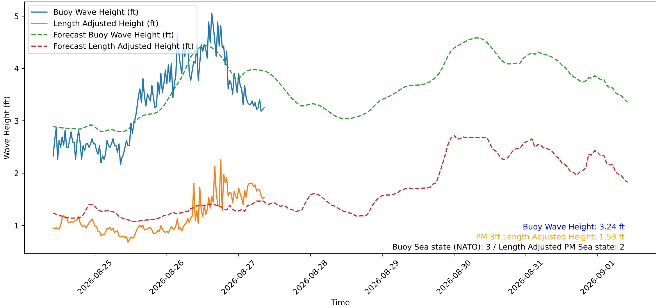
Wave Heights over Time for Red Beach at 2026-08-27 09:30:49
