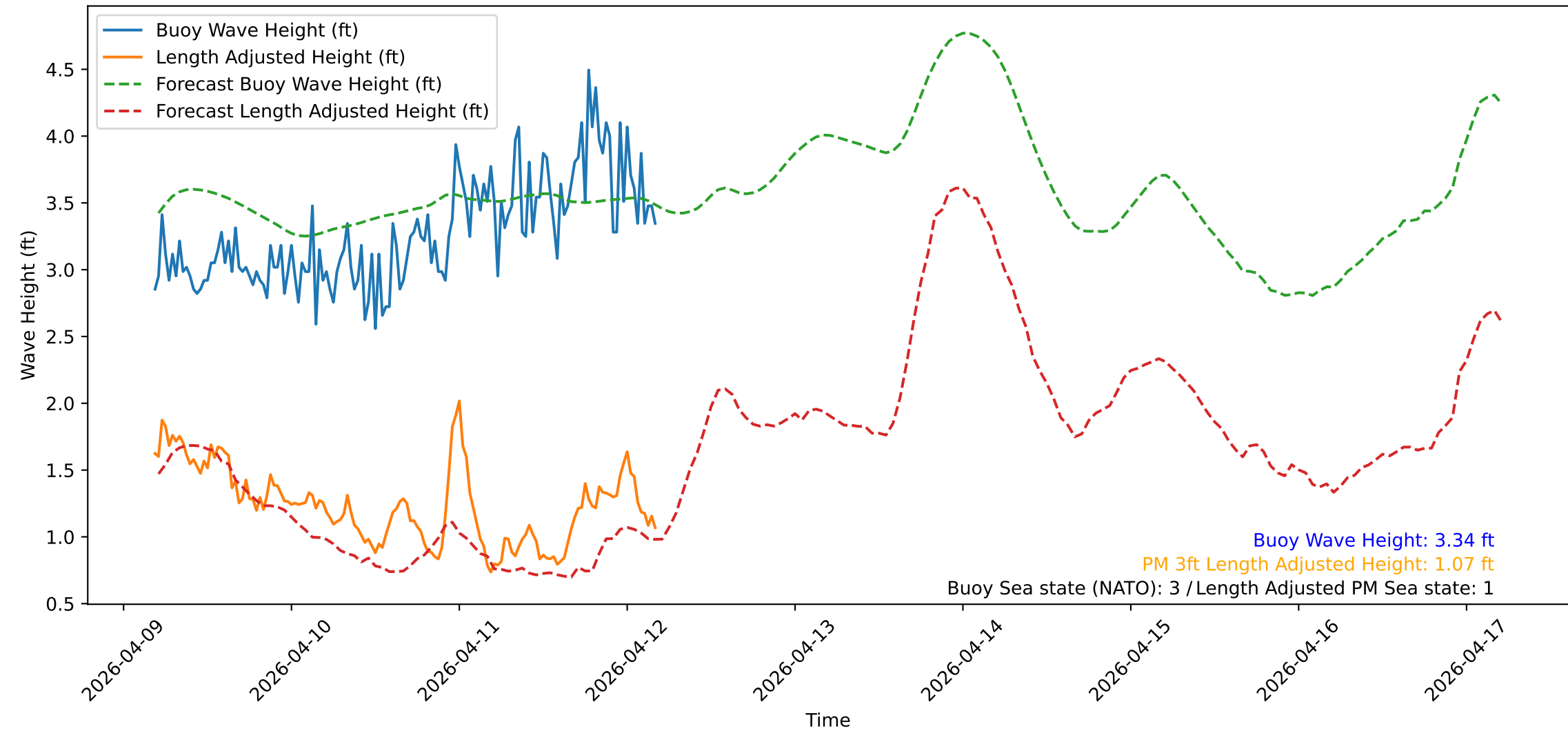
Wave Heights over Time for Green Beach at 2026-04-12 04:41:14
