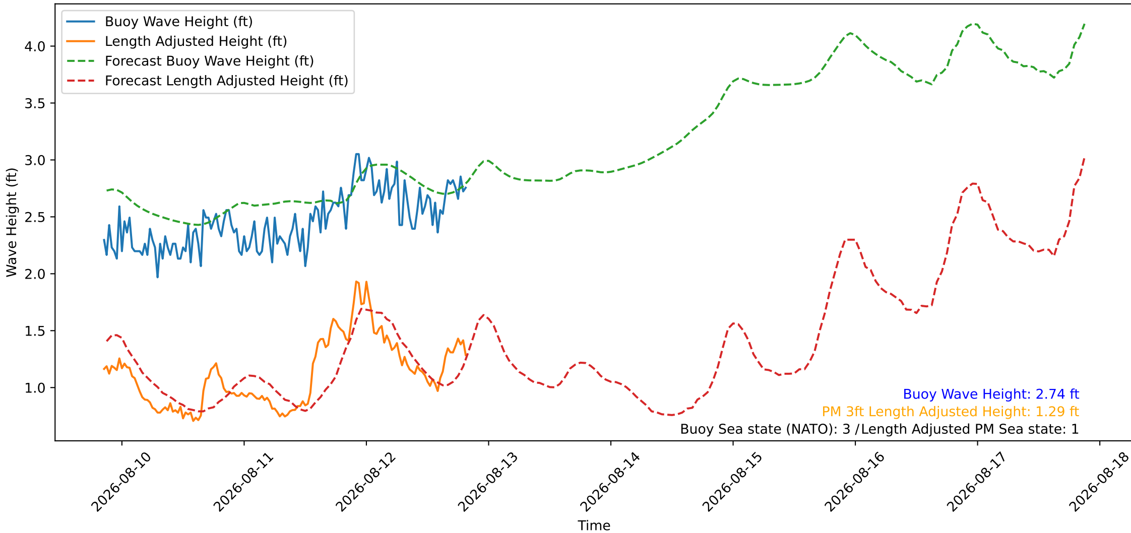
Wave Heights over Time for Oceanside Harbor at 2026-08-12 20:30:26
