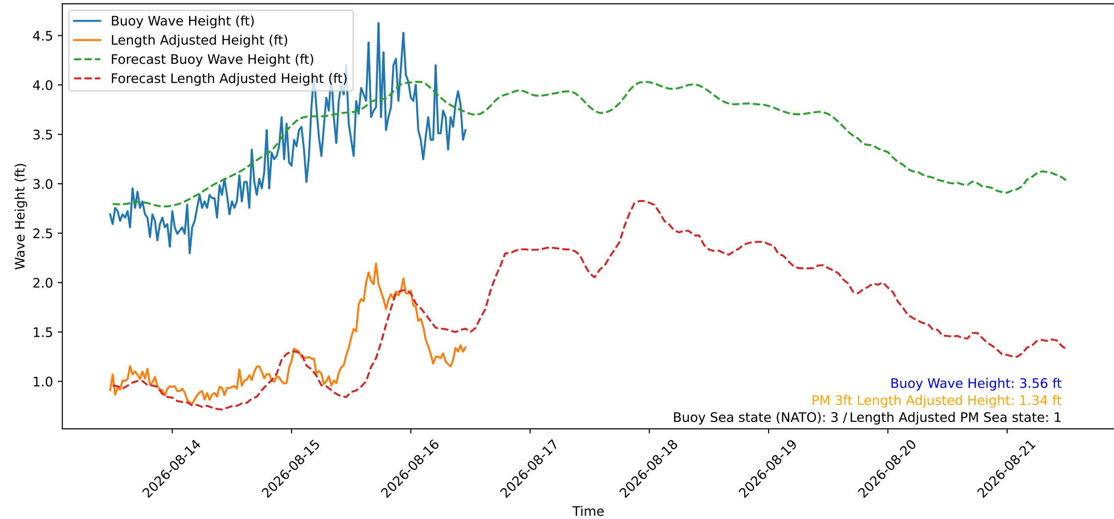
Wave Heights over Time for Oceanside Harbor at 2026-08-16 11:40:26
