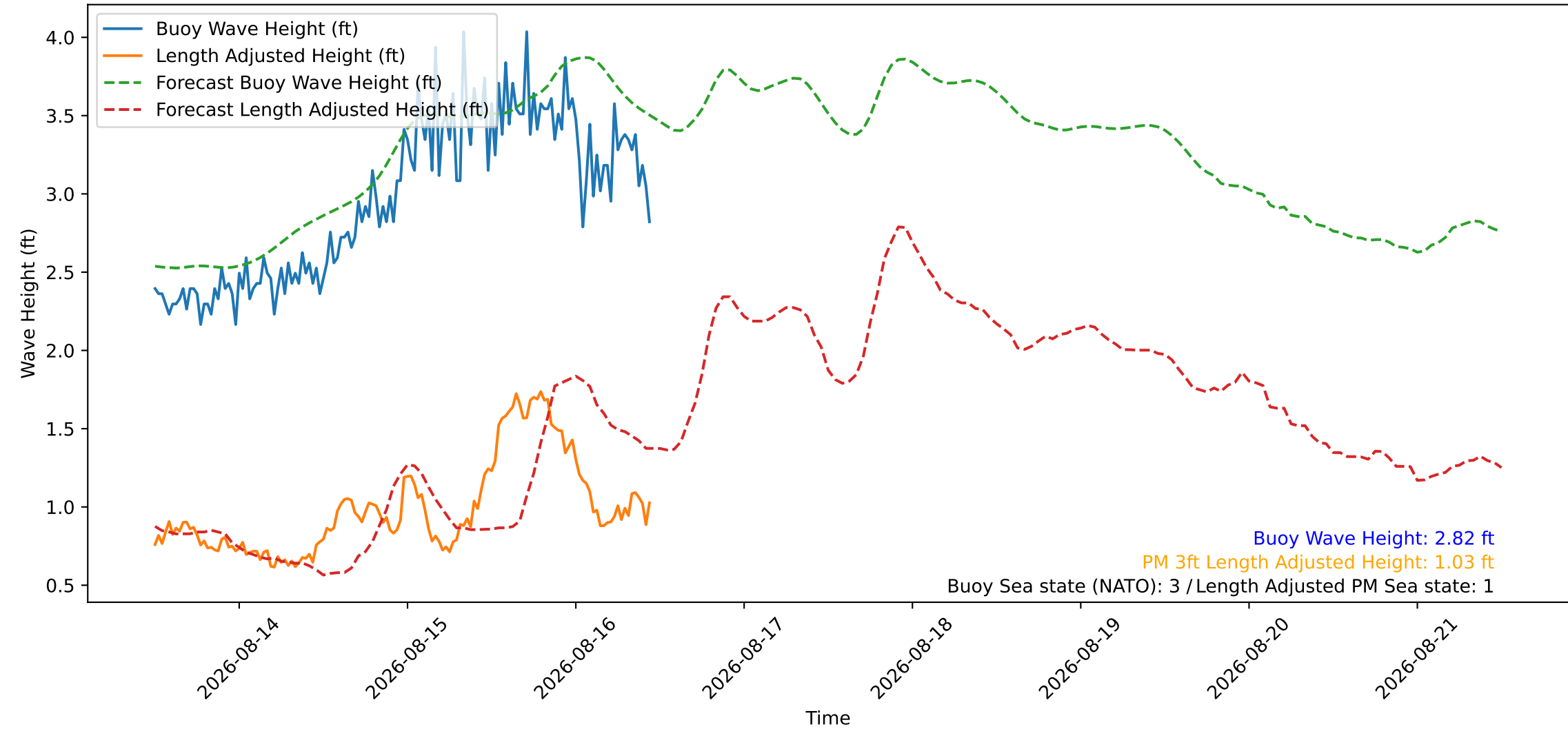
Wave Heights over Time for Red Beach at 2026-08-16 11:40:45
