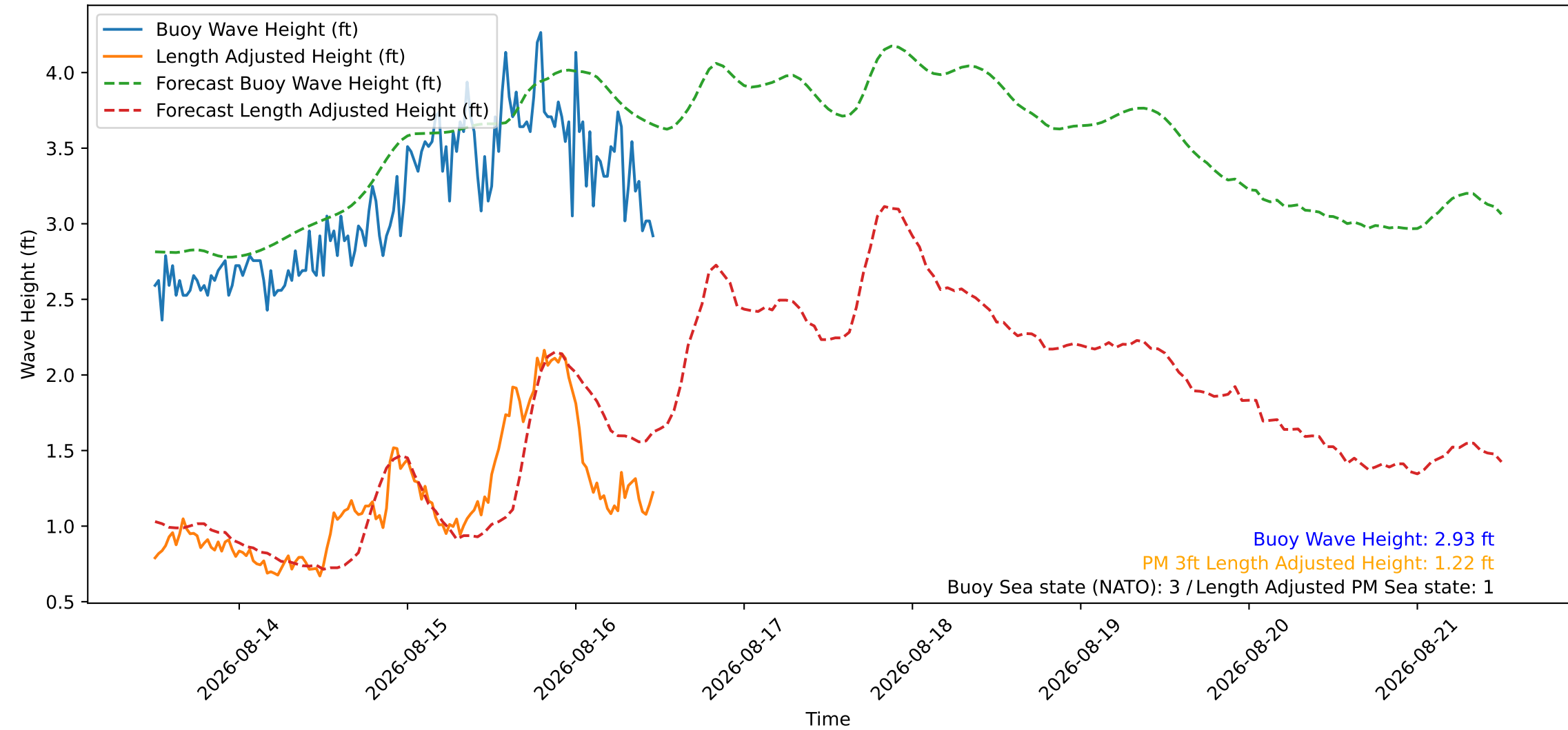
Wave Heights over Time for Green Beach at 2026-08-16 11:41:07
