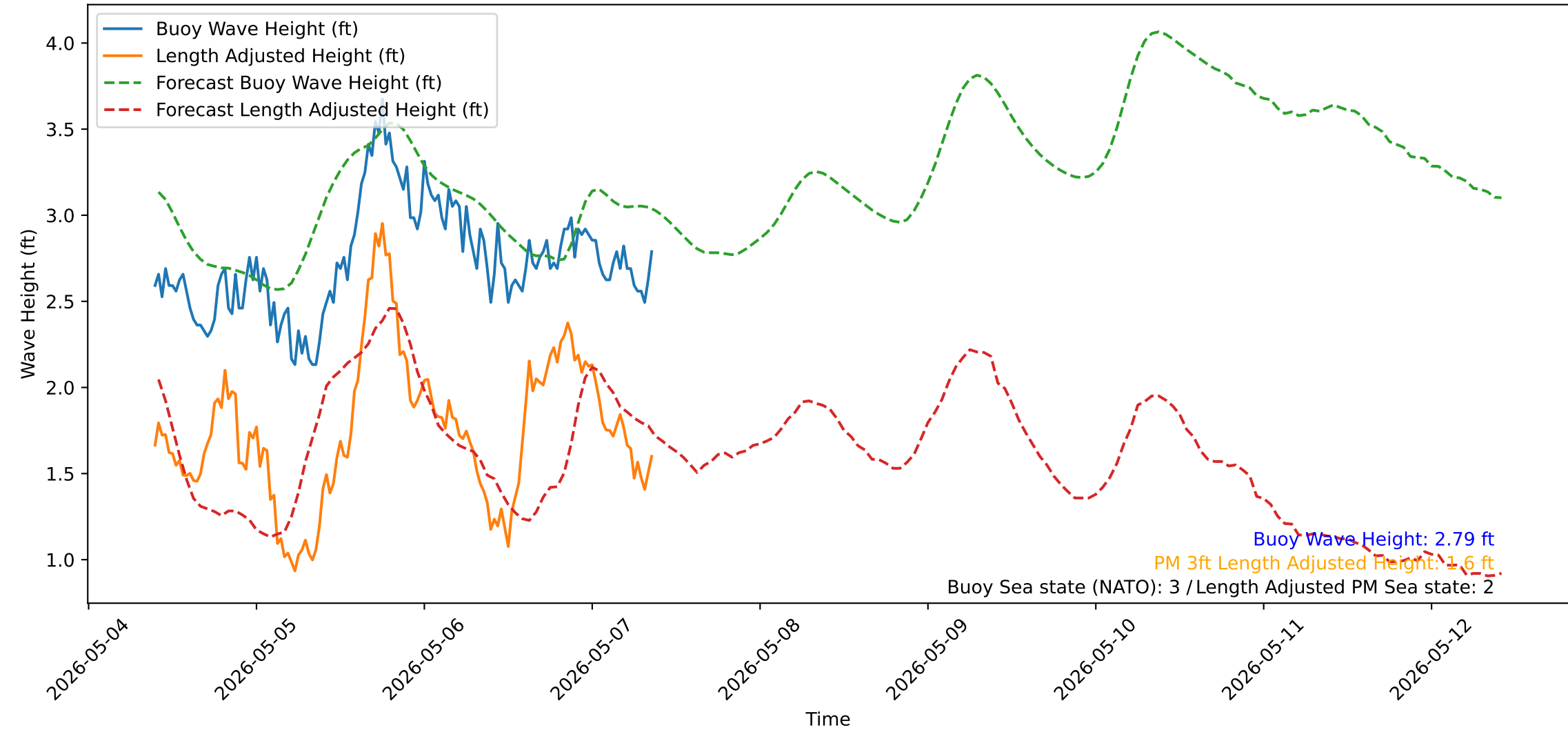
Wave Heights over Time for Green Beach at 2026-05-07 09:31:12
