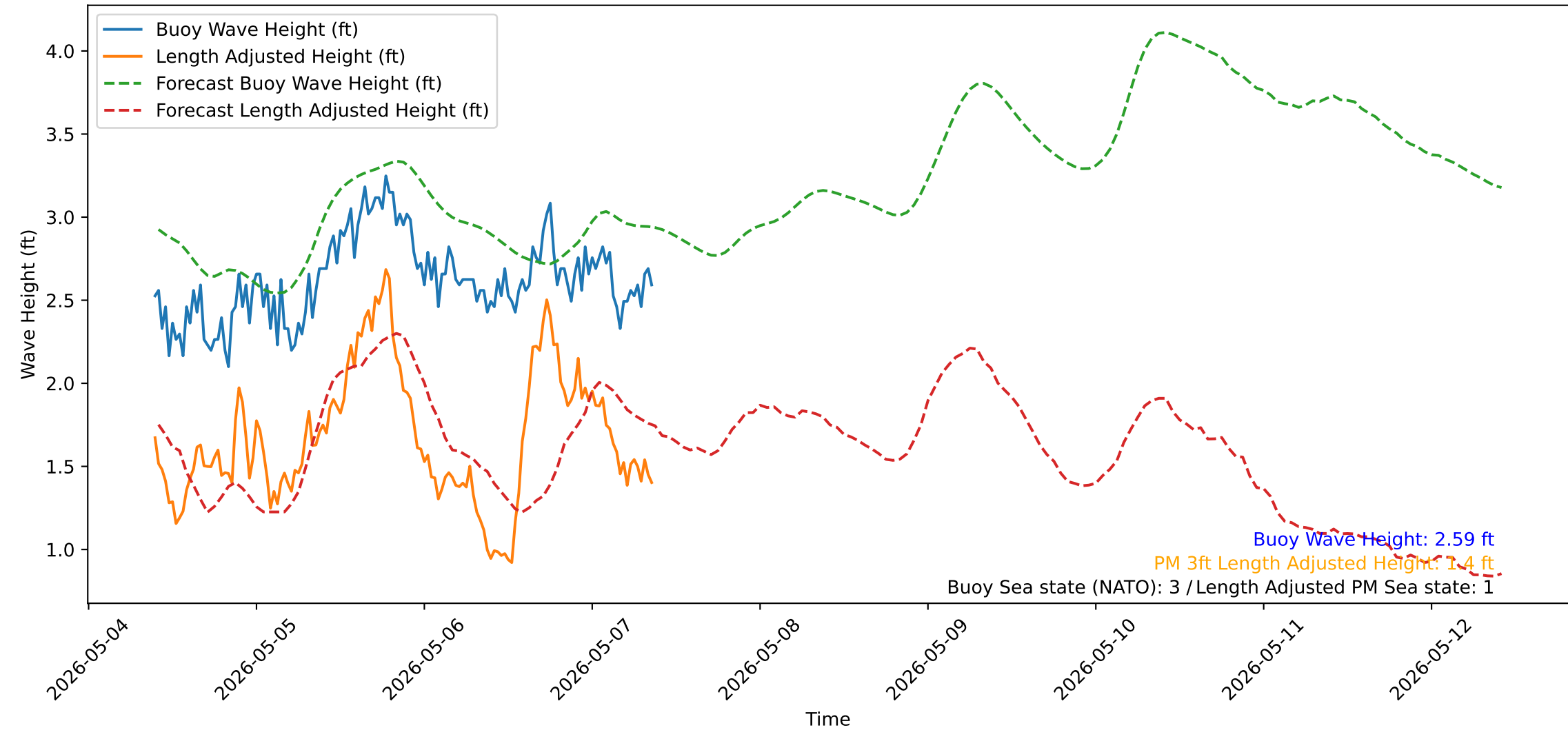
Wave Heights over Time for Oceanside Harbor at 2026-05-07 09:30:31
