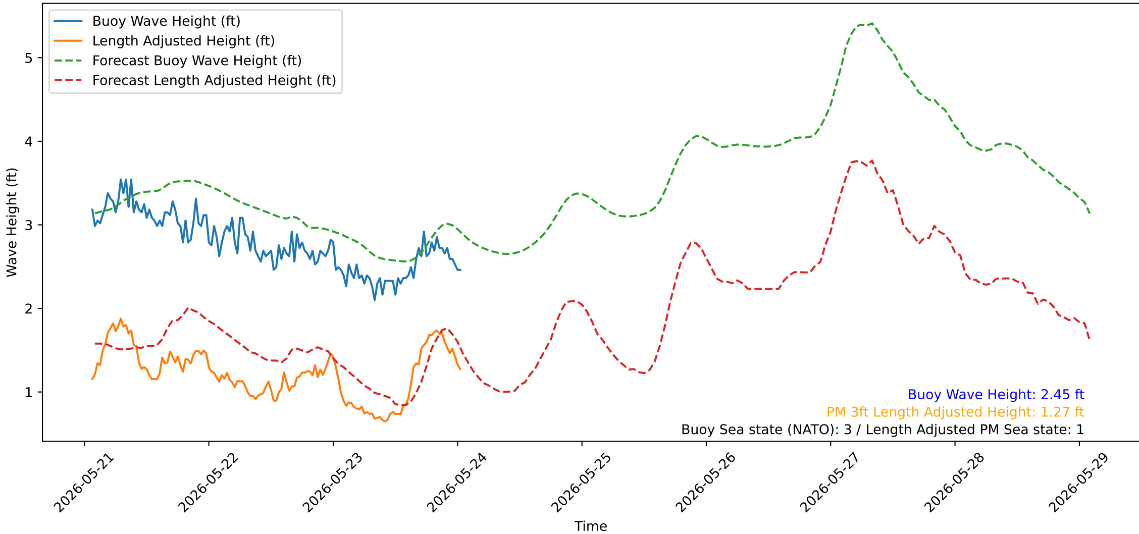
Wave Heights over Time for Green Beach at 2026-05-24 01:31:14
