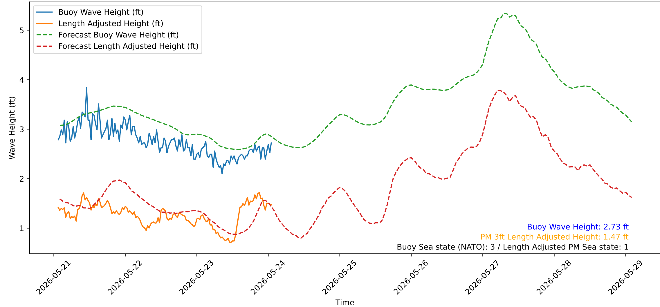
Wave Heights over Time for Oceanside Harbor at 2026-05-24 01:30:32
