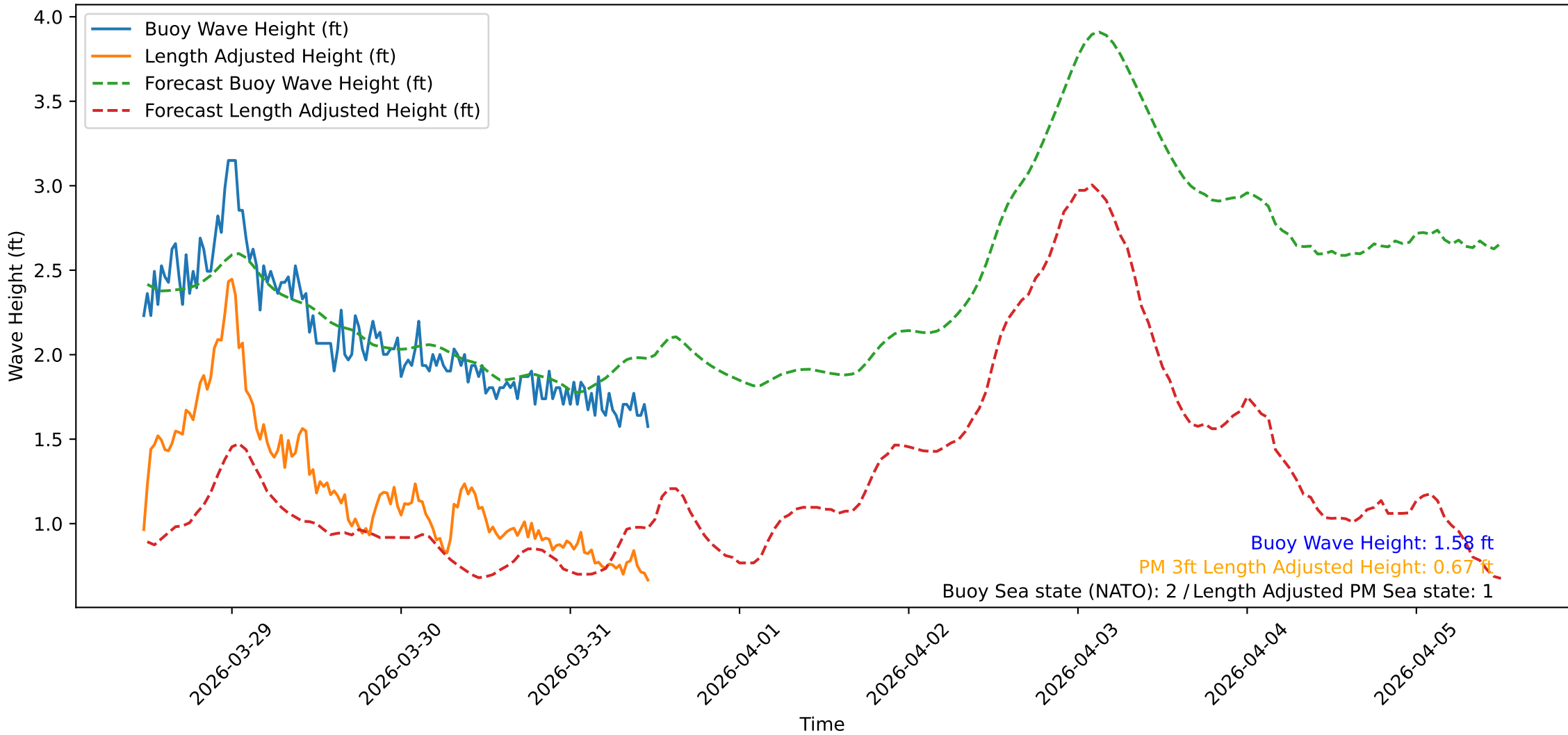
Wave Heights over Time for Oceanside Harbor at 2026-03-31 11:40:31
