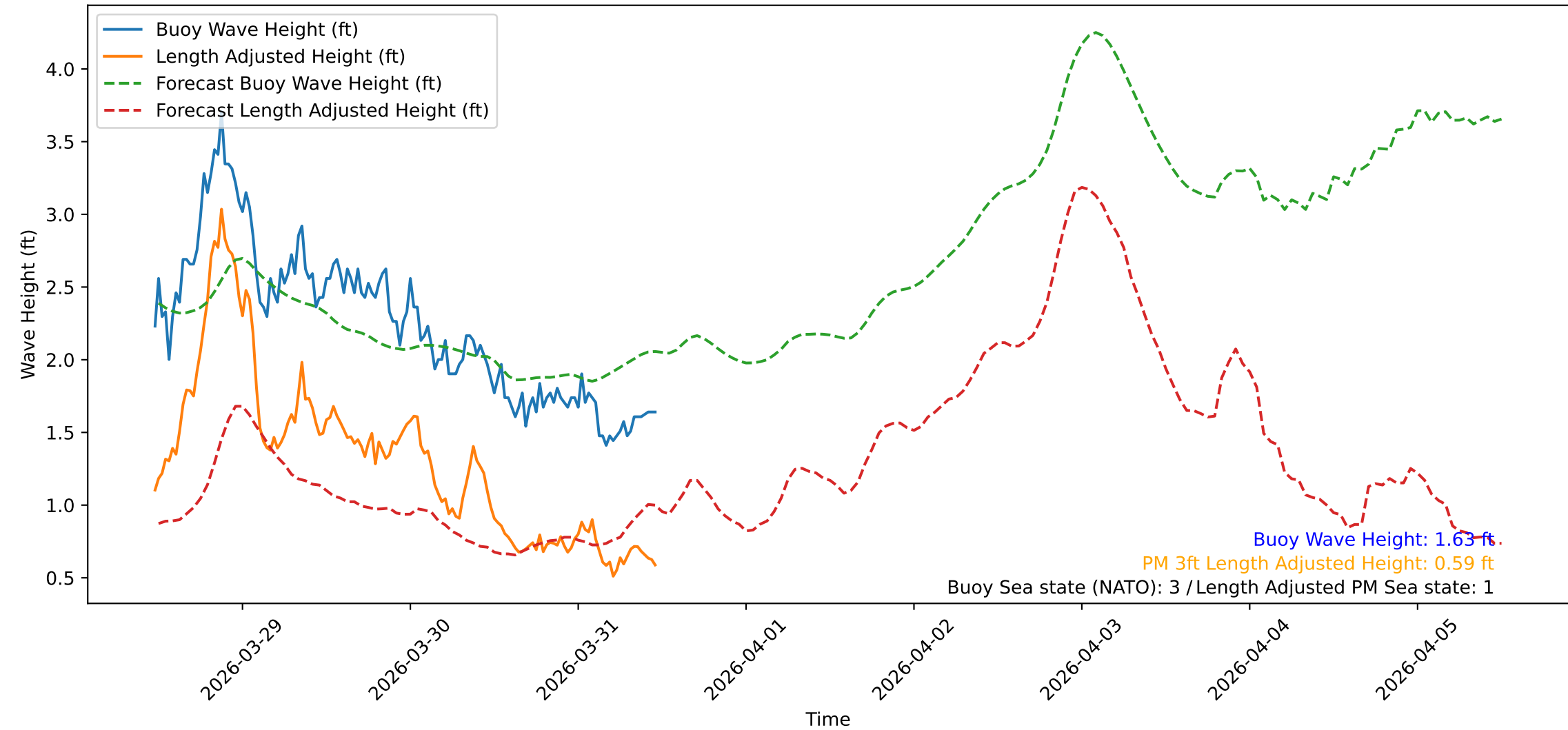
Wave Heights over Time for Green Beach at 2026-03-31 11:41:09
