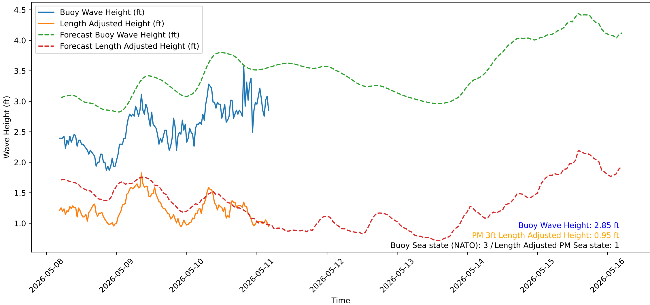
Wave Heights over Time for Oceanside Harbor at 2026-05-11 04:30:31
