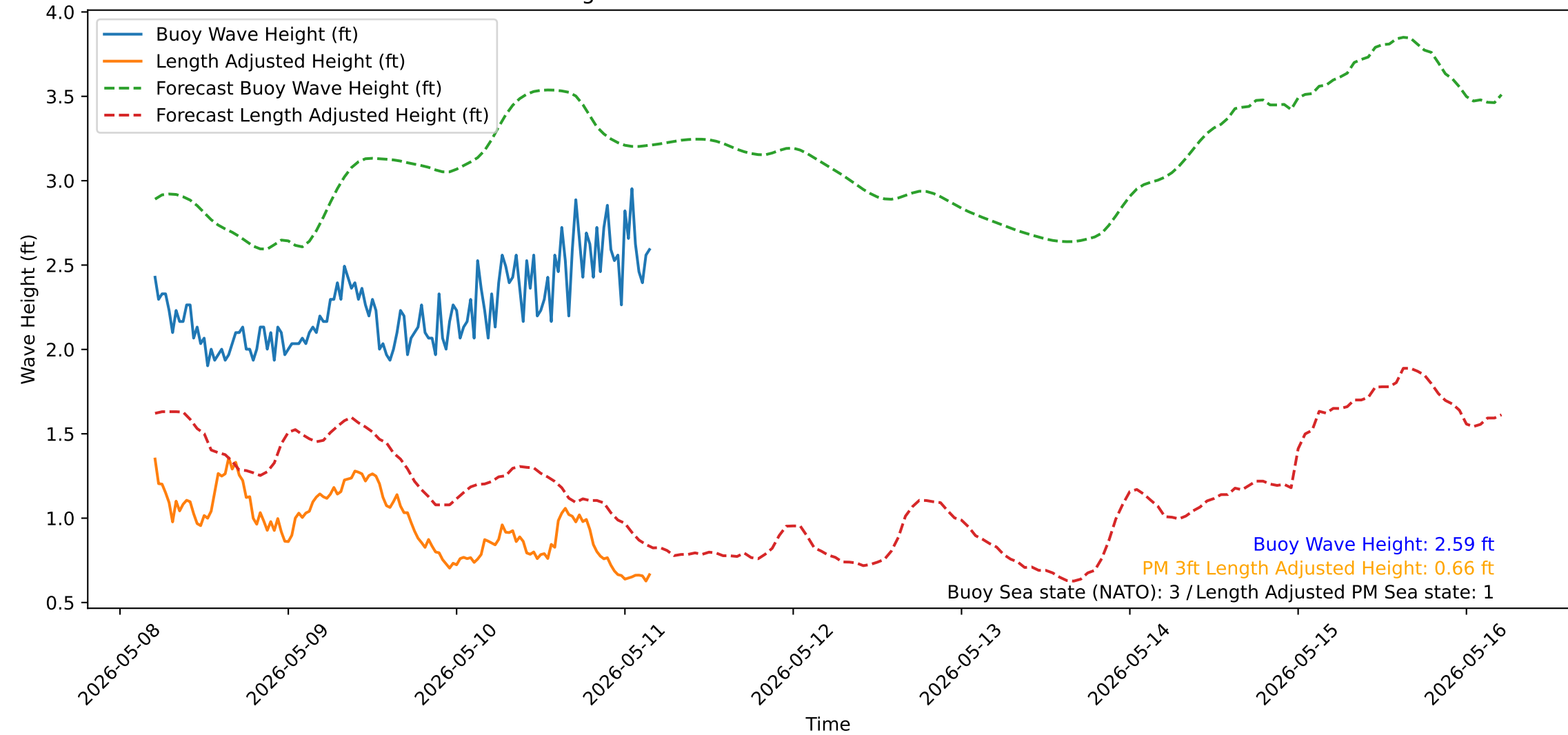
Wave Heights over Time for Red Beach at 2026-05-11 04:30:50
