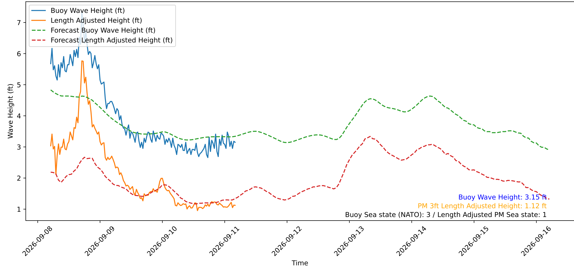
Wave Heights over Time for Oceanside Harbor at 2026-09-11 04:50:30
