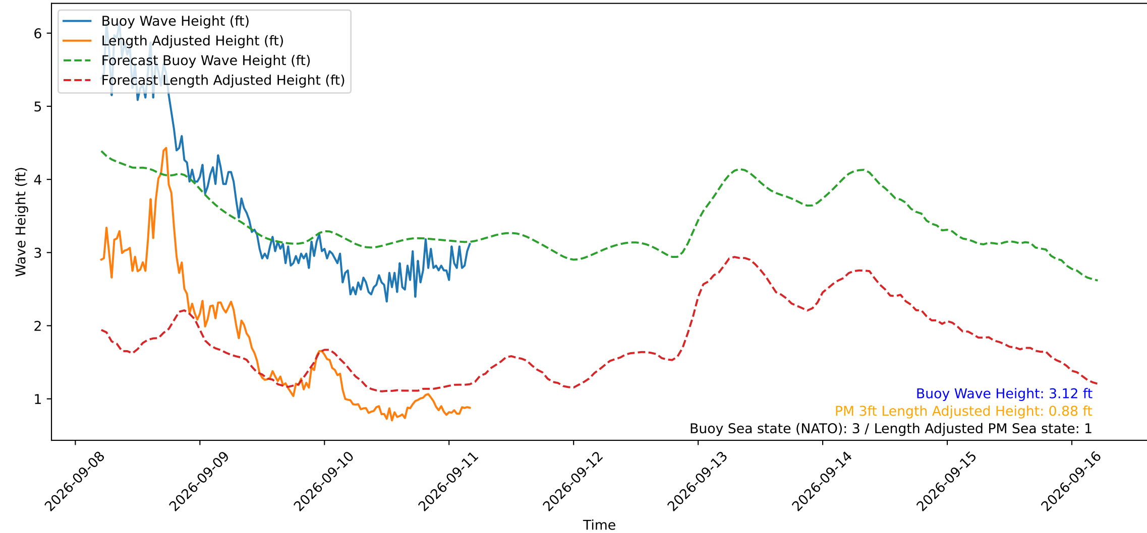
Wave Heights over Time for Red Beach at 2026-09-11 04:50:51
