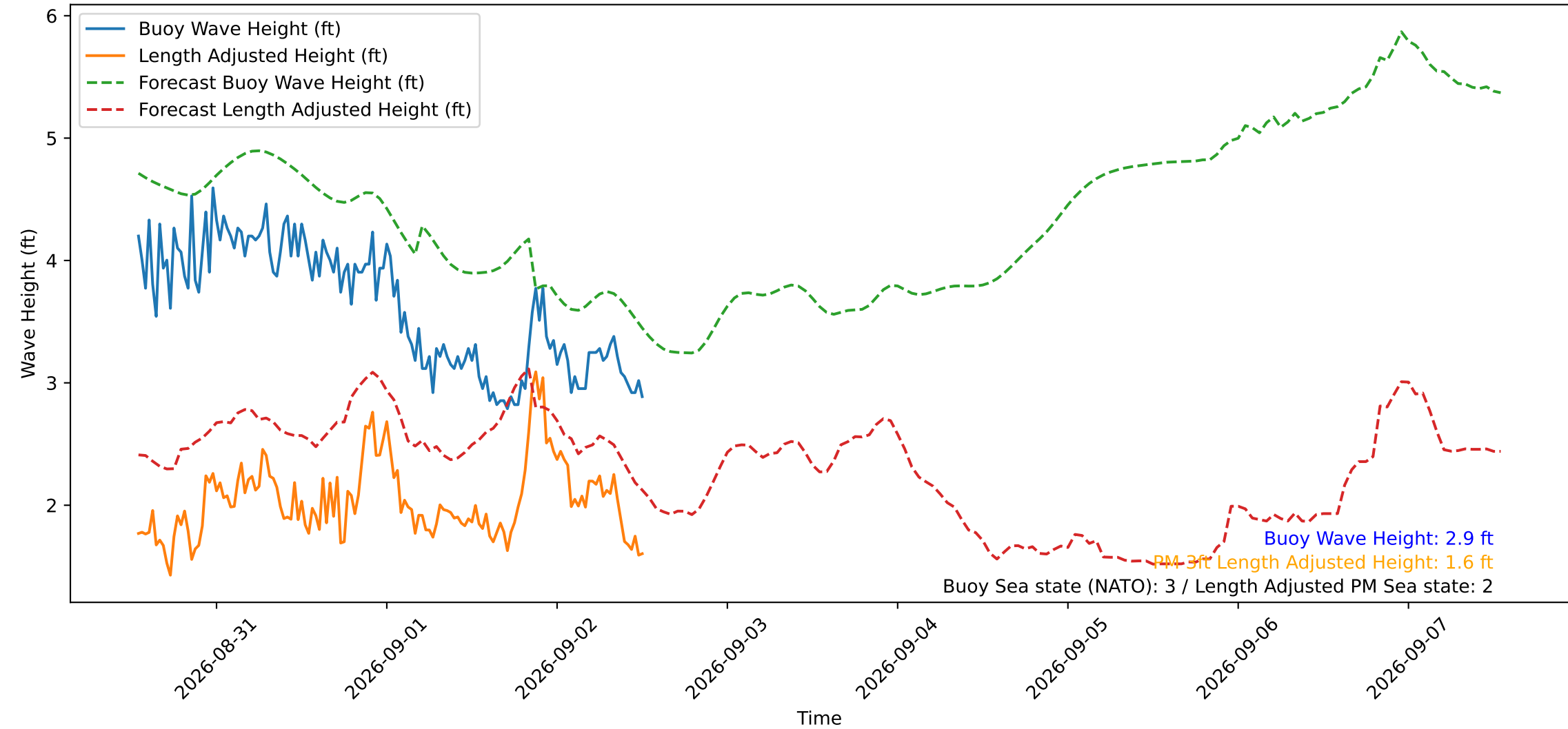
Wave Heights over Time for Green Beach at 2026-09-02 12:41:12
