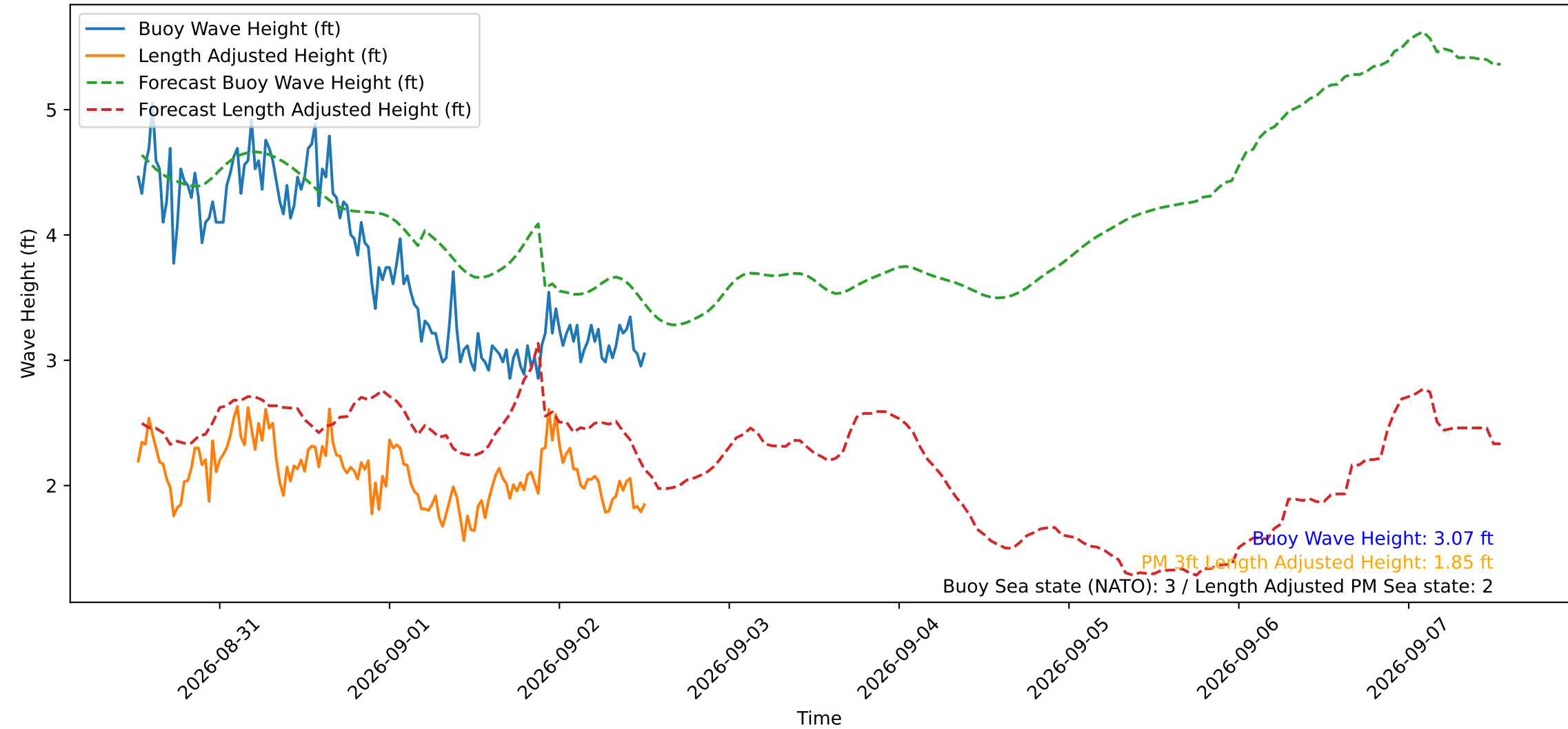
Wave Heights over Time for Oceanside Harbor at 2026-09-02 12:40:29
