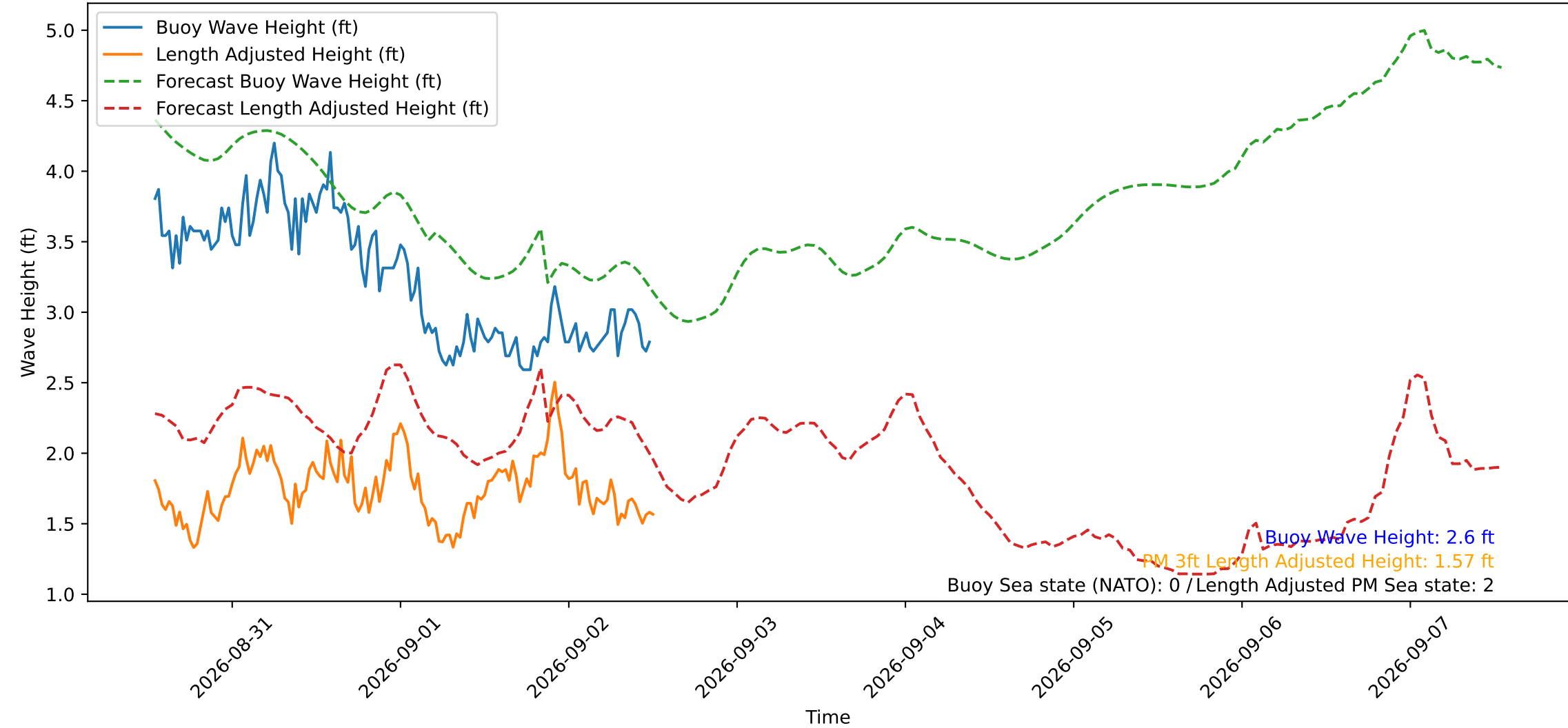
Wave Heights over Time for Red Beach at 2026-09-02 12:40:49
