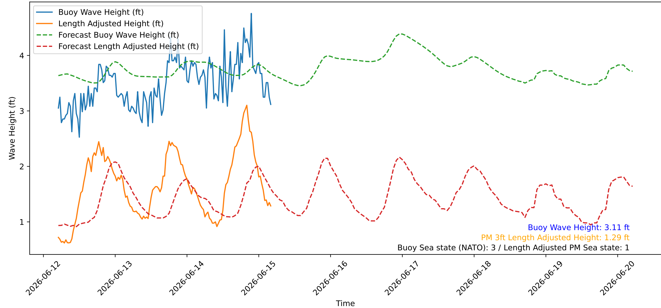
Wave Heights over Time for Red Beach at 2026-06-15 04:40:45
