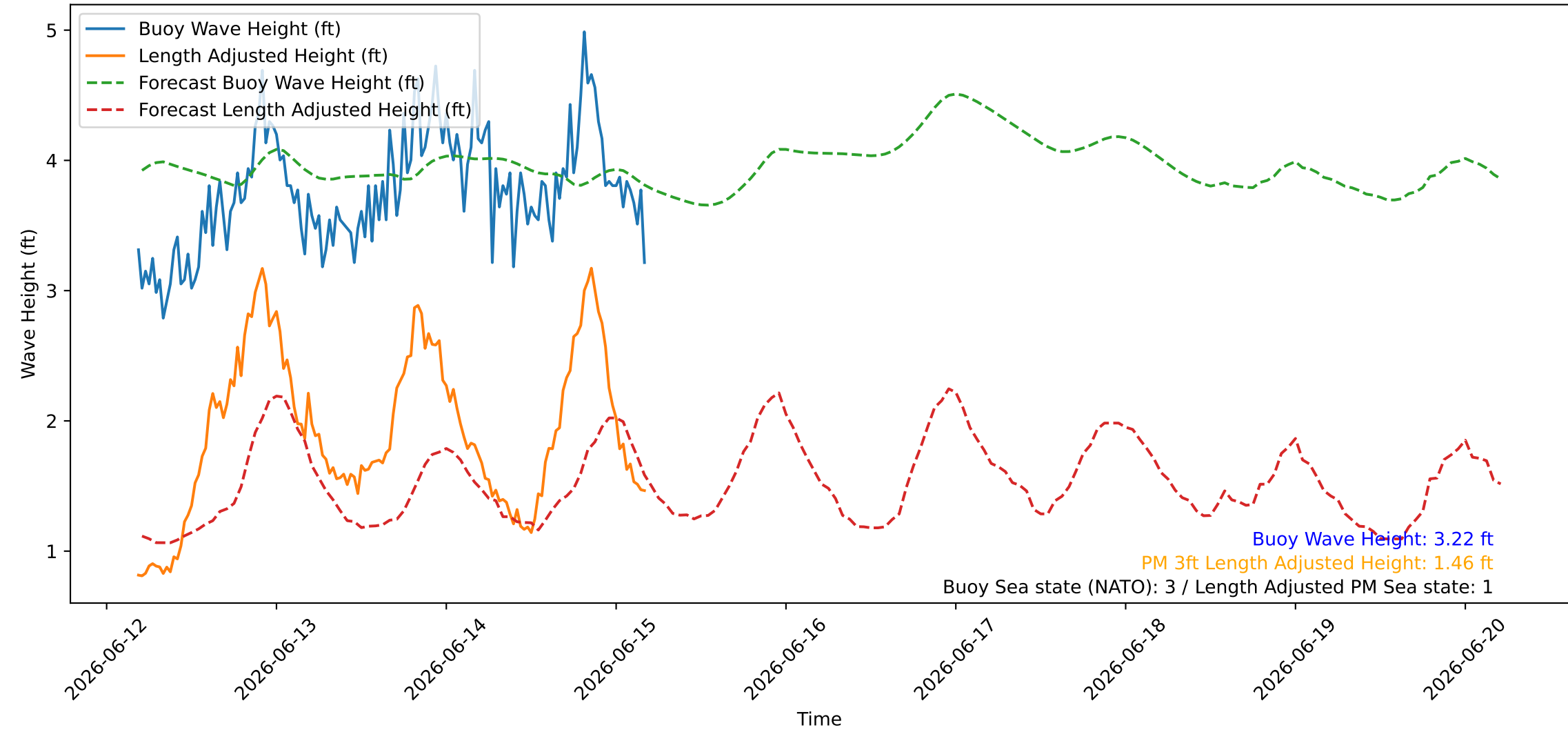
Wave Heights over Time for Oceanside Harbor at 2026-06-15 04:40:26
