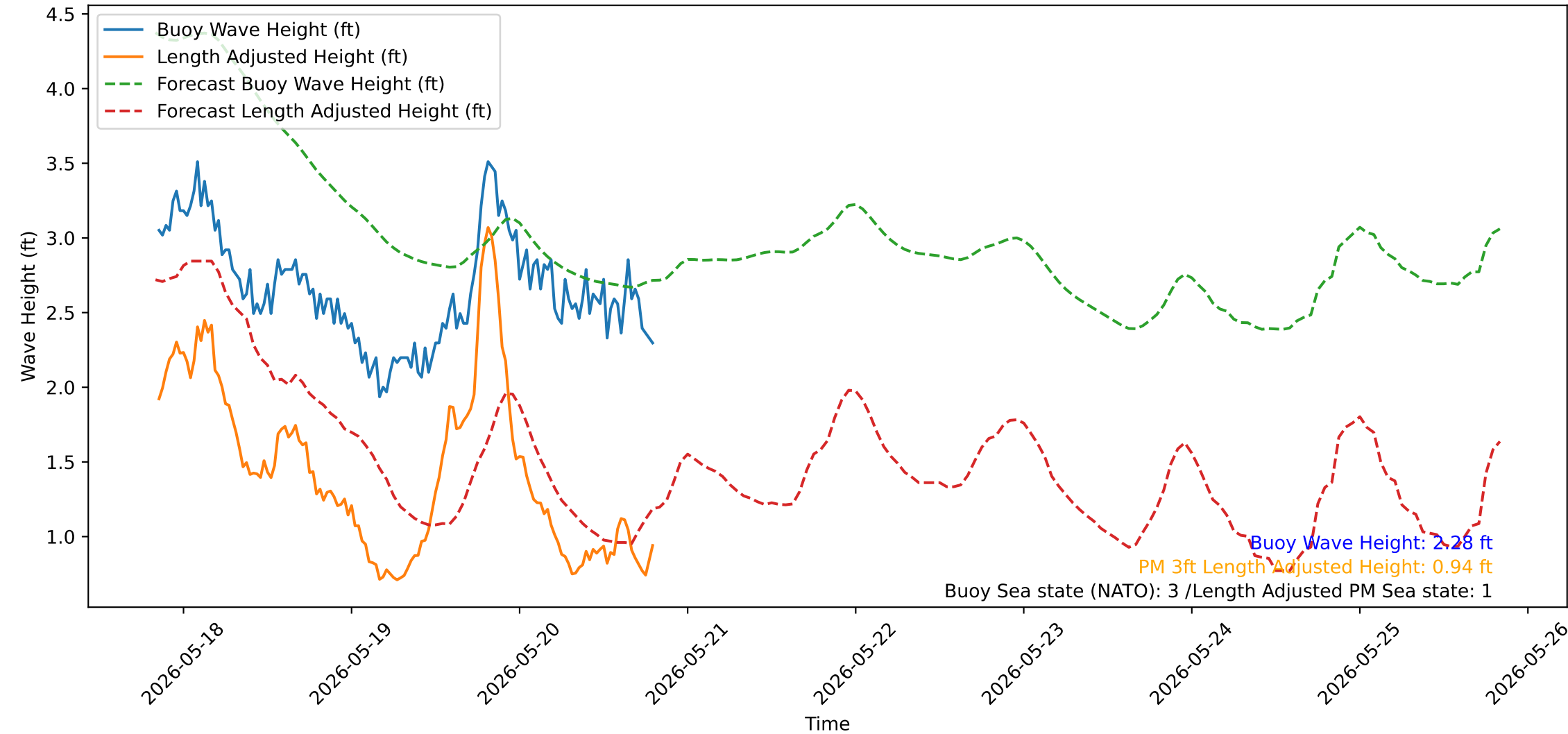
Wave Heights over Time for Red Beach at 2026-05-20 20:00:51
