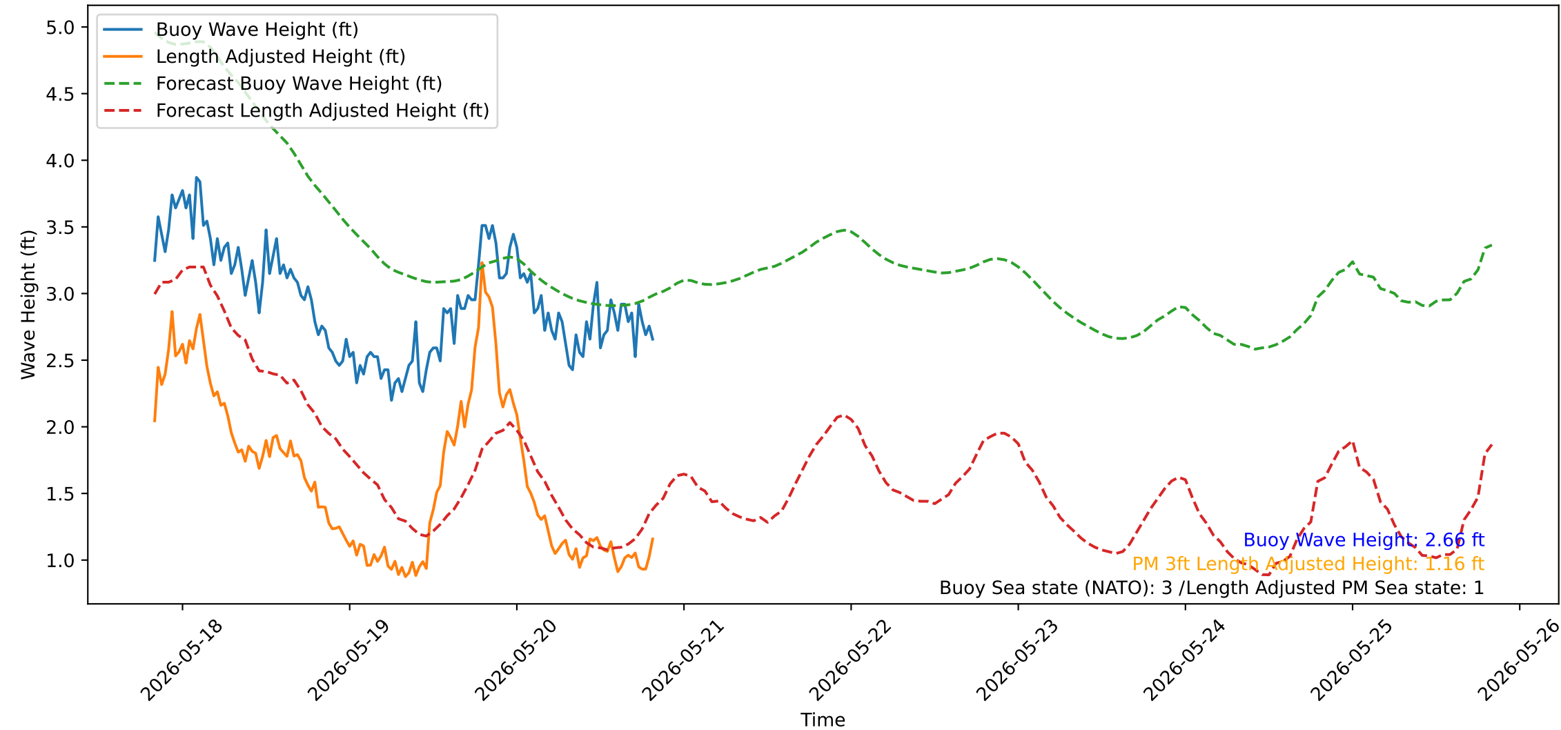
Wave Heights over Time for Oceanside Harbor at 2026-05-20 20:00:31
