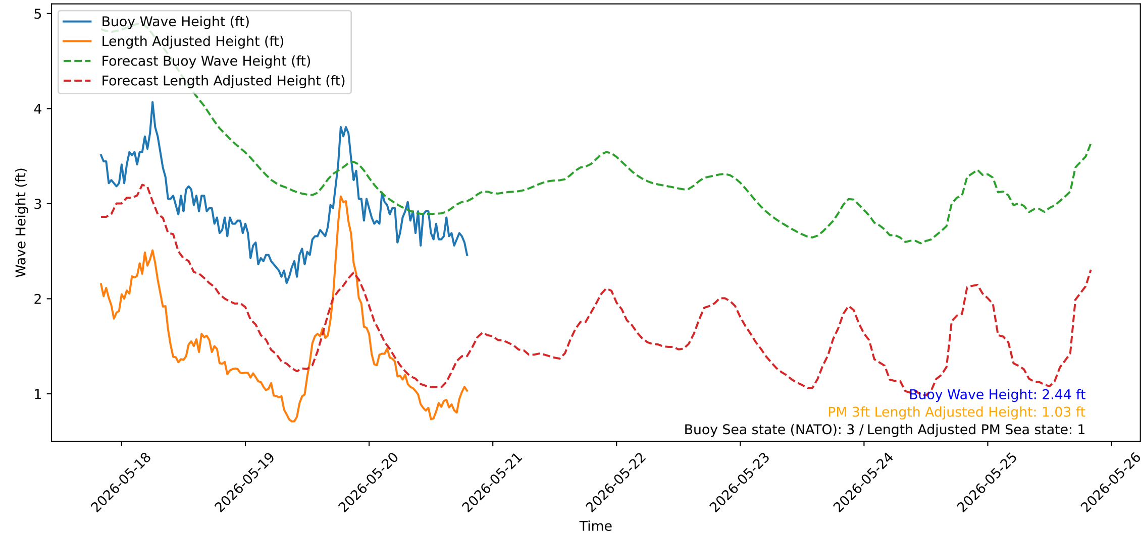
Wave Heights over Time for Green Beach at 2026-05-20 20:01:13
