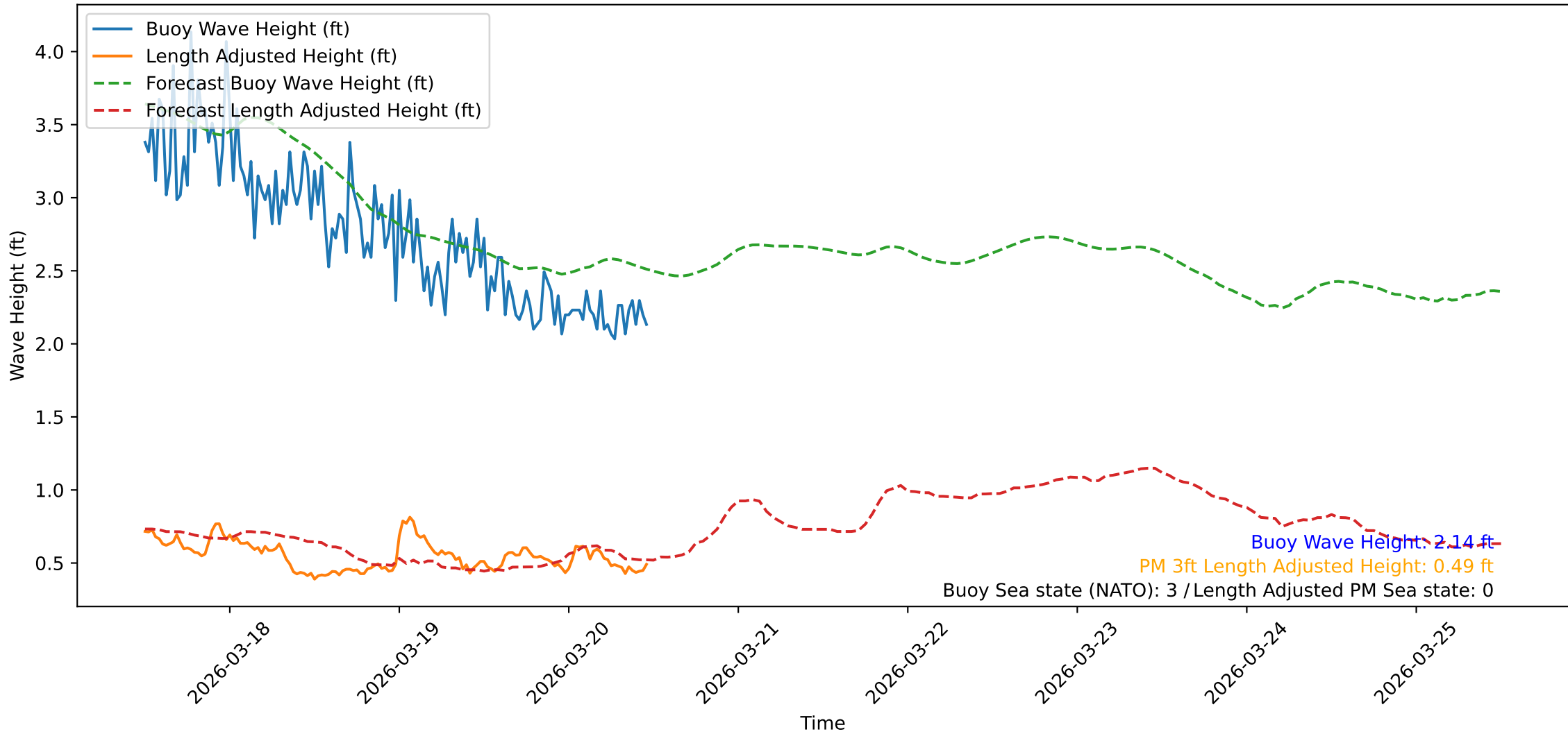
Wave Heights over Time for Green Beach at 2026-03-20 11:51:09
