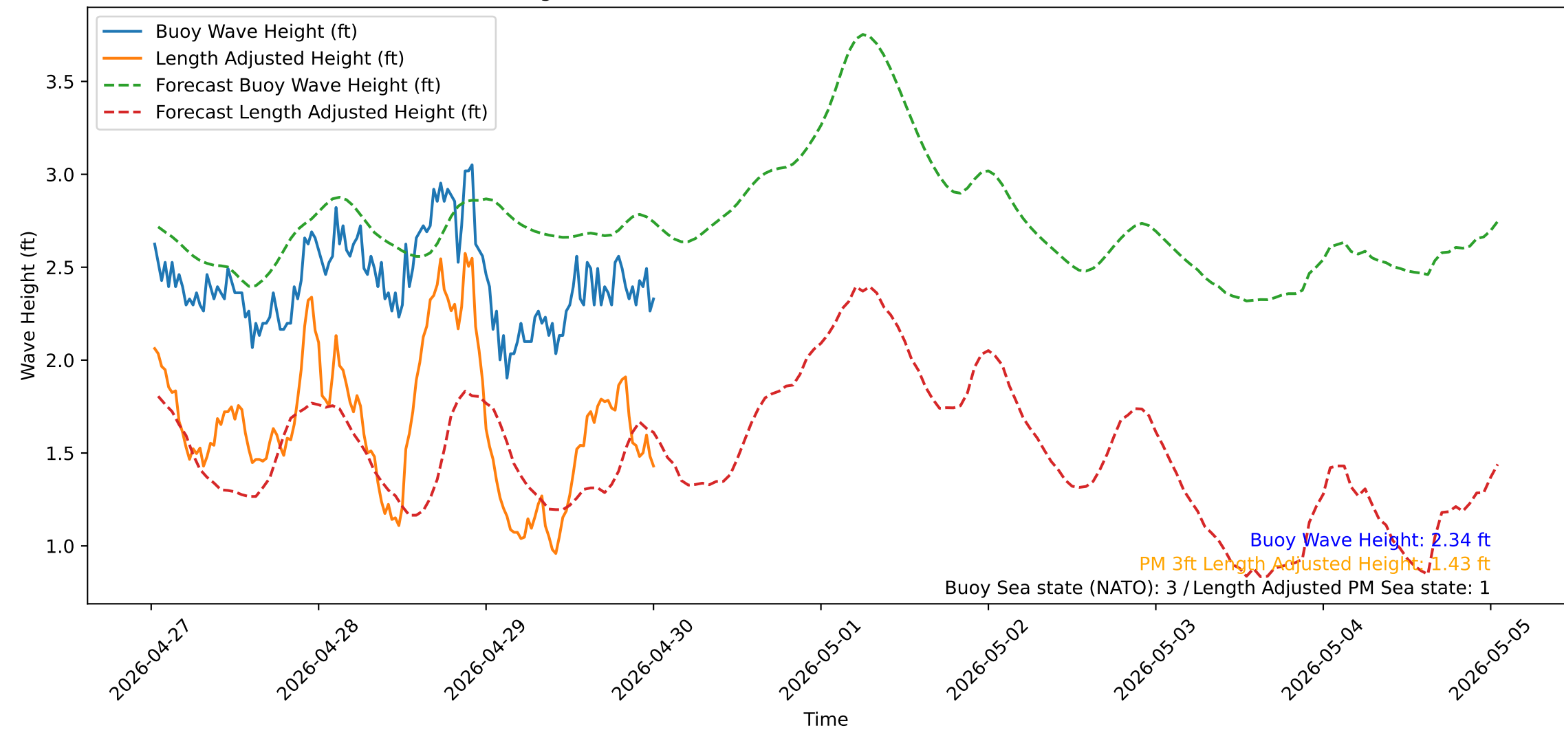
Wave Heights over Time for Oceanside Harbor at 2026-04-30 00:40:31
