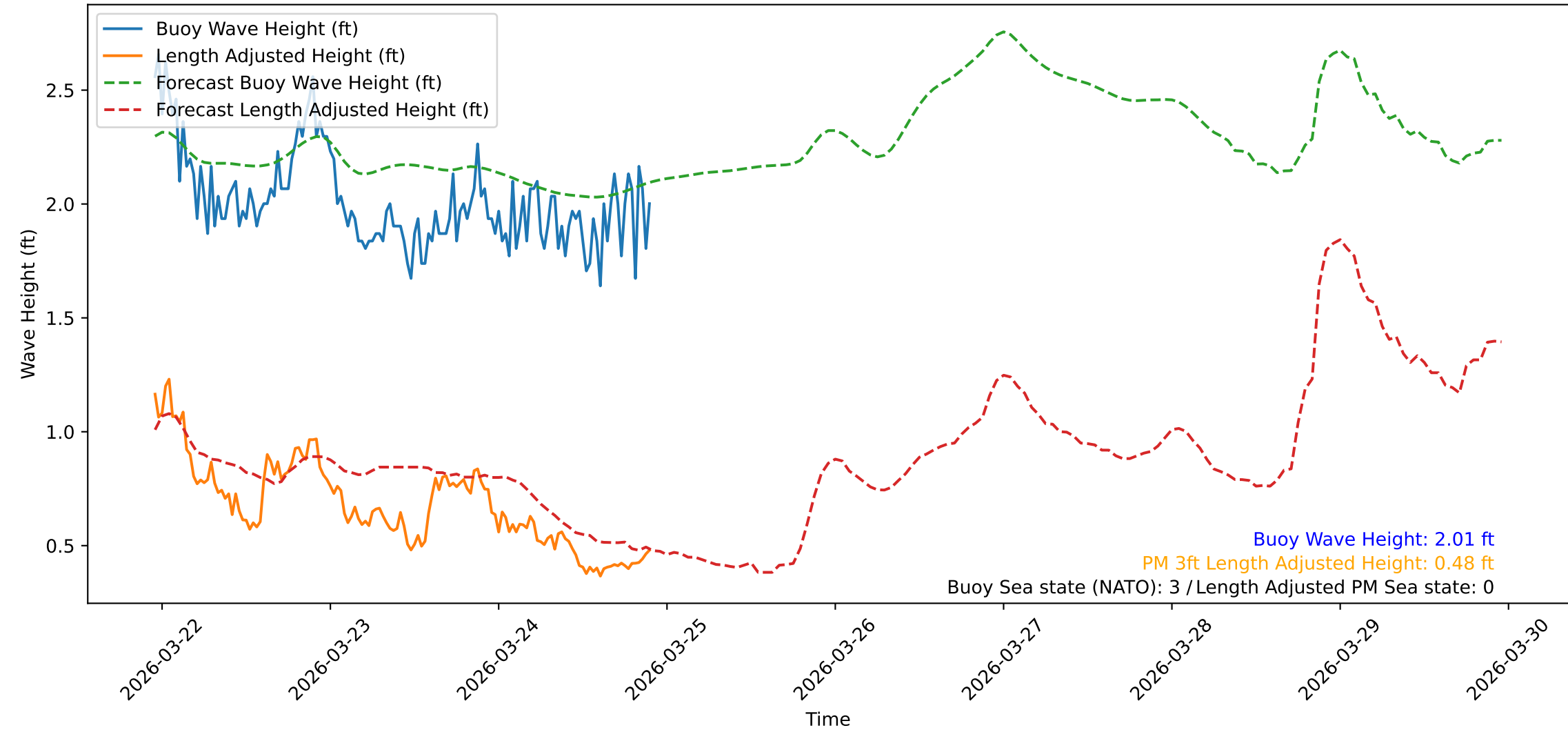
Wave Heights over Time for Red Beach at 2026-03-24 22:30:48
