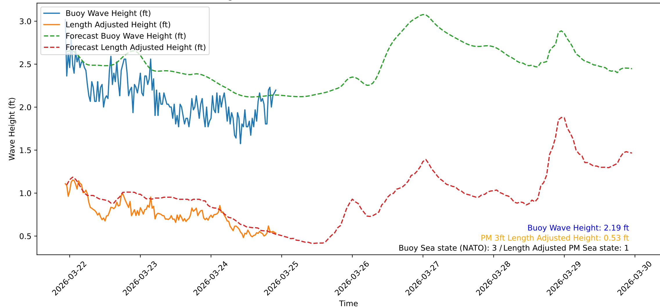
Wave Heights over Time for Oceanside Harbor at 2026-03-24 22:30:32
