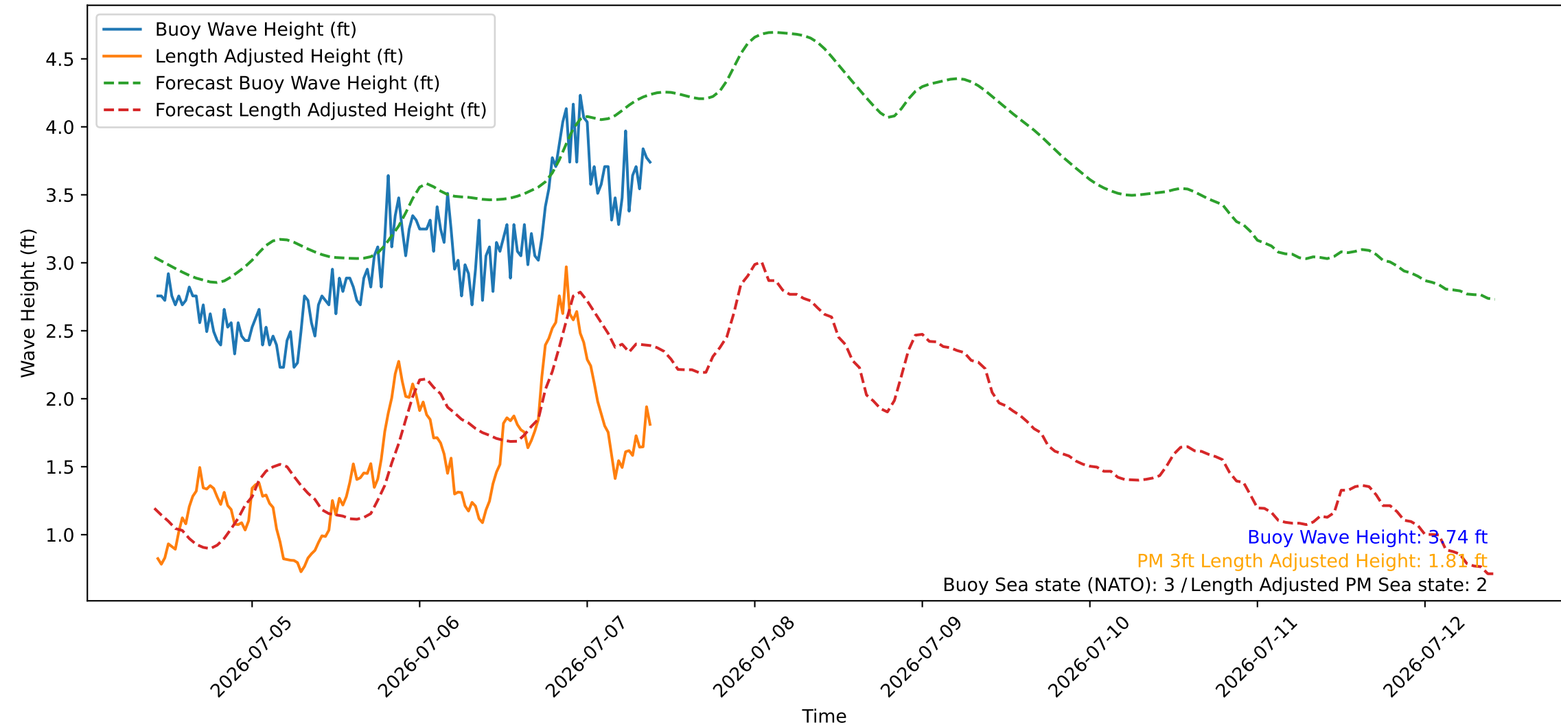
Wave Heights over Time for Red Beach at 2026-07-07 10:10:46
