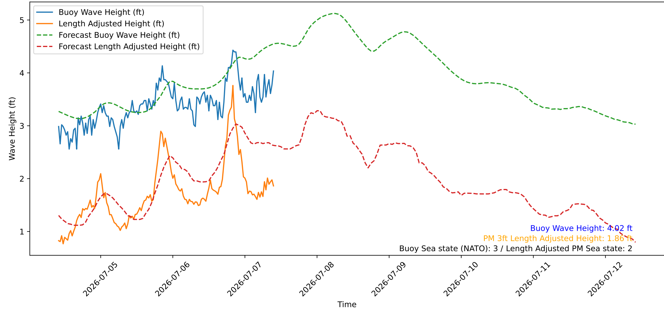
Wave Heights over Time for Green Beach at 2026-07-07 10:11:08
