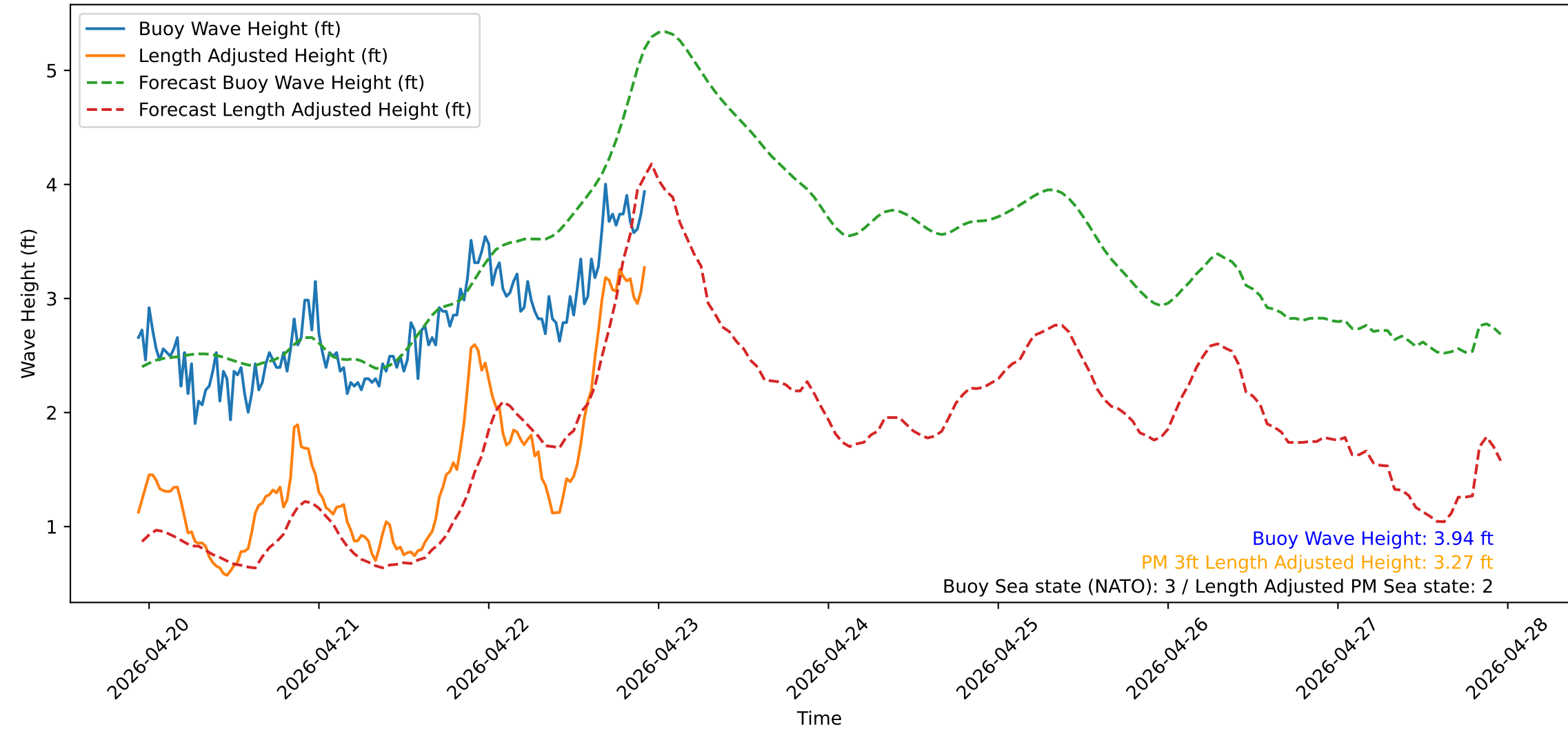
Wave Heights over Time for Green Beach at 2026-04-22 22:41:14
