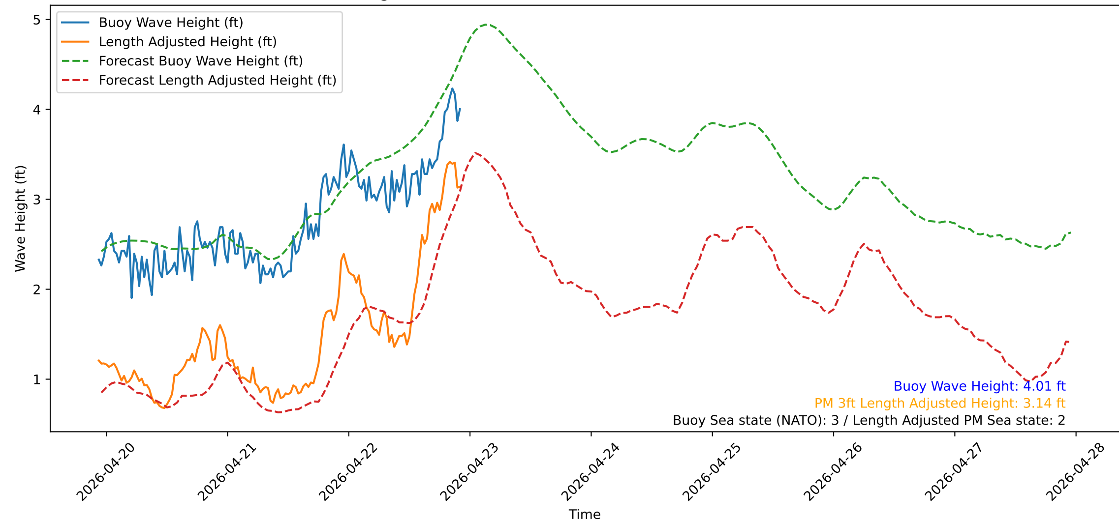
Wave Heights over Time for Oceanside Harbor at 2026-04-22 22:40:32
