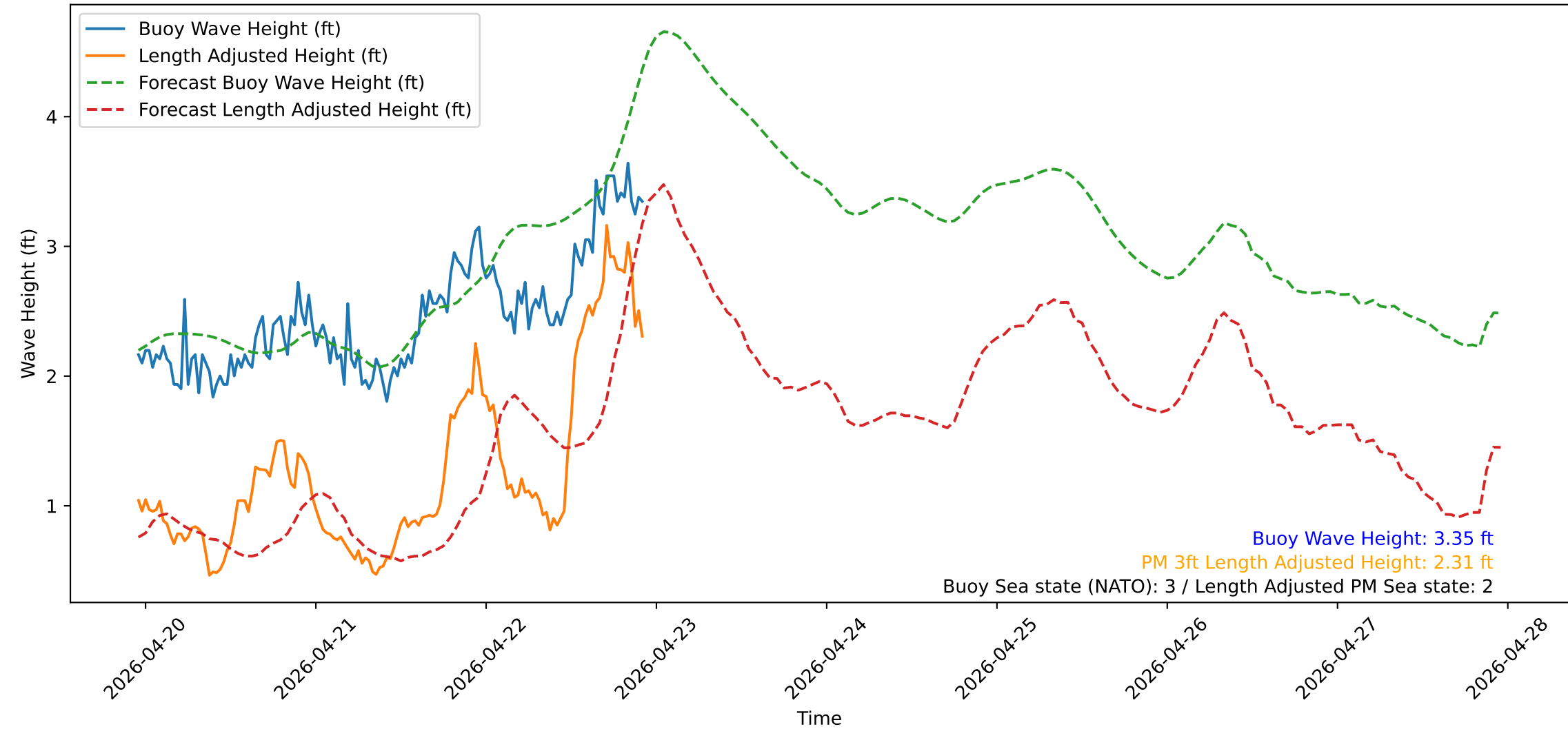
Wave Heights over Time for Red Beach at 2026-04-22 22:40:52
