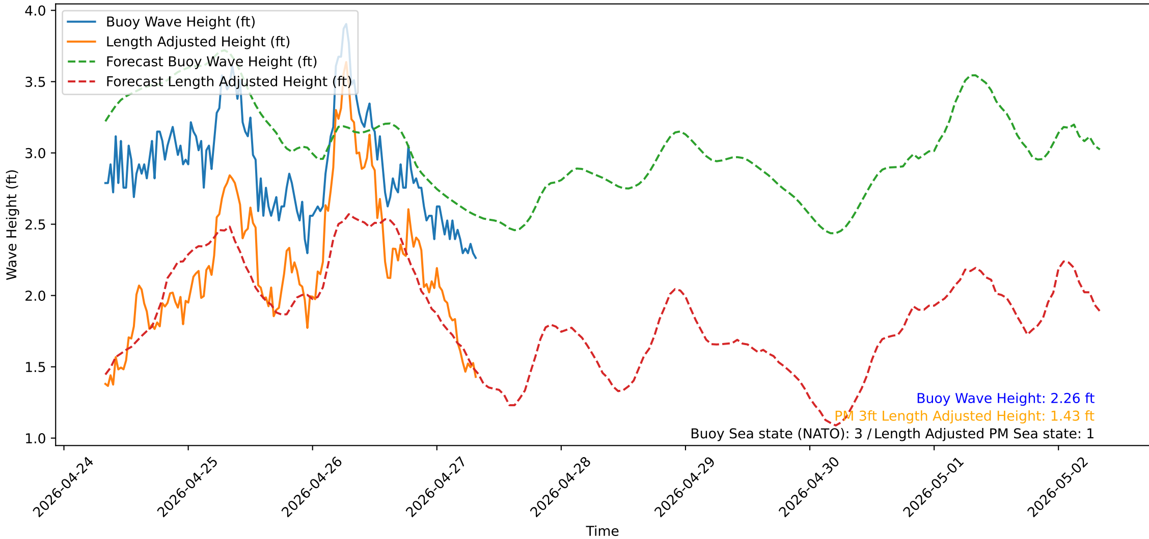
Wave Heights over Time for Oceanside Harbor at 2026-04-27 08:10:31
