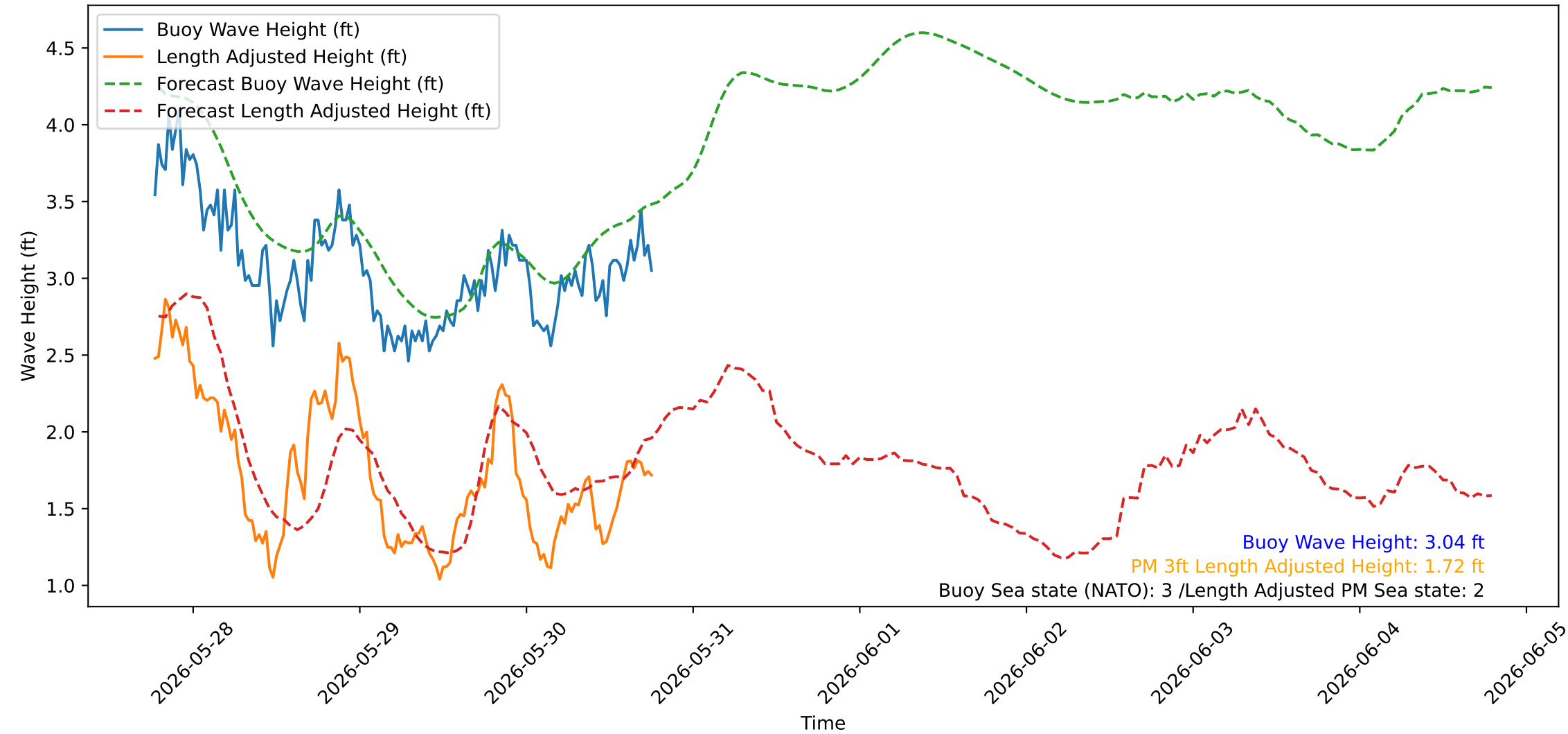
Wave Heights over Time for Green Beach at 2026-05-30 18:41:07
