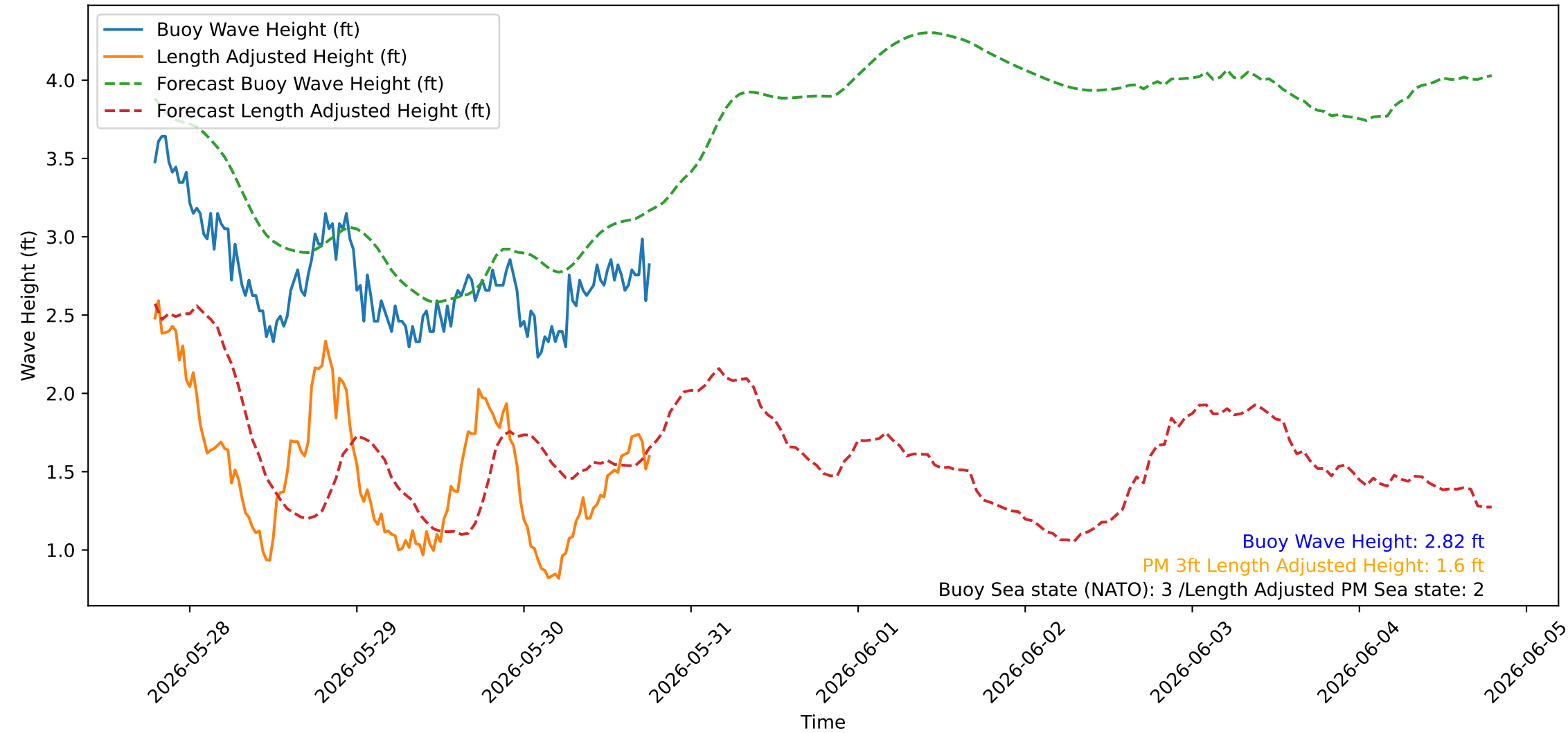
Wave Heights over Time for Red Beach at 2026-05-30 18:40:44
