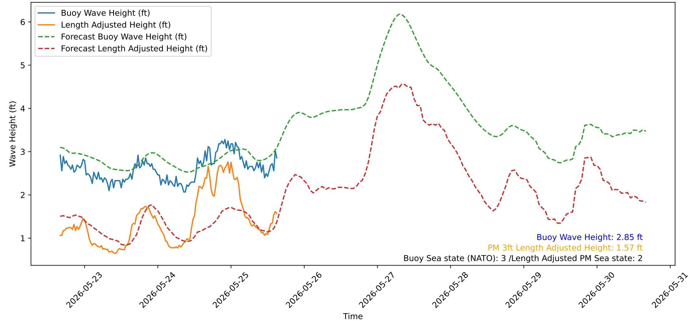
Wave Heights over Time for Green Beach at 2026-05-25 15:51:14
