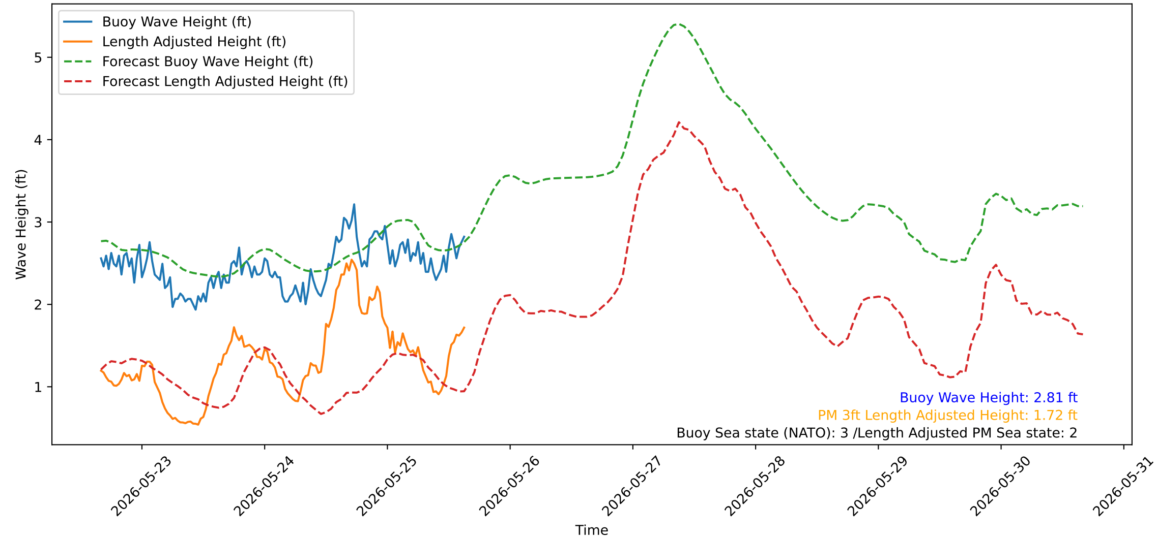
Wave Heights over Time for Red Beach at 2026-05-25 15:50:51
