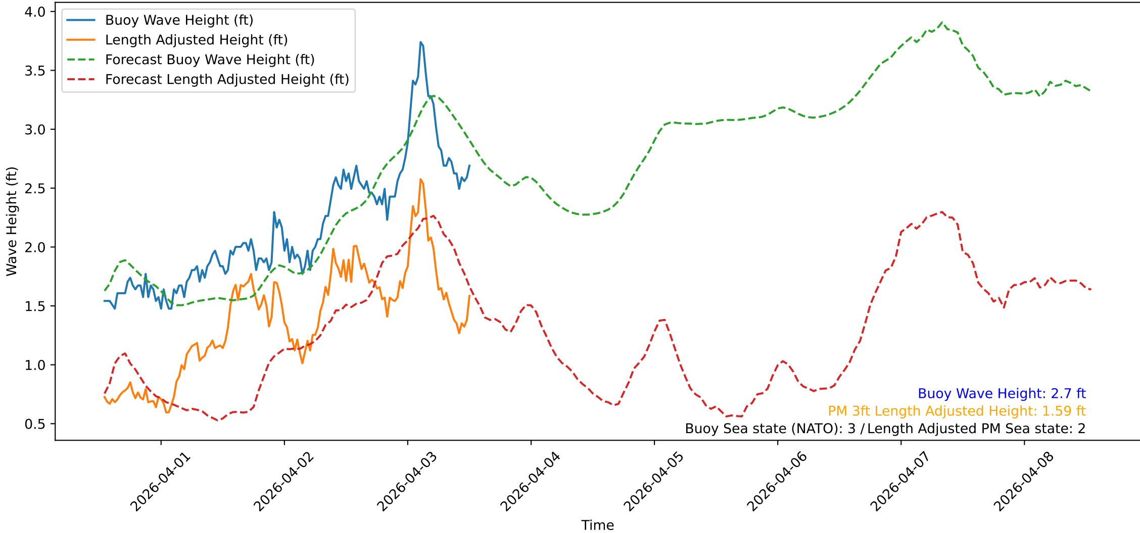
Wave Heights over Time for Red Beach at 2026-04-03 12:40:50
