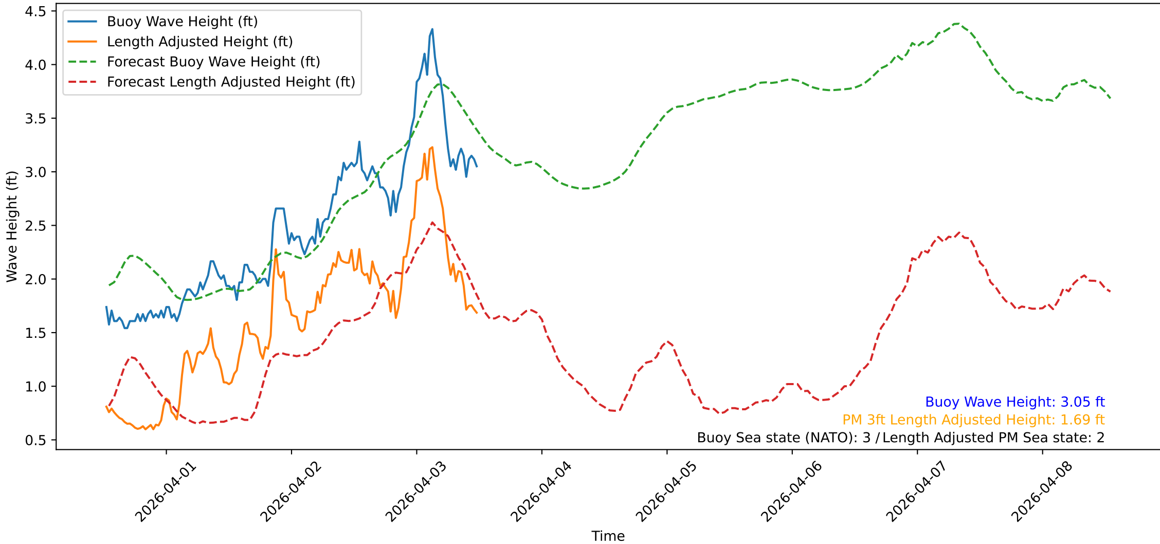
Wave Heights over Time for Green Beach at 2026-04-03 12:41:12
