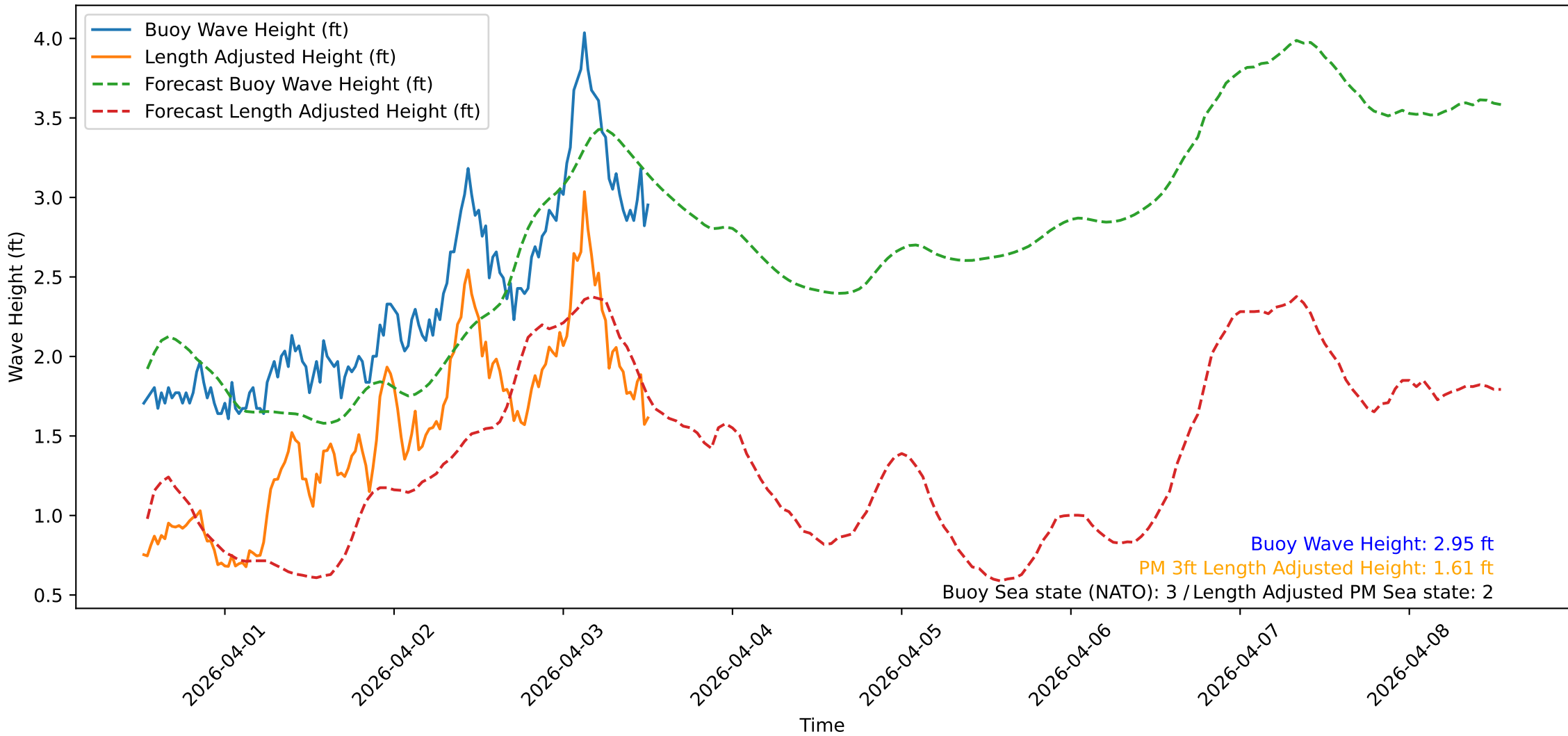
Wave Heights over Time for Oceanside Harbor at 2026-04-03 12:40:32
