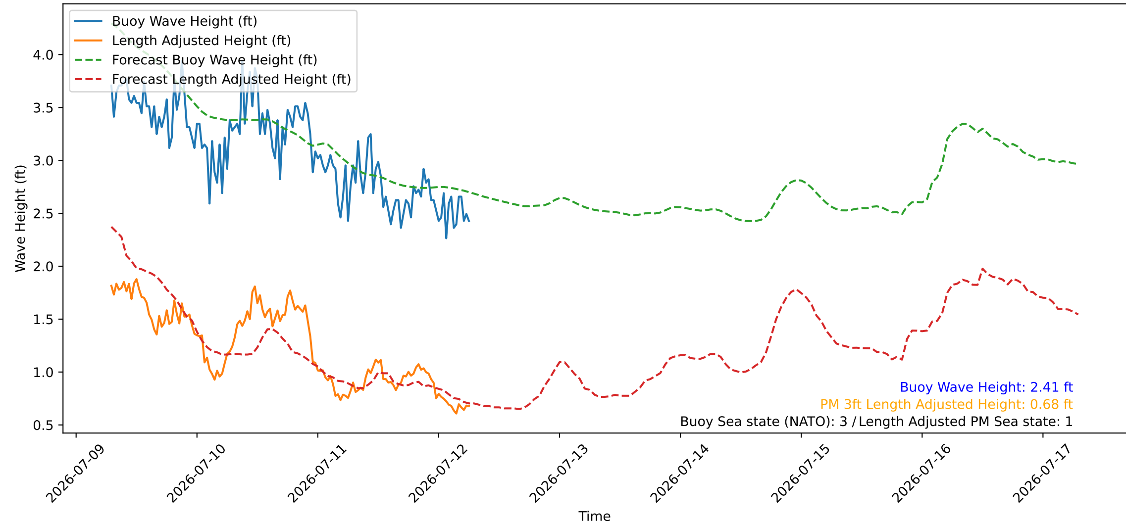
Wave Heights over Time for Red Beach at 2026-07-12 06:50:48
