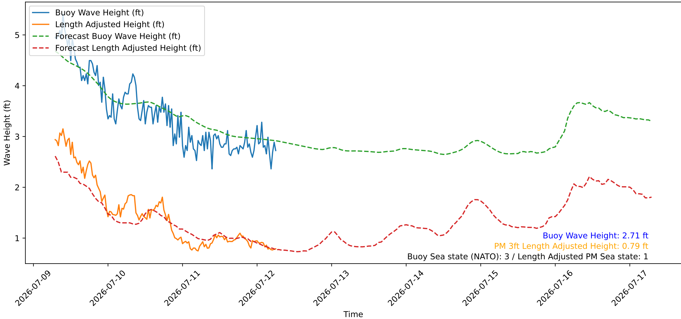
Wave Heights over Time for Oceanside Harbor at 2026-07-12 06:50:27
