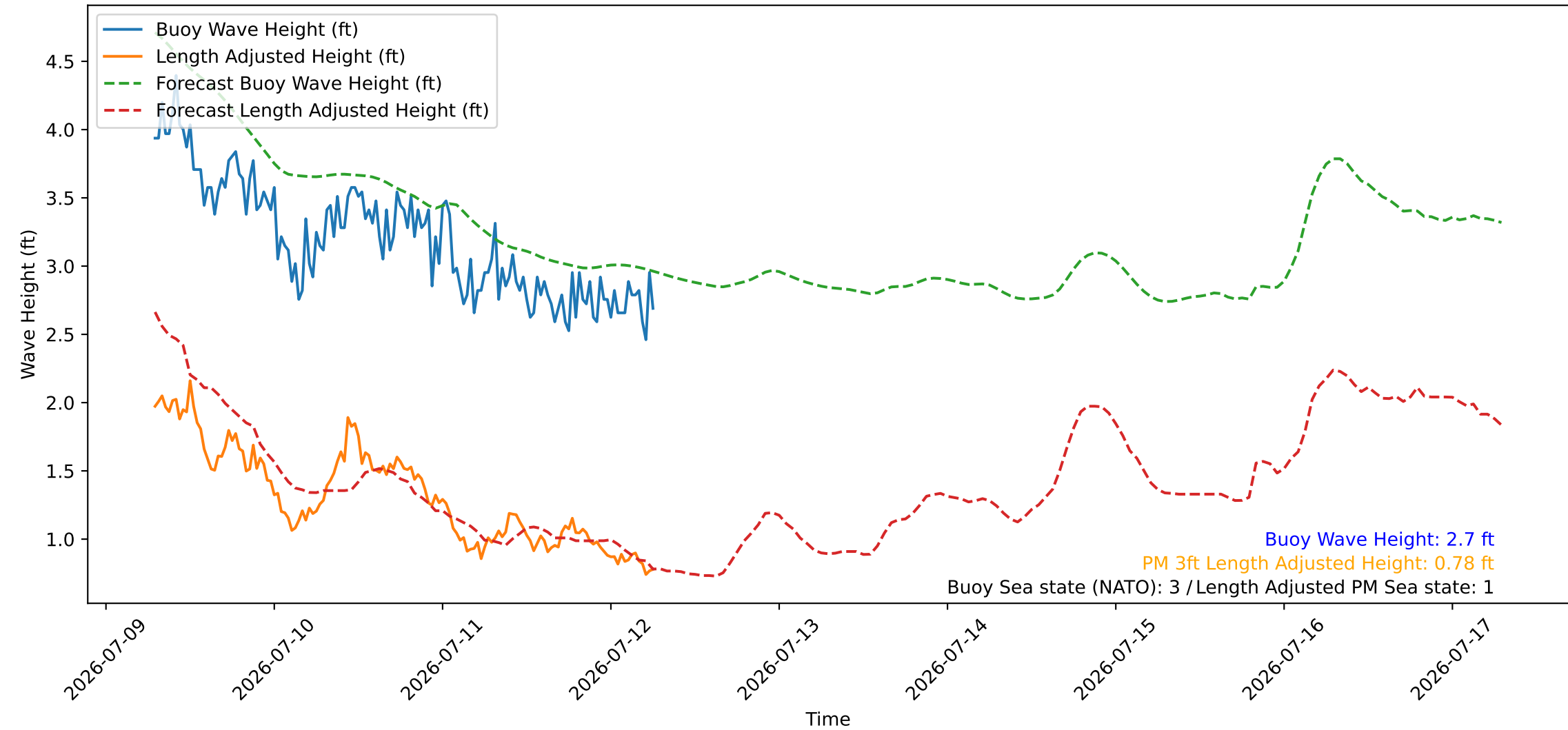
Wave Heights over Time for Green Beach at 2026-07-12 06:51:10
