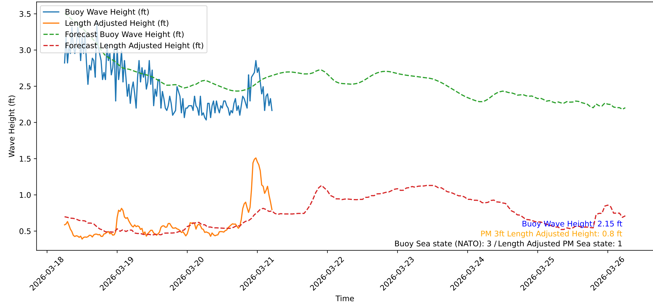
Wave Heights over Time for Green Beach at 2026-03-21 06:01:09
