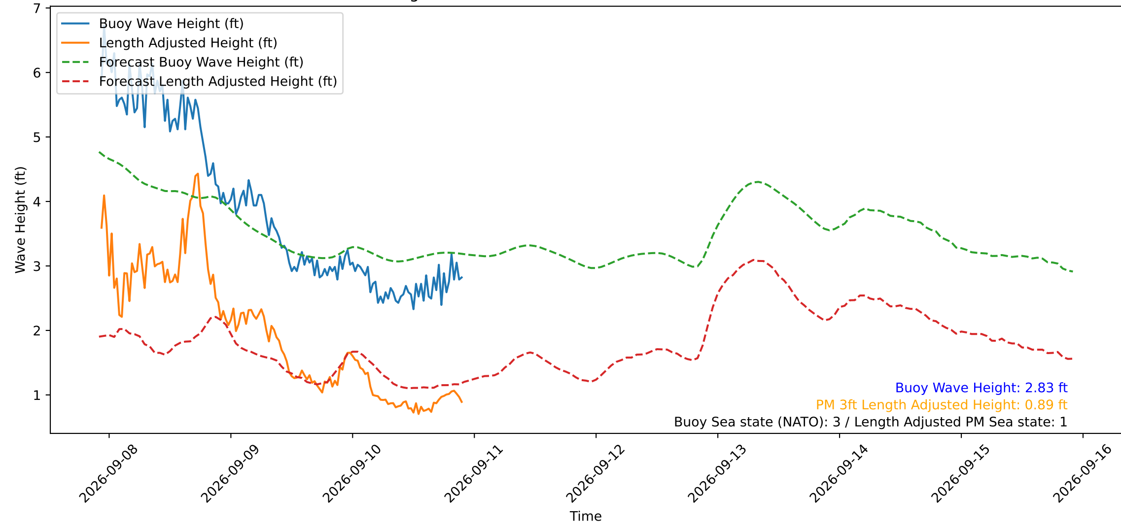
Wave Heights over Time for Red Beach at 2026-09-10 22:20:50
