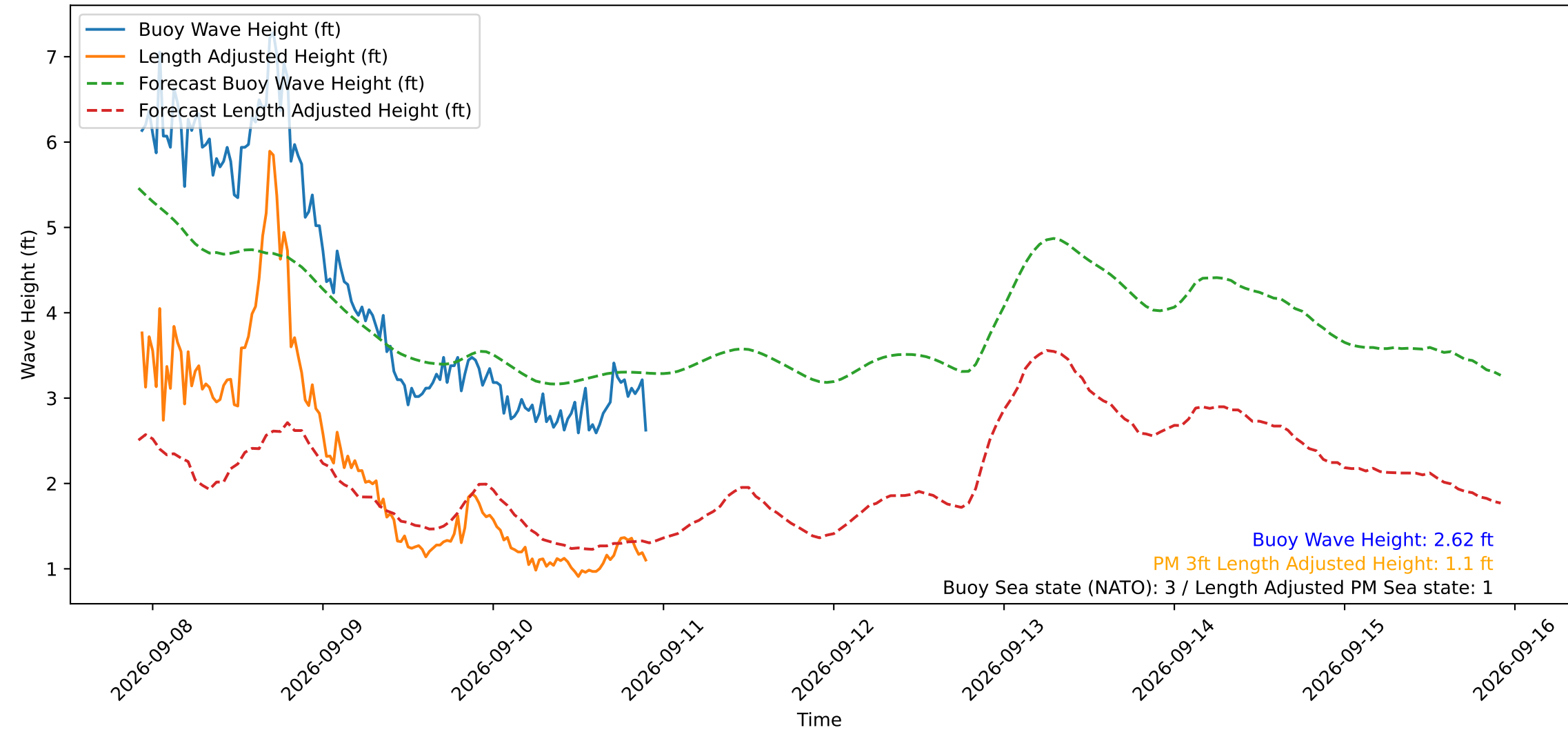
Wave Heights over Time for Green Beach at 2026-09-10 22:21:14
