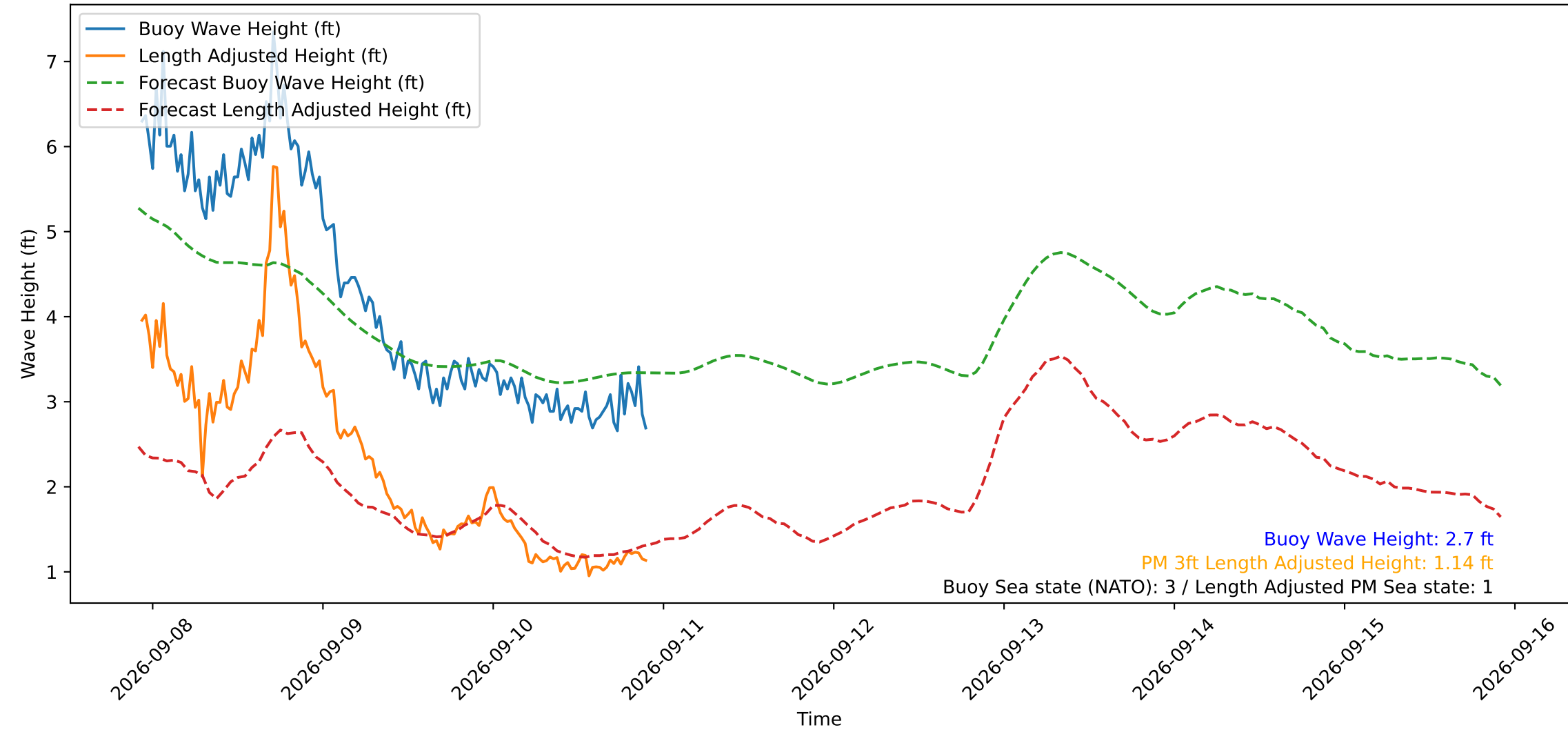
Wave Heights over Time for Oceanside Harbor at 2026-09-10 22:20:30
