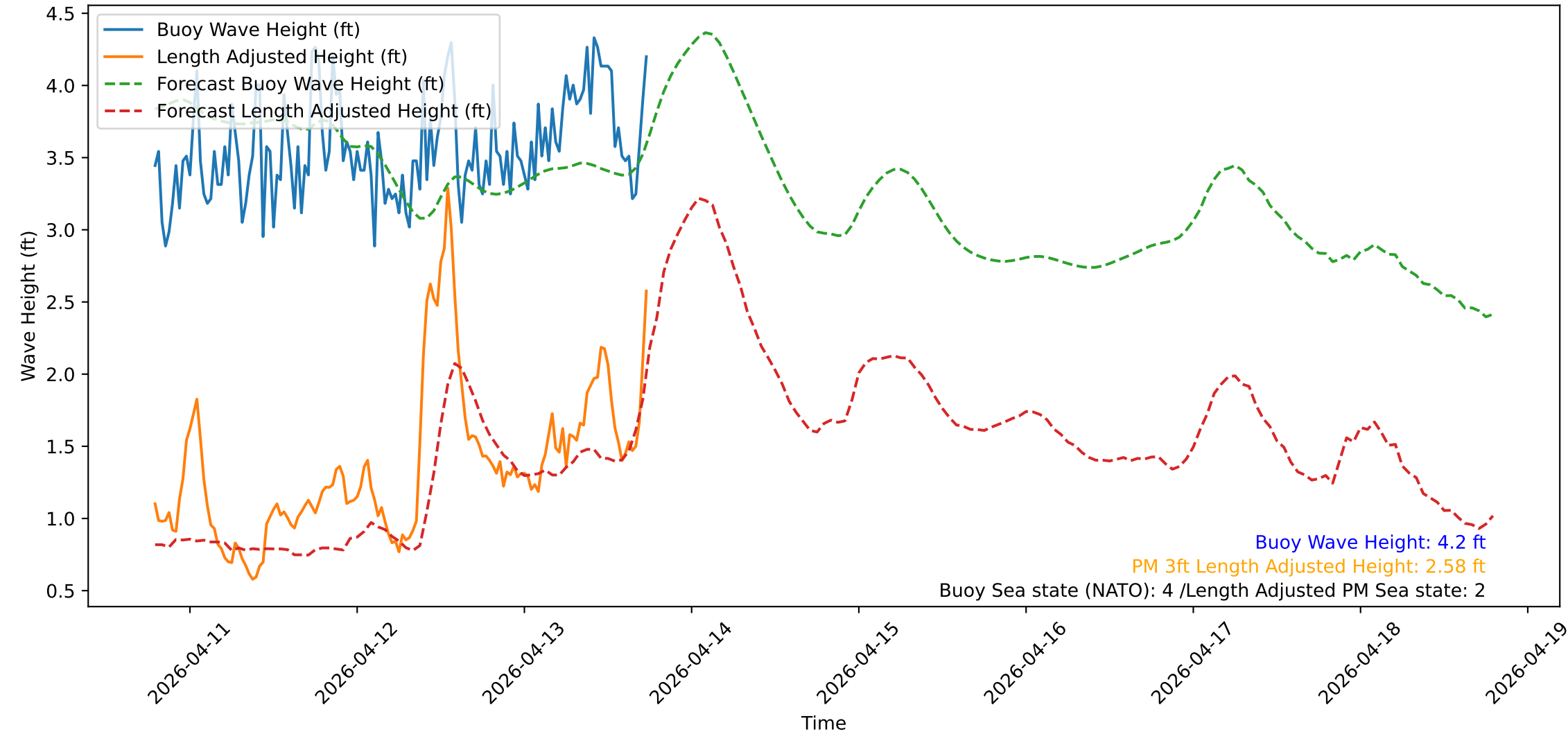
Wave Heights over Time for Red Beach at 2026-04-13 18:30:50
