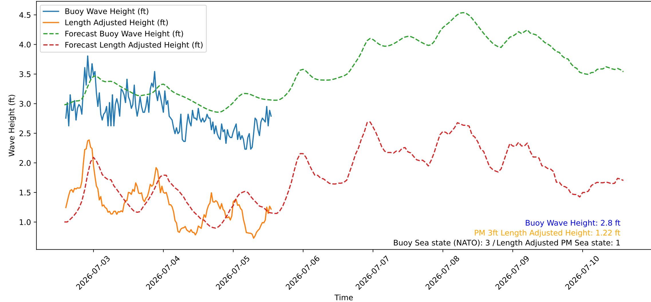
Wave Heights over Time for Red Beach at 2026-07-05 14:00:47
