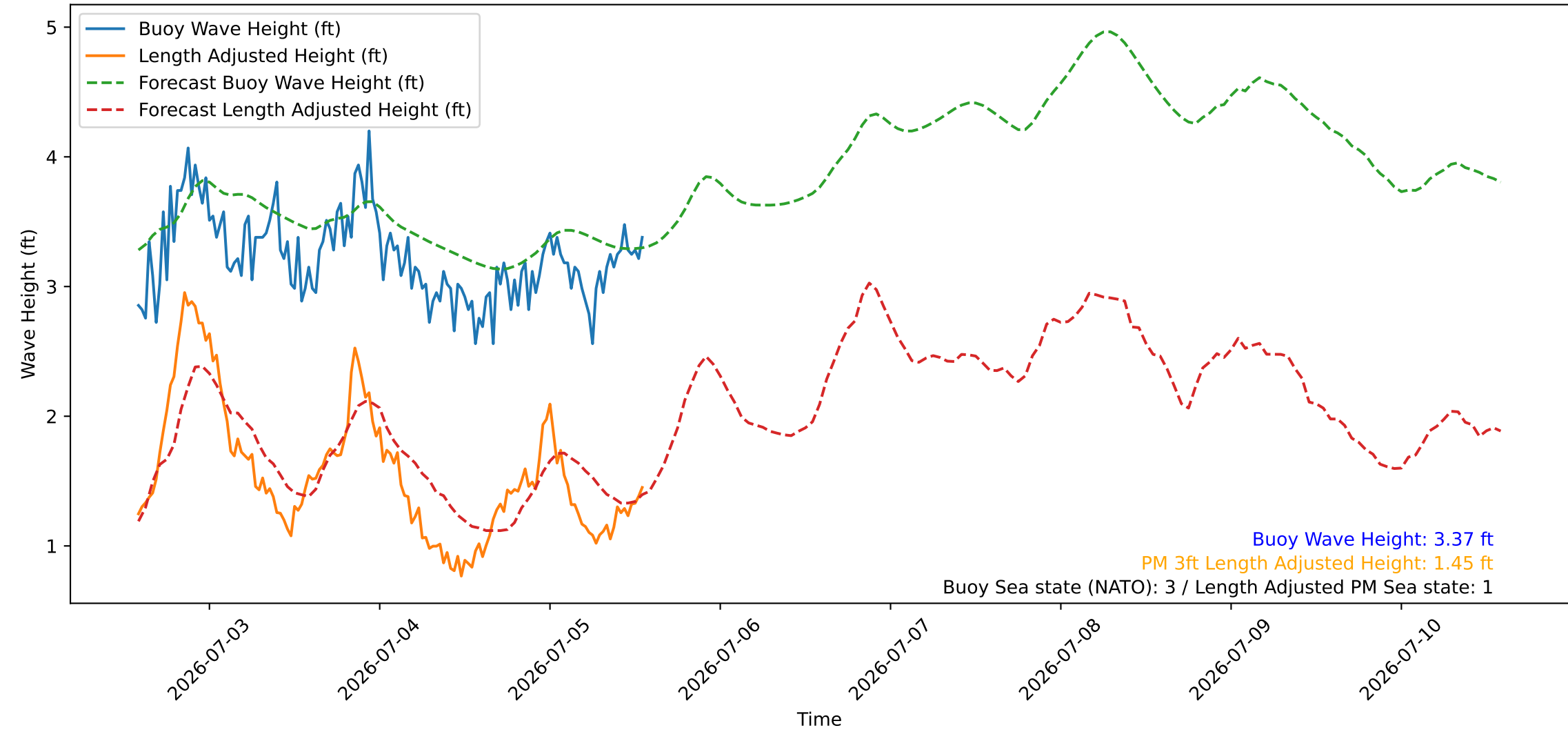
Wave Heights over Time for Green Beach at 2026-07-05 14:01:09
