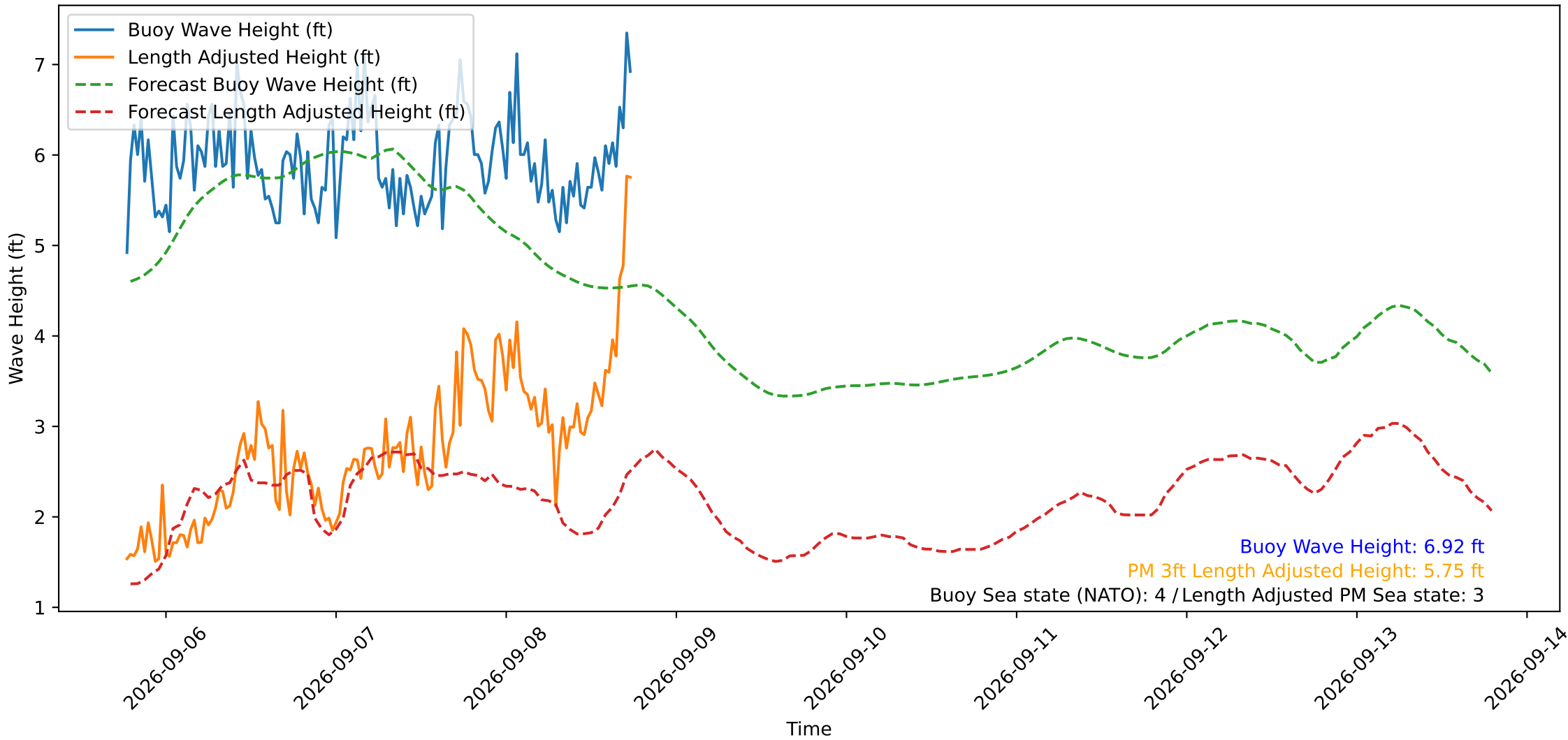
Wave Heights over Time for Oceanside Harbor at 2026-09-08 18:40:29
