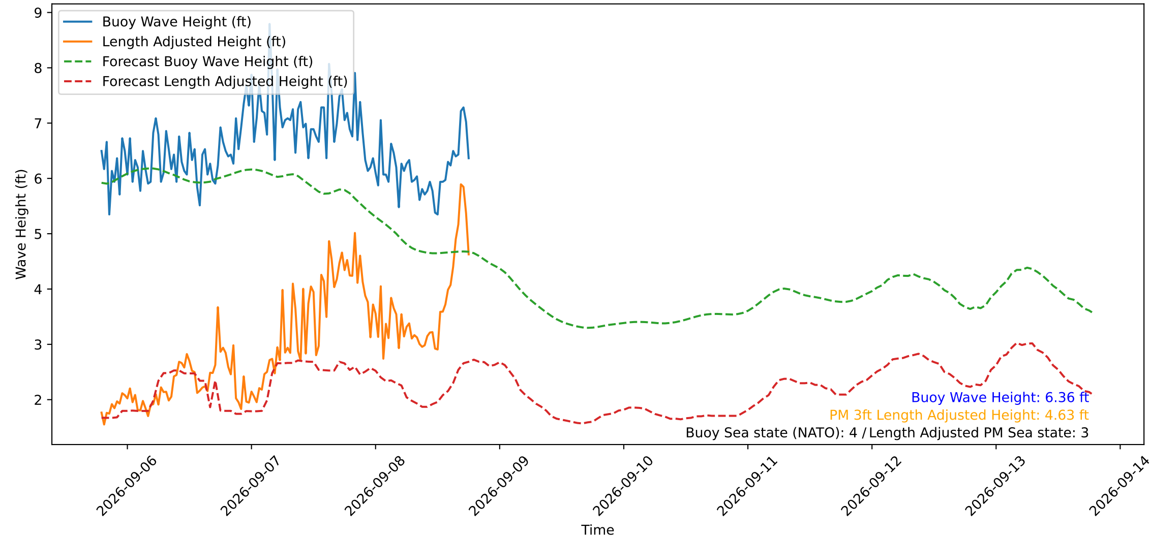
Wave Heights over Time for Green Beach at 2026-09-08 18:41:11
