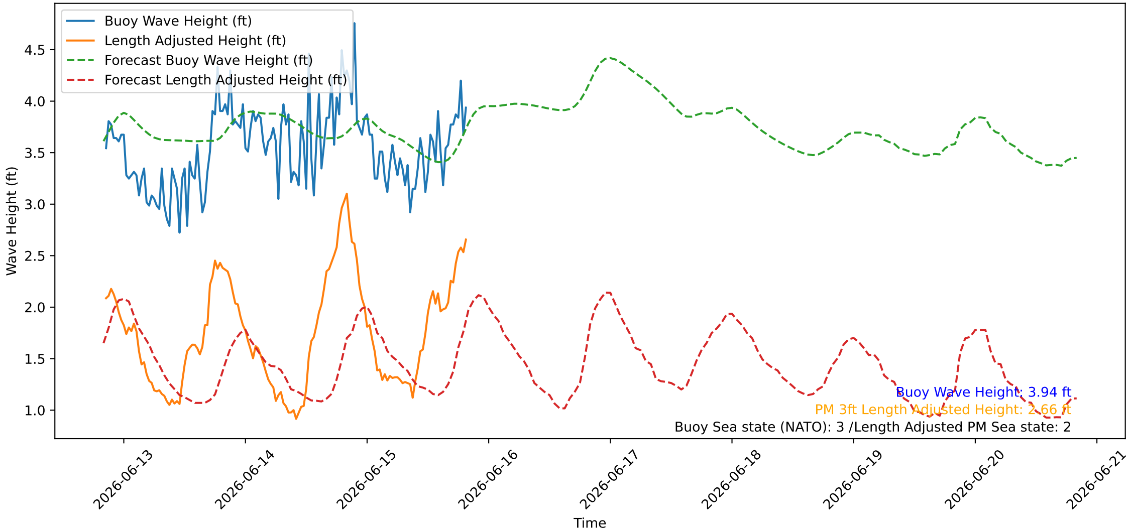
Wave Heights over Time for Red Beach at 2026-06-15 20:20:47
