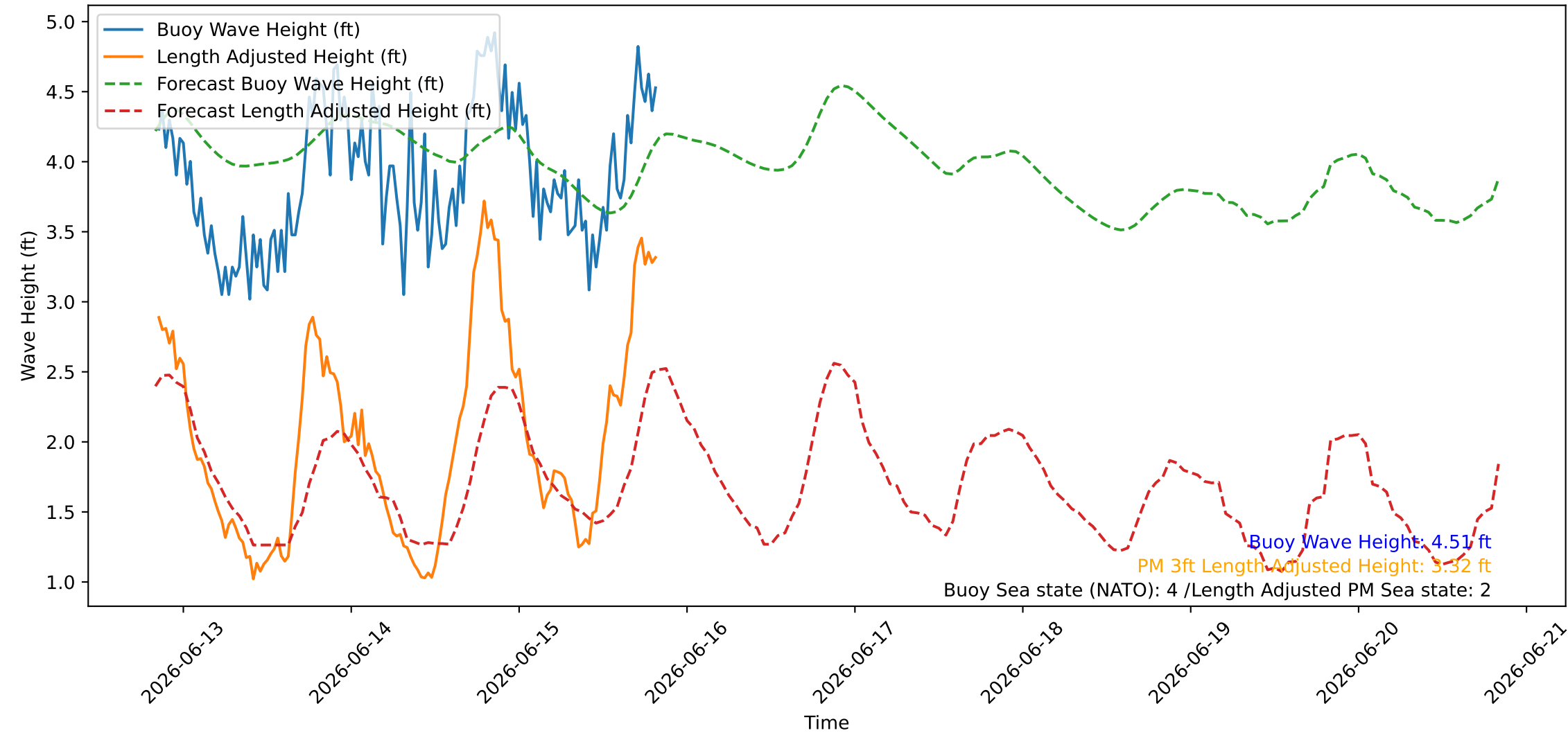
Wave Heights over Time for Green Beach at 2026-06-15 20:21:09
