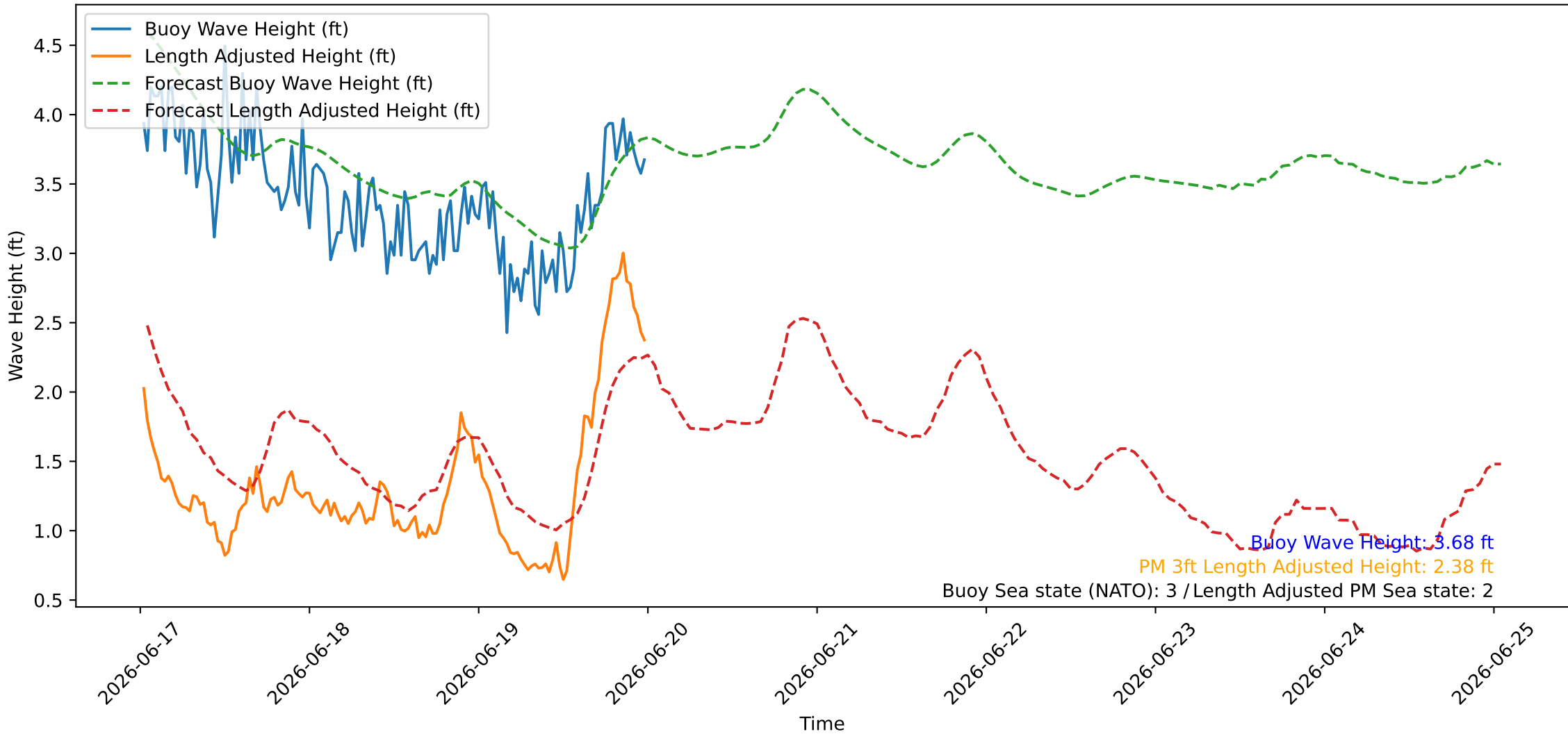
Wave Heights over Time for Green Beach at 2026-06-20 00:31:07
