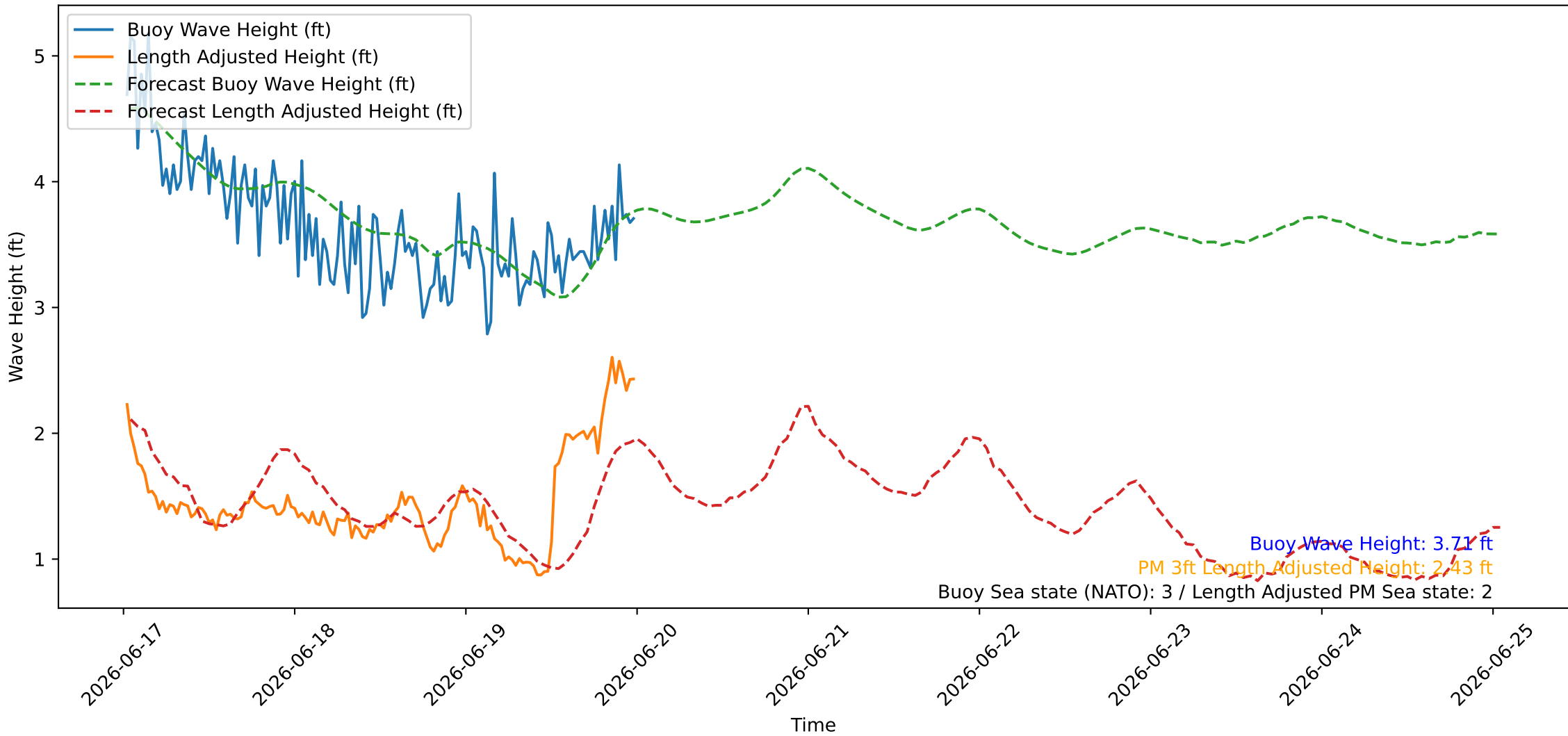
Wave Heights over Time for Oceanside Harbor at 2026-06-20 00:30:26
