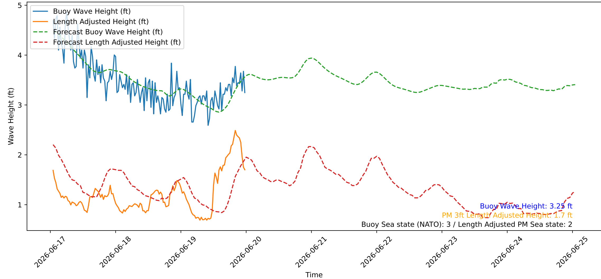
Wave Heights over Time for Red Beach at 2026-06-20 00:30:45
