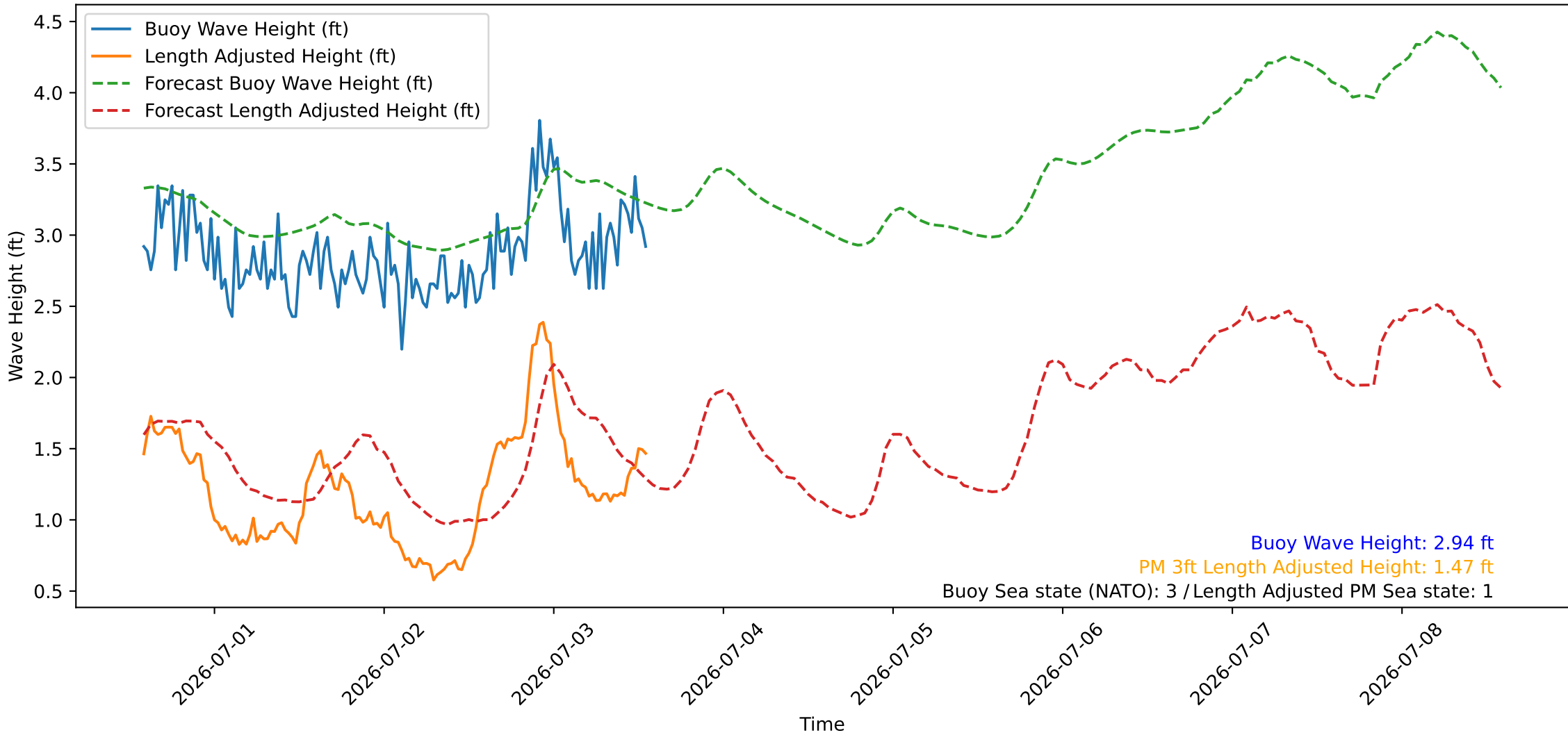
Wave Heights over Time for Red Beach at 2026-07-03 13:50:48
