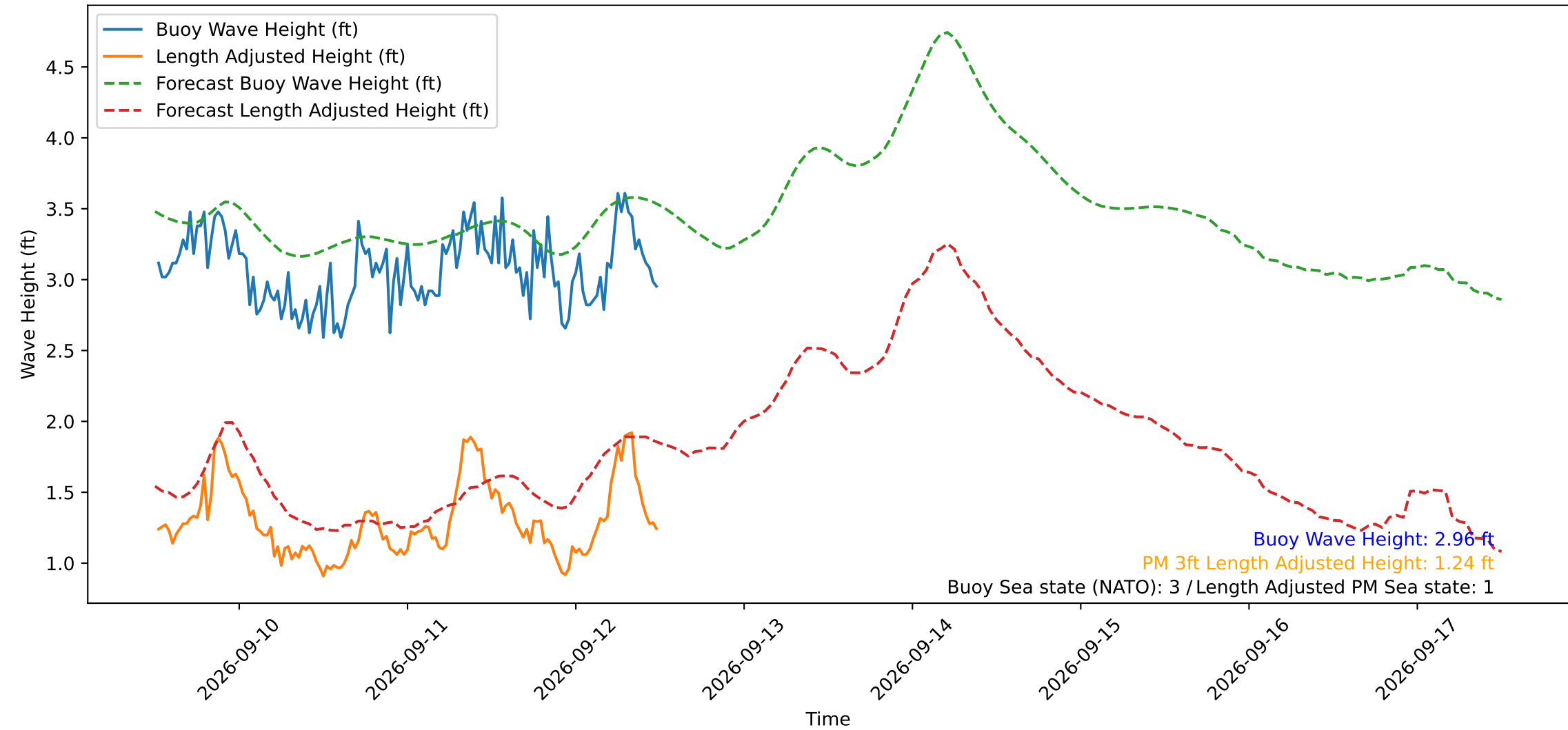
Wave Heights over Time for Green Beach at 2026-09-12 12:21:15
