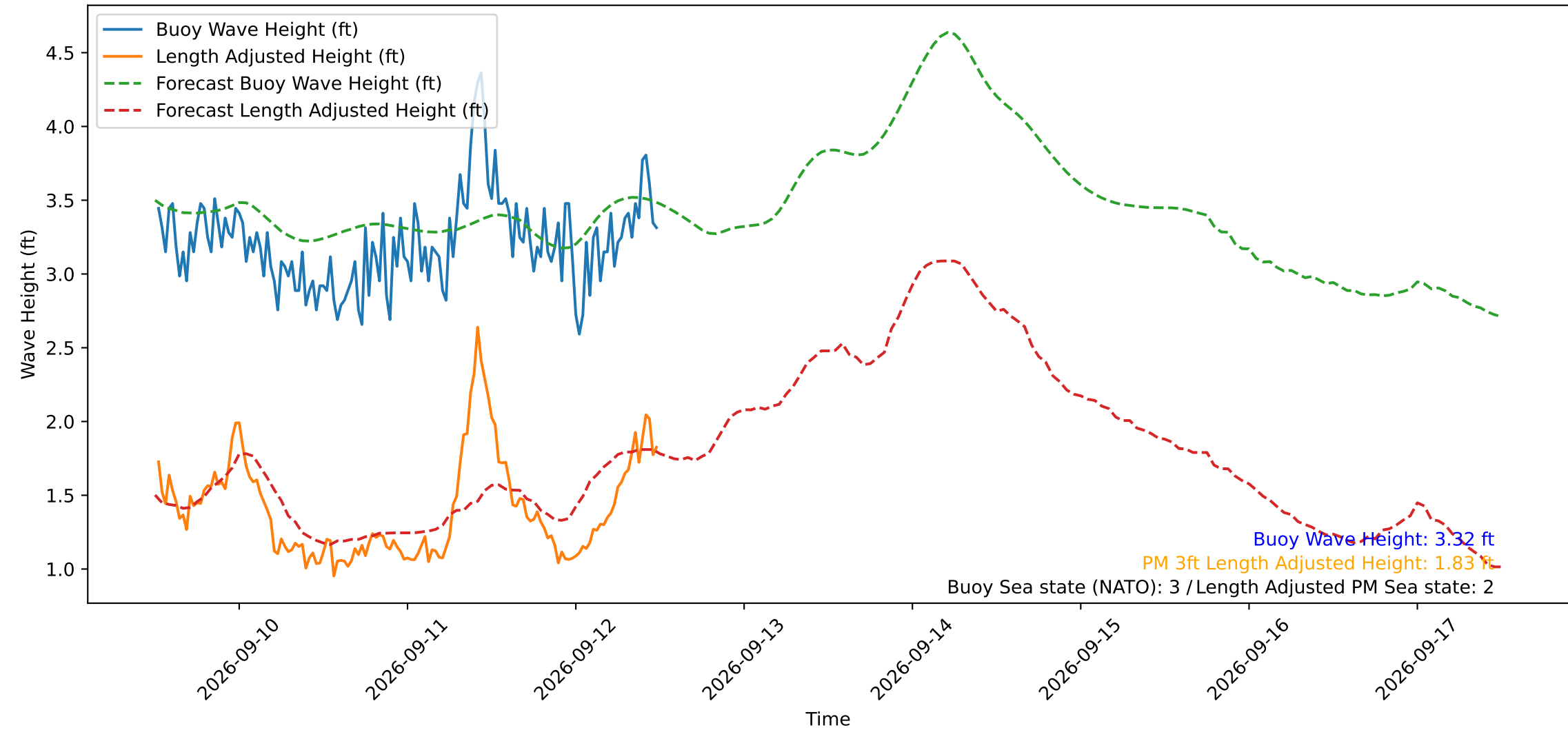
Wave Heights over Time for Oceanside Harbor at 2026-09-12 12:20:29
