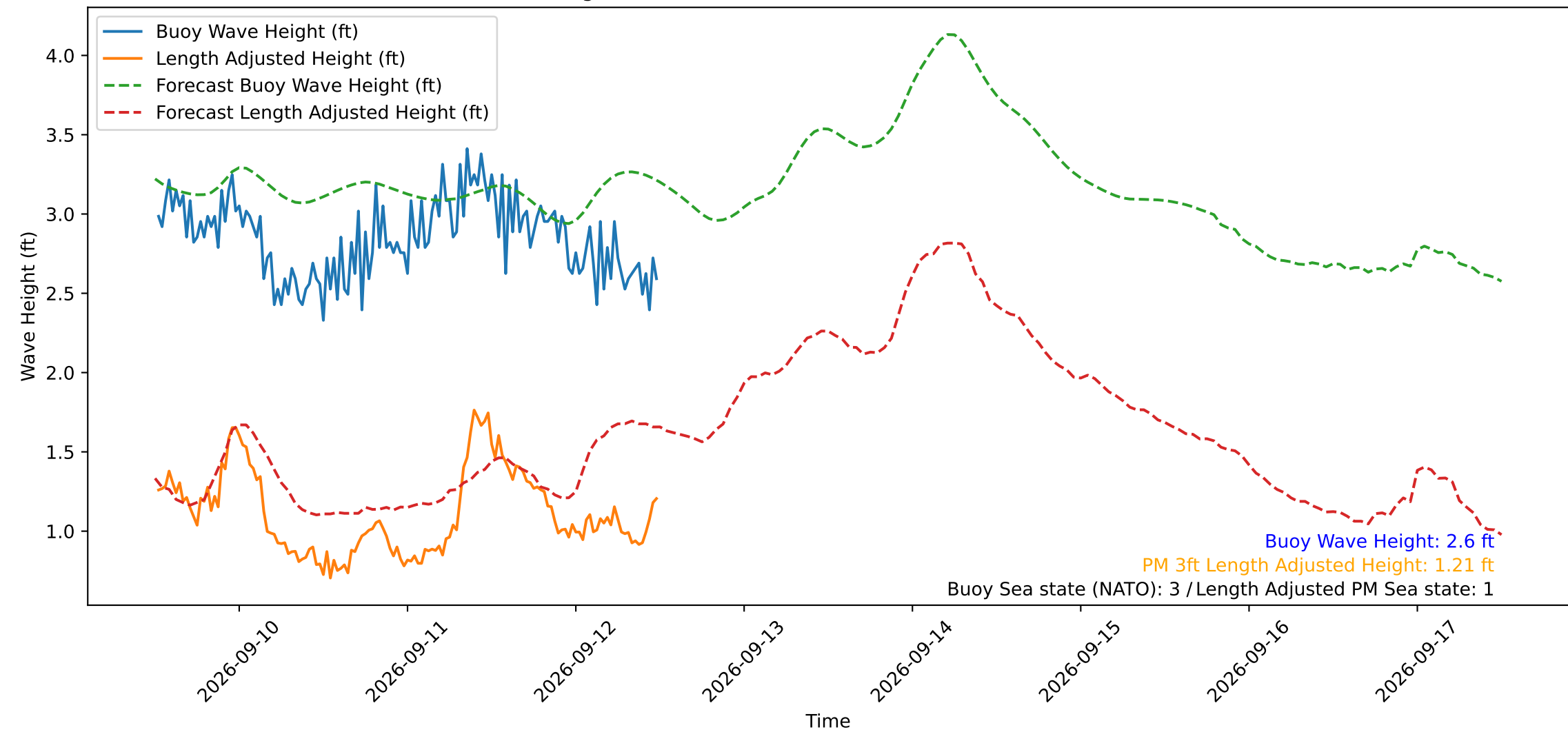
Wave Heights over Time for Red Beach at 2026-09-12 12:20:50
